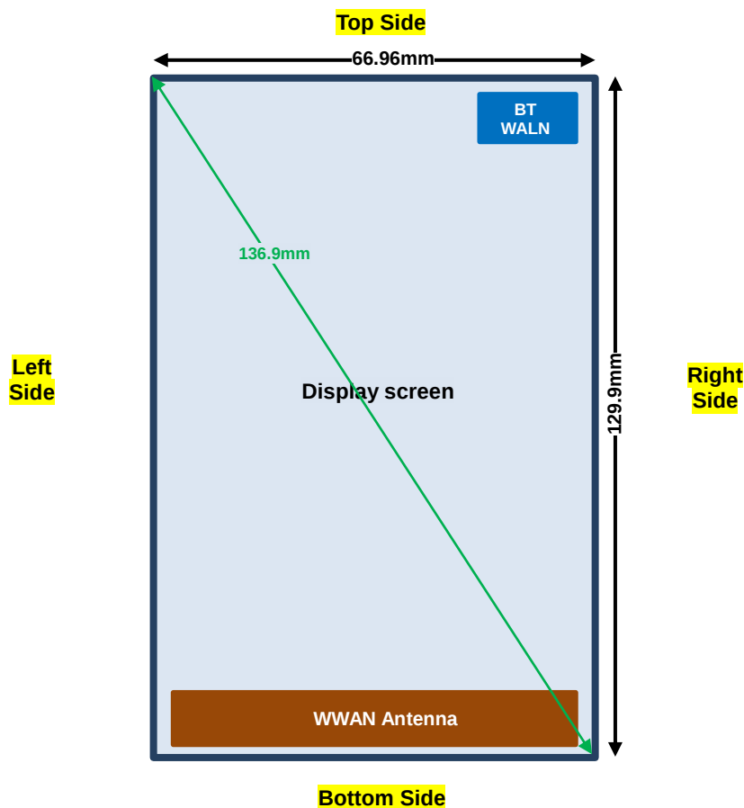
Front View
