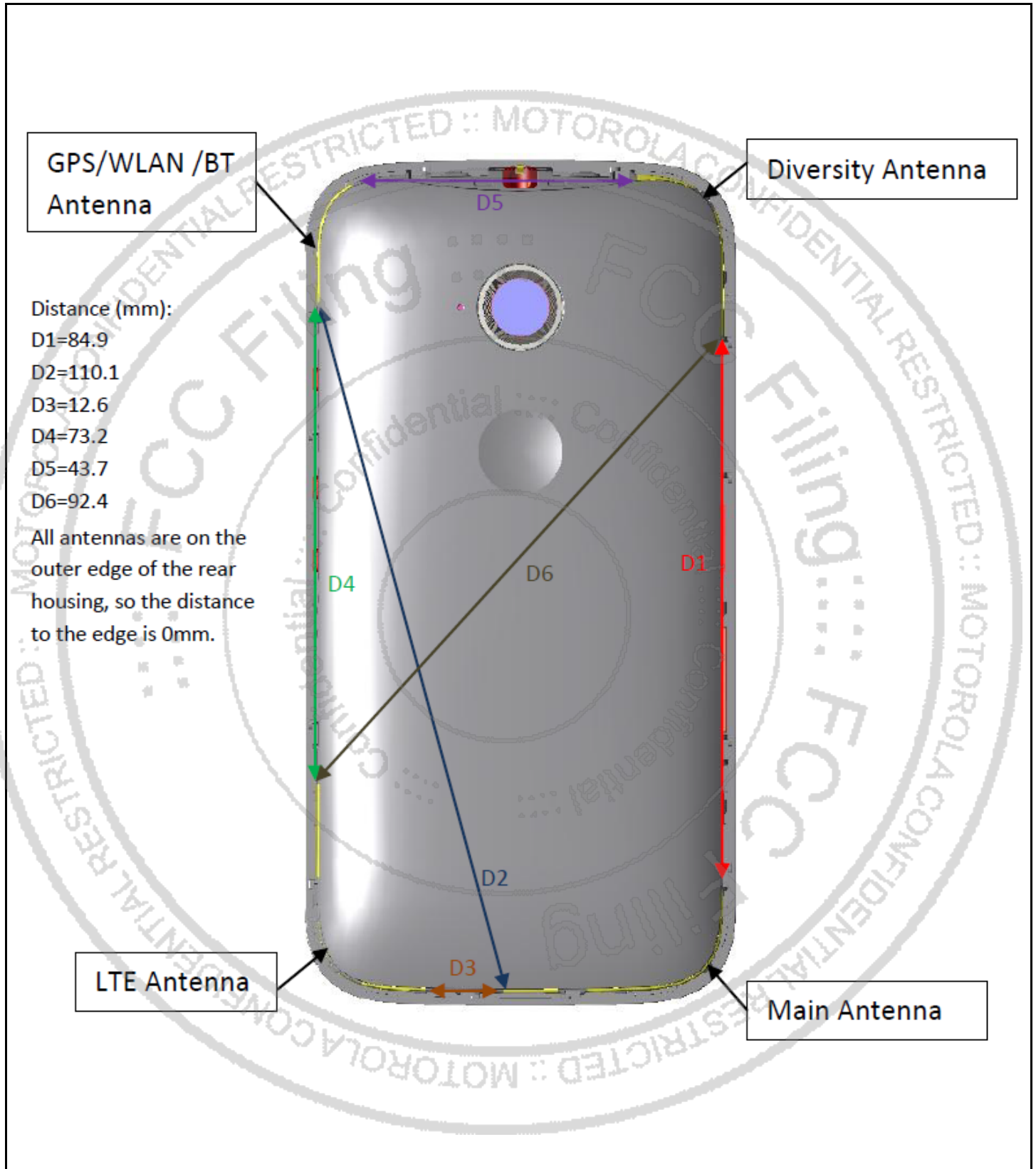
Photograph 9-4: Antenna Locations and Spacings.
