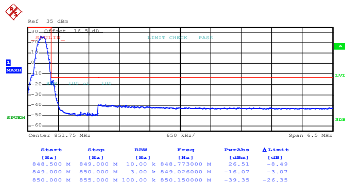
Higher Band Edge Plot on Channel 251 (848.8 MHz)
