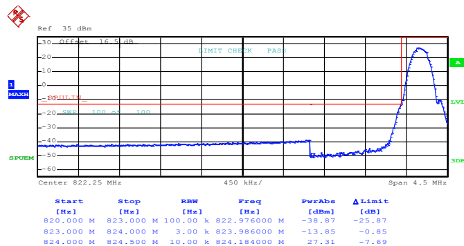
Lower Band Edge Plot on Channel 128 (824.2 MHz)
