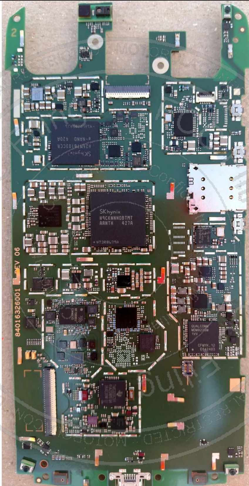
Photograph 9-3: Front side view of the device's PC Board, Shields Removed.
