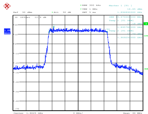
Highest Channel / 15MHz / 16QAM
