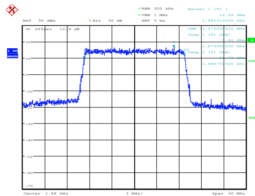
Middle Channel / 15MHz / 16QAM
