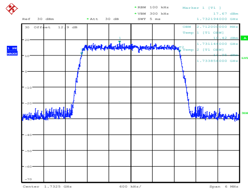
Middle Channel / 3MHz / 16QAM
