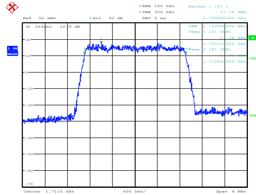
Lowest Channel / 3MHz / 16QAM
