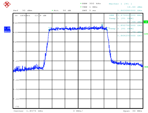
Lowest Channel / 15MHz / 16QAM
