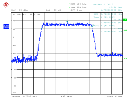
Highest Channel / 3MHz / 16QAM
