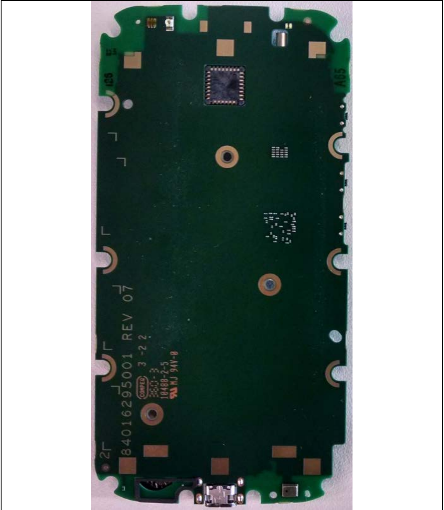
Photograph 9-3: Opposite Side view of the device's PC Board, Shields Removed.
