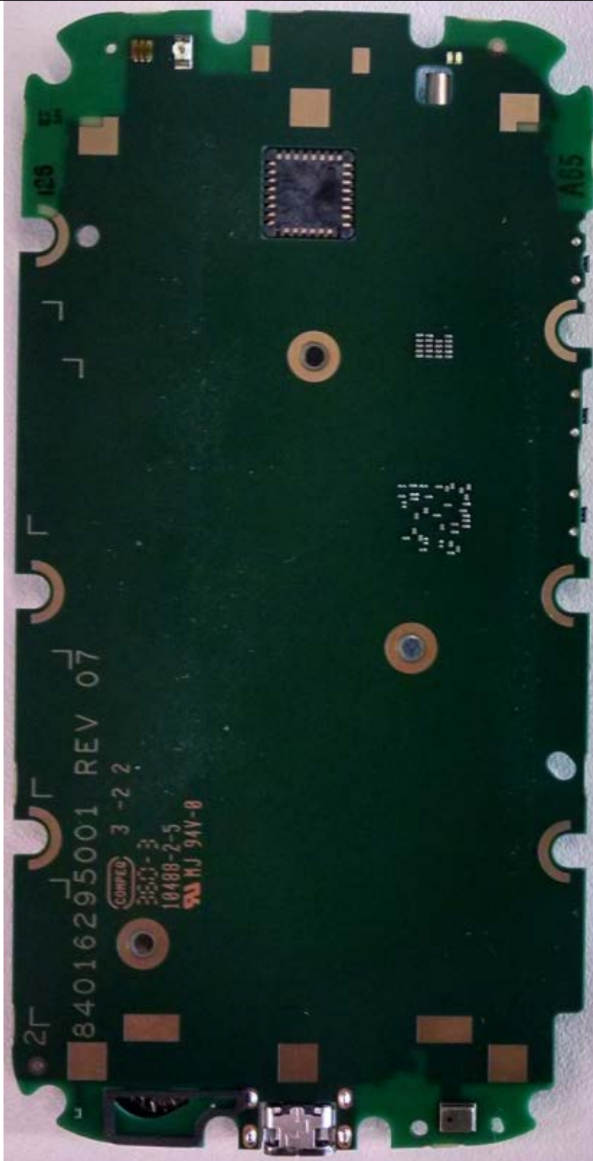
Photograph 9-3: Opposite Side view of the device's PC Board, Shields Removed.
