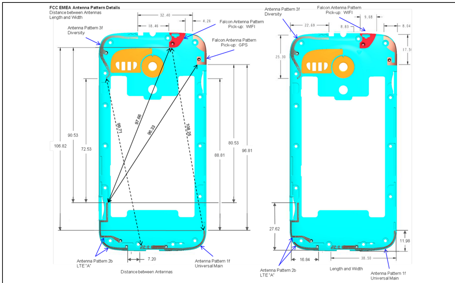
Photograph 9-5: Antenna Spacings.
