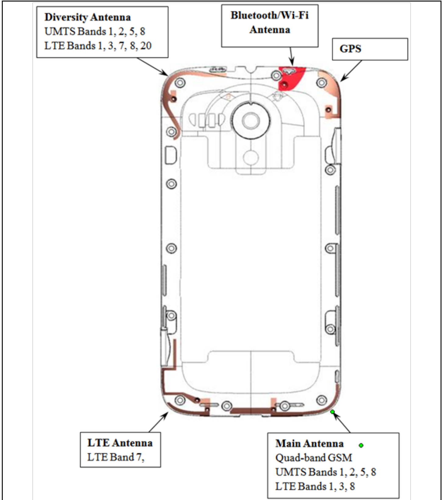
Photograph 9-4: Antenna Locations.
