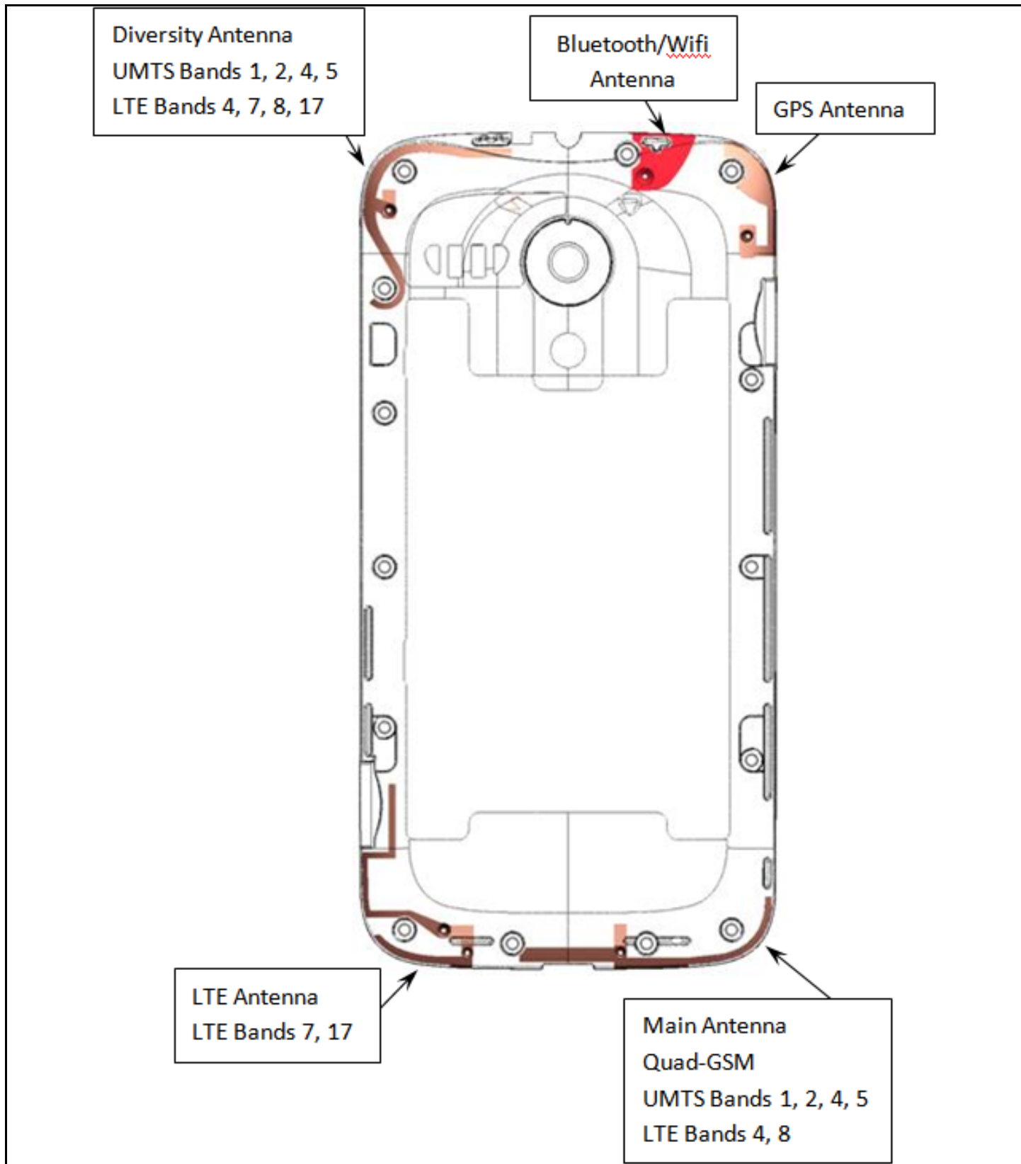
Photograph 9-4: Antenna Locations.
