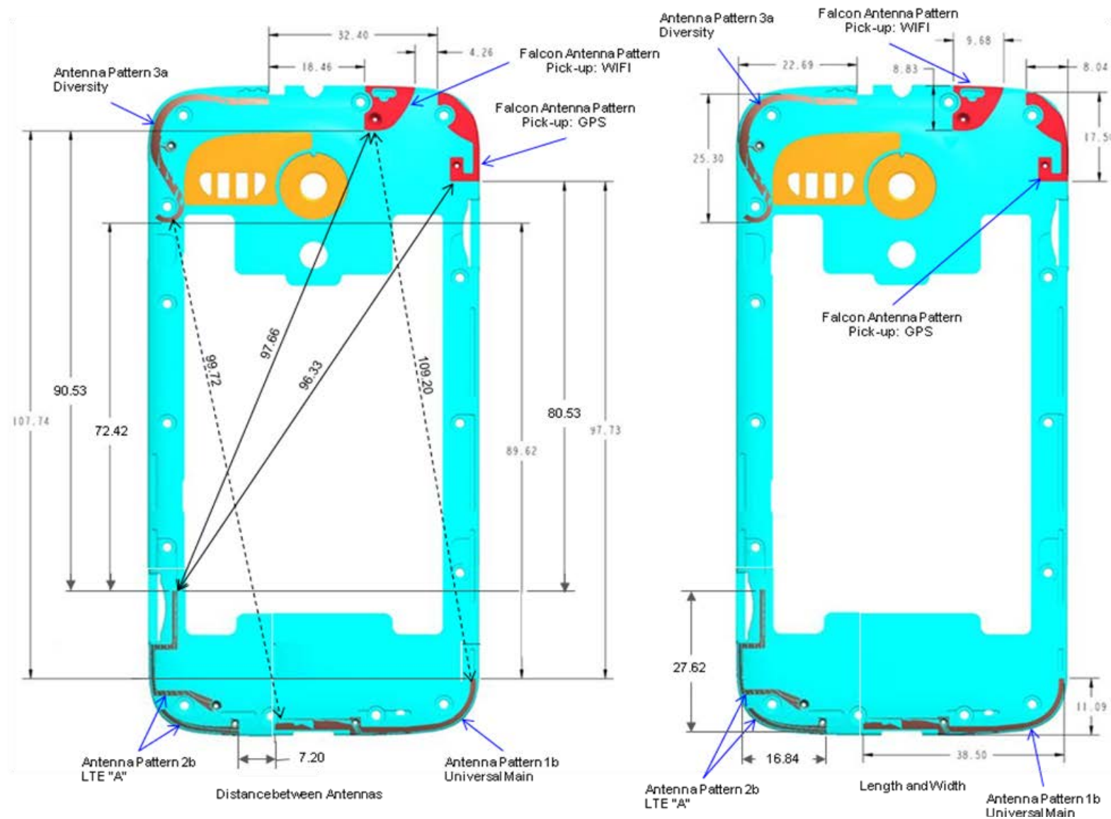
Photograph 9-5: Antenna Spacings.
