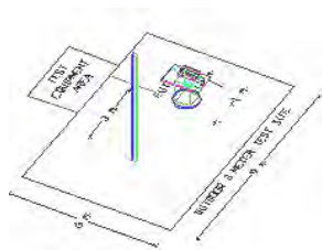
Figure 3-7. Turntable and System Setup
