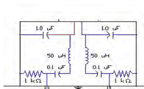
Figure 3-4. LISN Schematic Diagram
