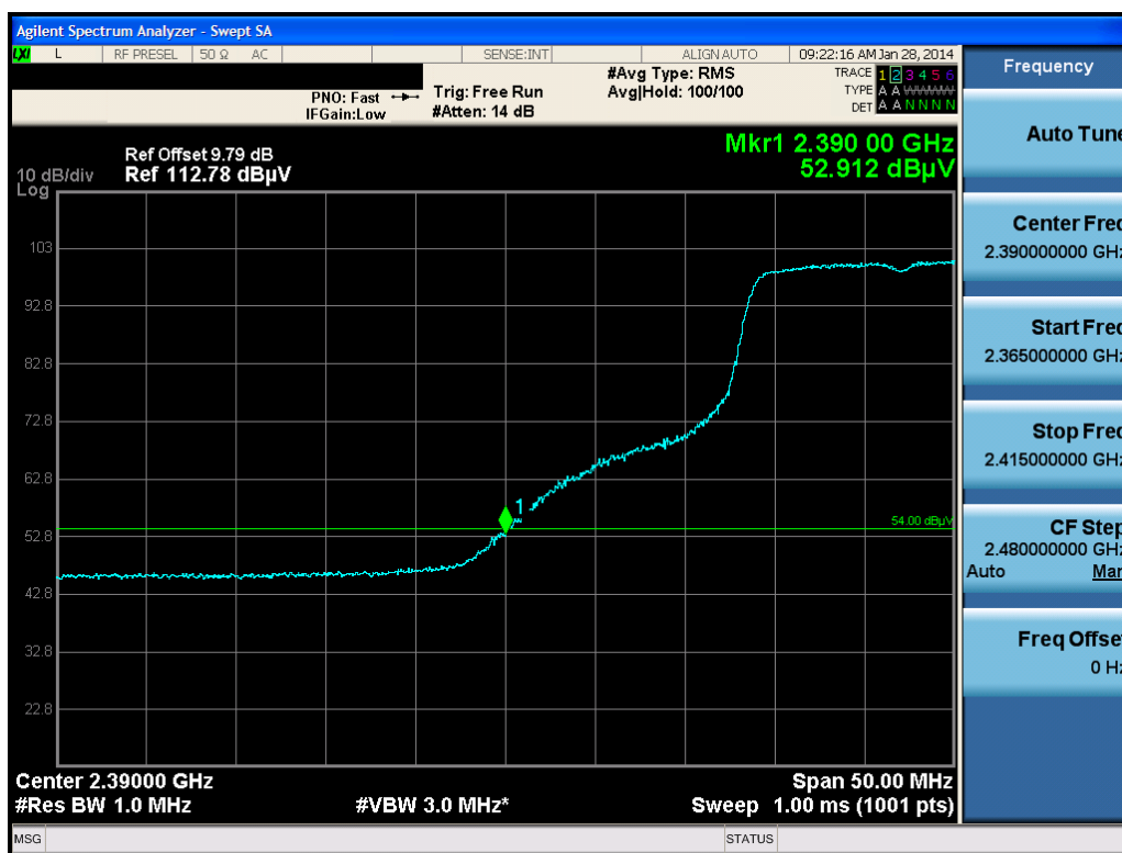
Plot 6-31. Radiated Restricted Lower Band Edge Measurement (Average)
