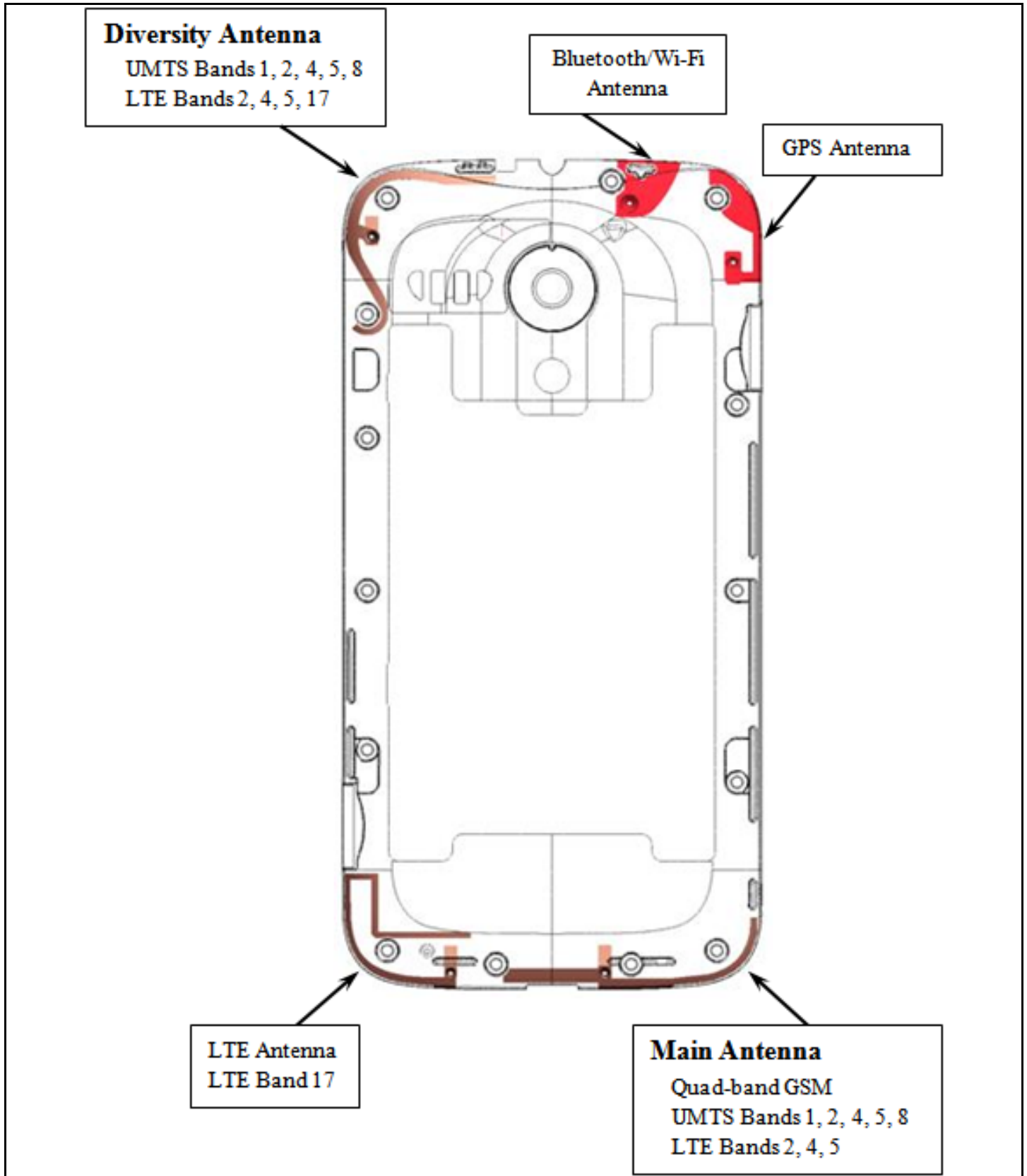
Photograph 9-4: Location of Antennas (Viewed from Rear).
