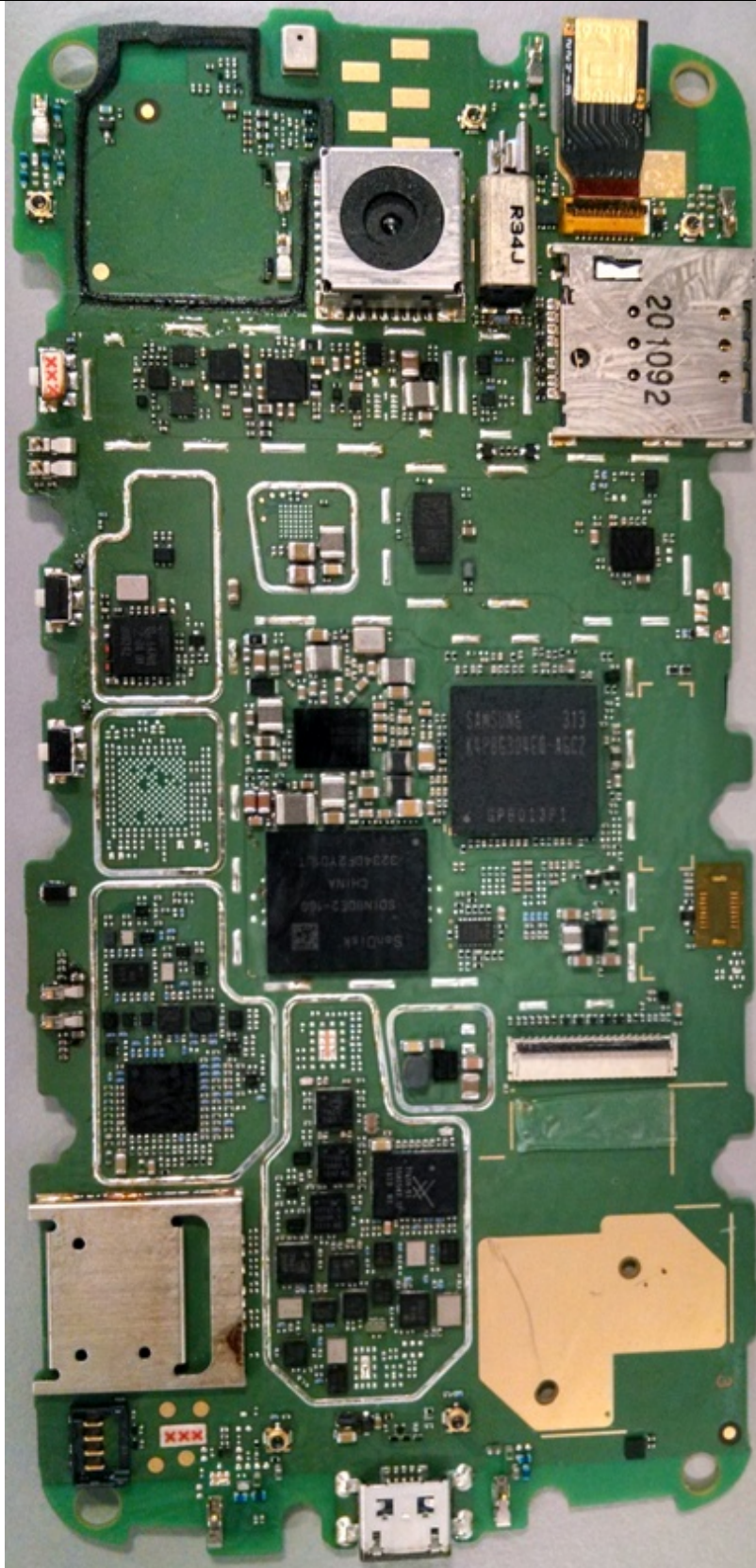
Photograph 9-2: Component side view of the device's PC Board, Shields removed.
