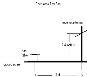
Figure 3-1. Diagram of 3-meter Test Range
