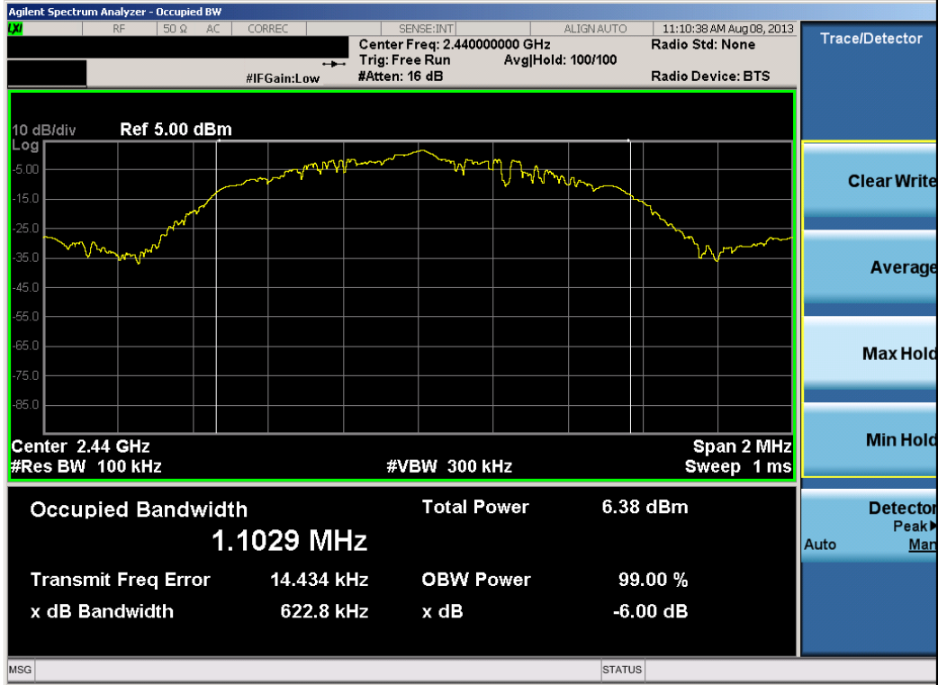
Plot 6-2. 6dB Bandwidth Plot (Bluetooth (LE) – Ch. 19)
