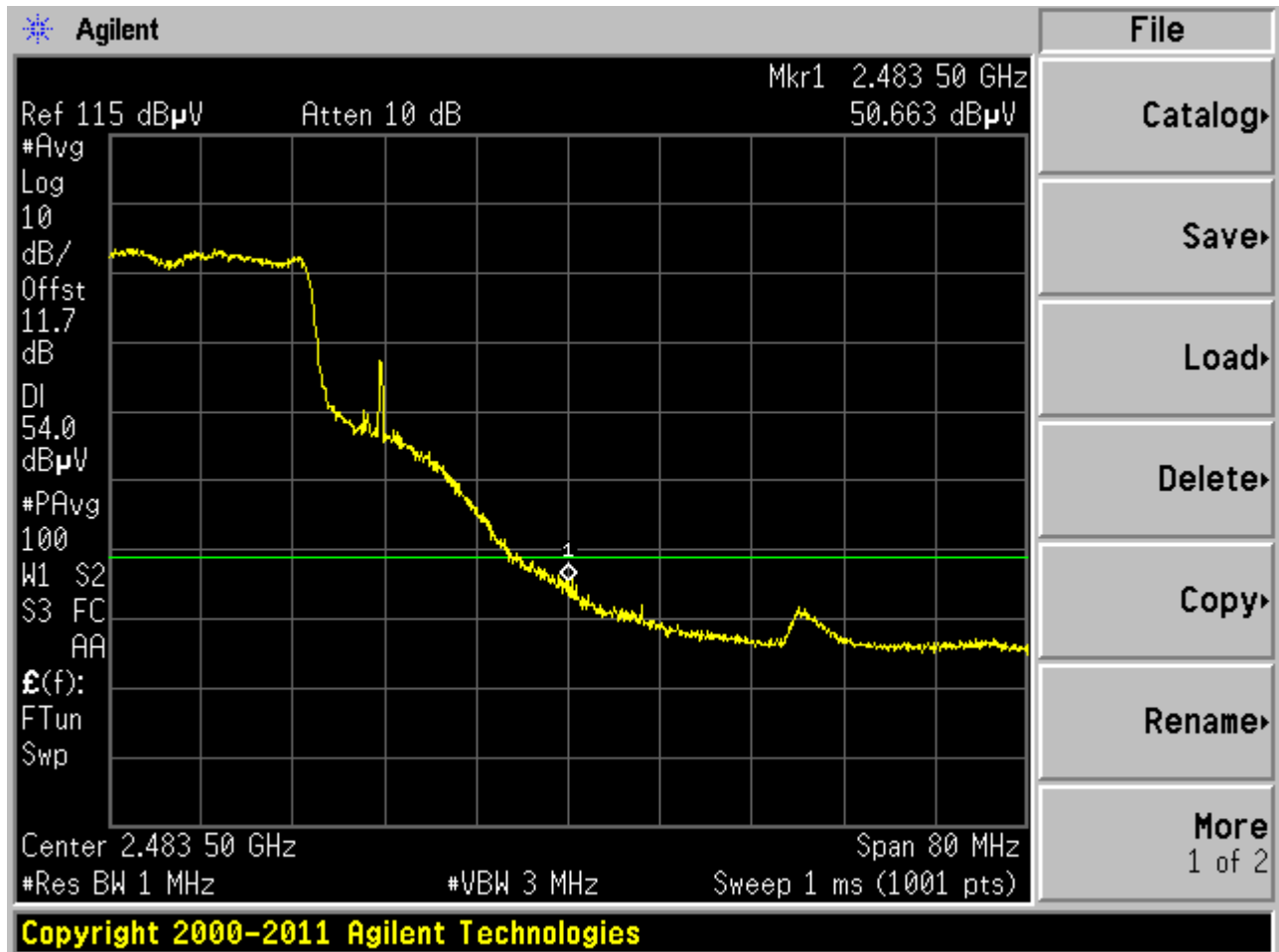
Plot 6-45. Radiated Restricted Upper Band Edge Measurement (Average)
