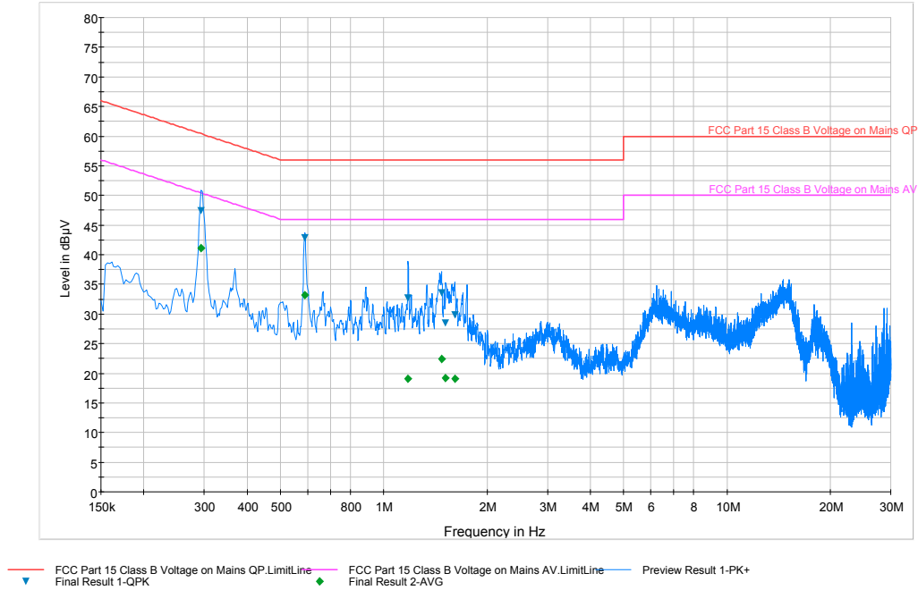
Plot 6-52. Line Conducted Plot with 802.11b (N)
