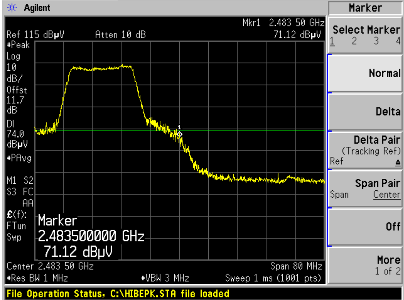
Plot 6-50. Radiated Restricted Upper Band Edge Measurement (Peak)
