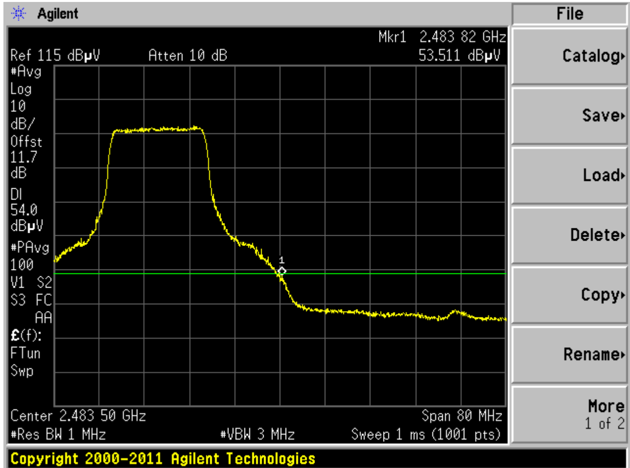
Plot 6-39. Radiated Restricted Upper Band Edge Measurement (Average)
