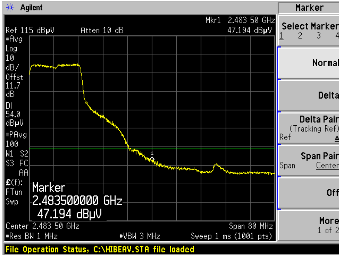
Plot 6-35. Radiated Restricted Upper Band Edge Measurement (Average)
