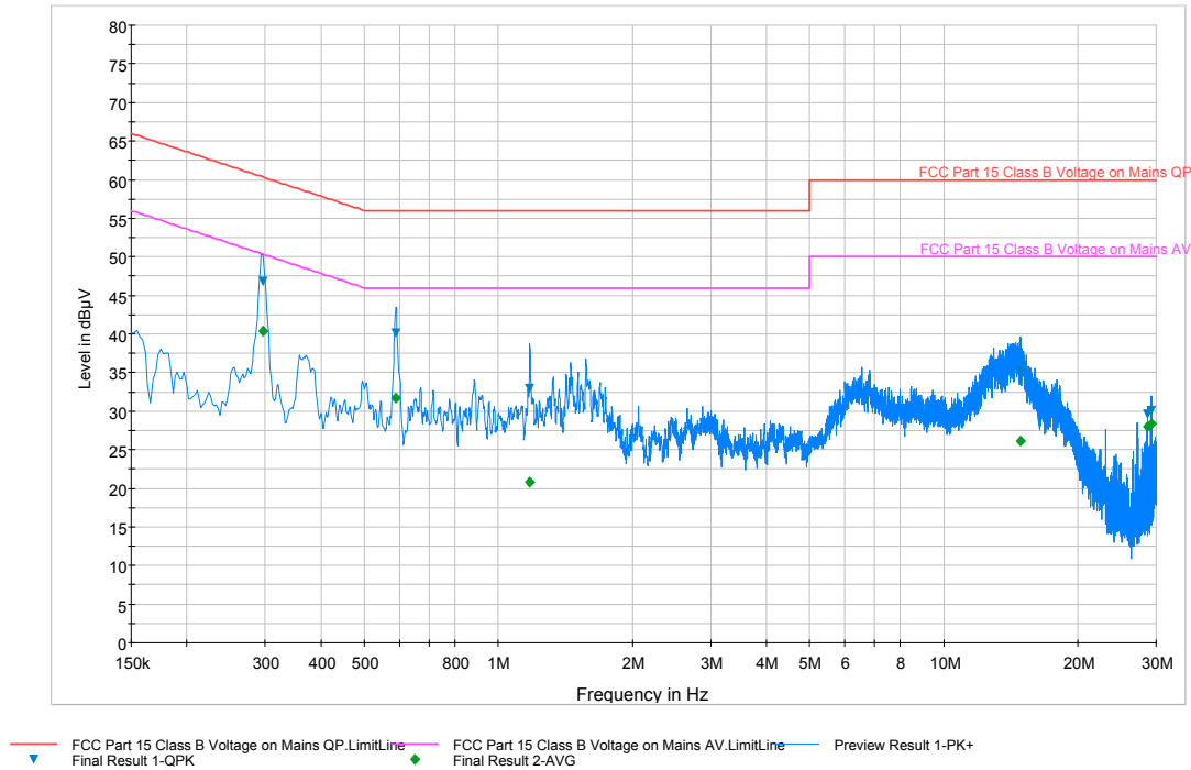
Plot 6-51. Line Conducted Plot with 802.11b (L1)
