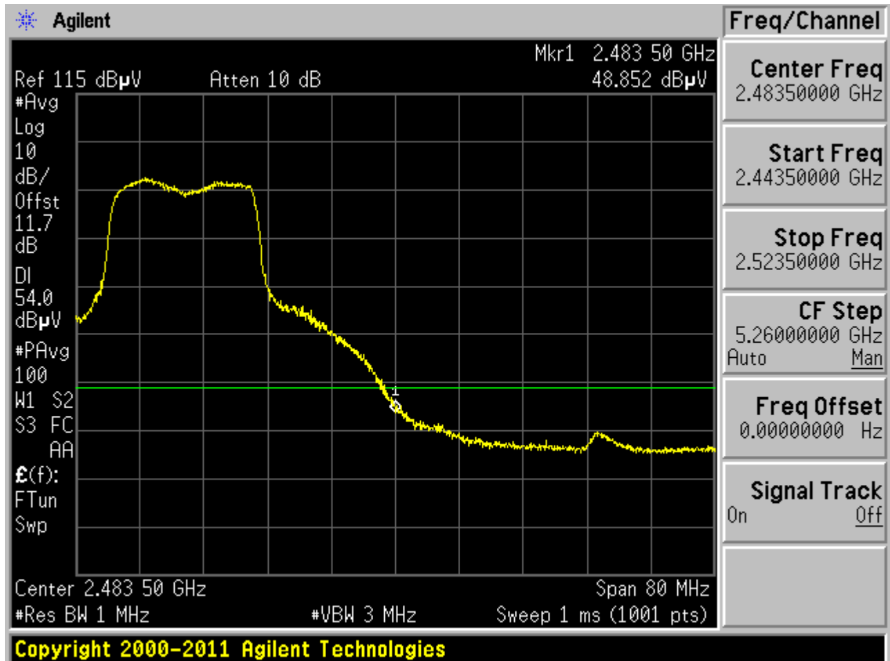
Plot 6-47. Radiated Restricted Upper Band Edge Measurement (Average)
