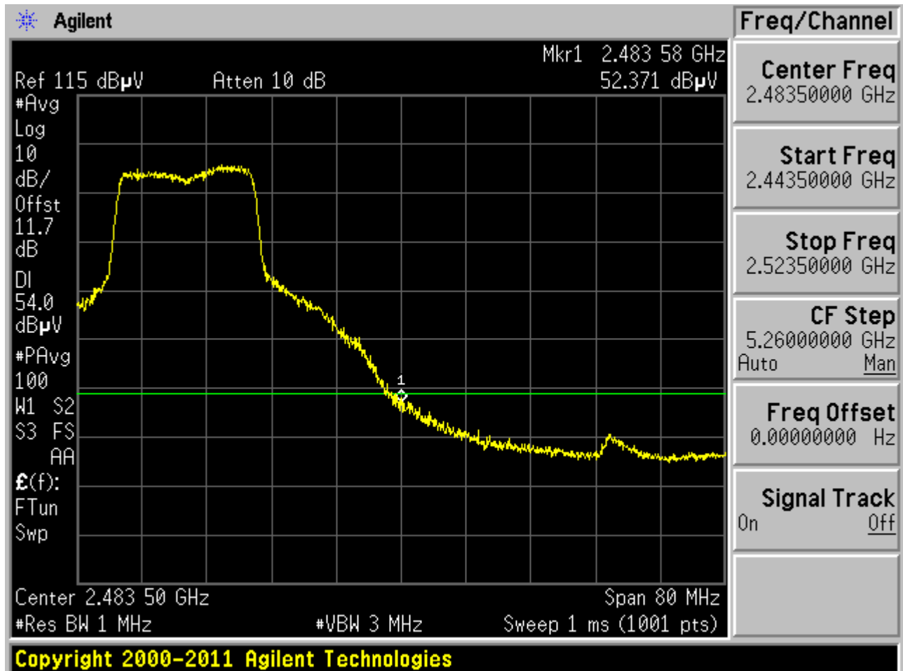
Plot 6-37. Radiated Restricted Upper Band Edge Measurement (Average)
