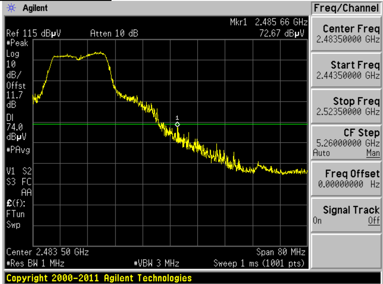
Plot 6-38. Radiated Restricted Upper Band Edge Measurement (Peak)
