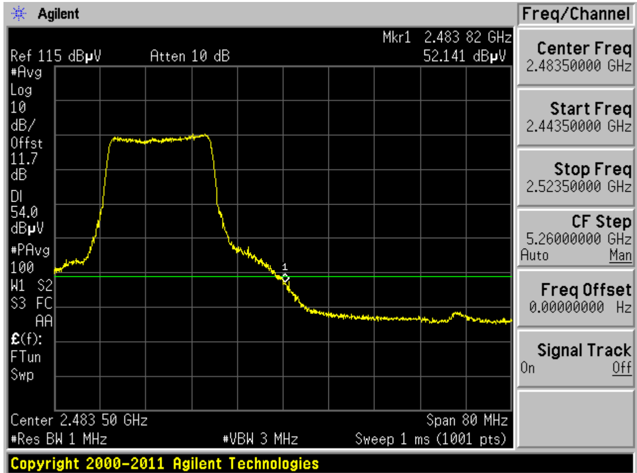
Plot 6-49. Radiated Restricted Upper Band Edge Measurement (Average)
