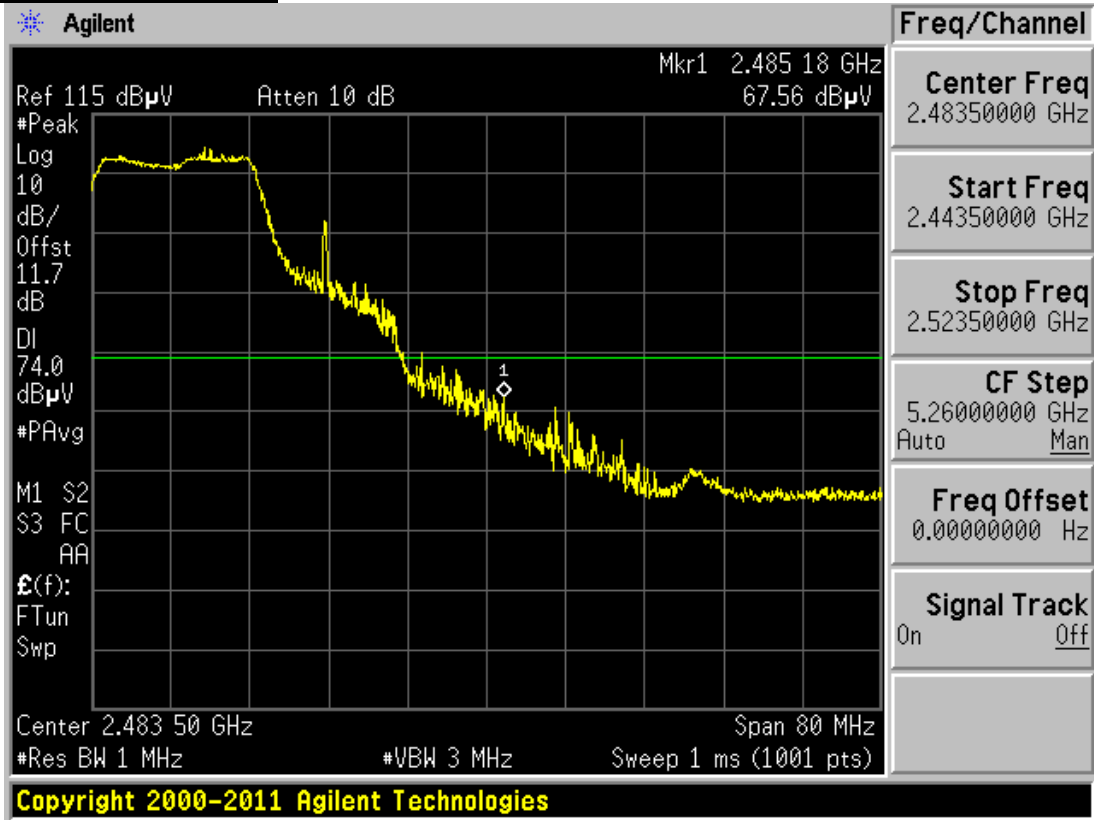
Plot 6-36. Radiated Restricted Upper Band Edge Measurement (Peak)
