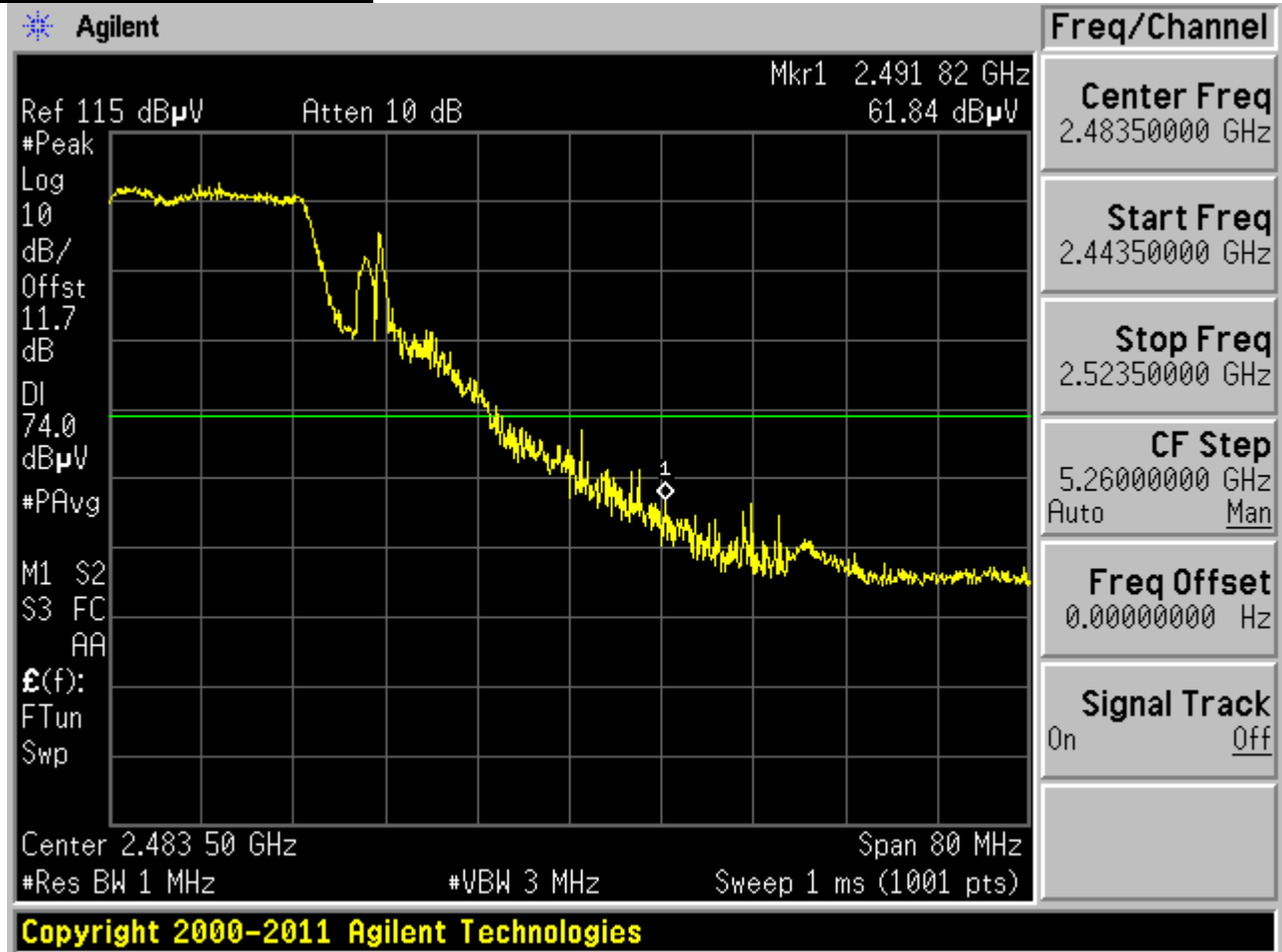
Plot 6-46. Radiated Restricted Upper Band Edge Measurement (Peak)
