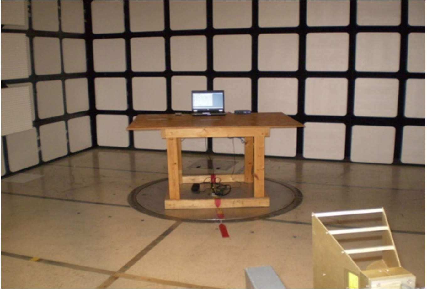
Figure 7B2-1: Spurious Radiations (Part 15 Computing Device).
