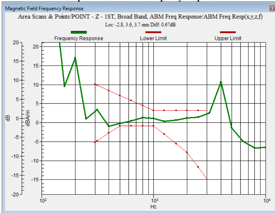
Graph 4: WCDMA 850 Frequency Response
