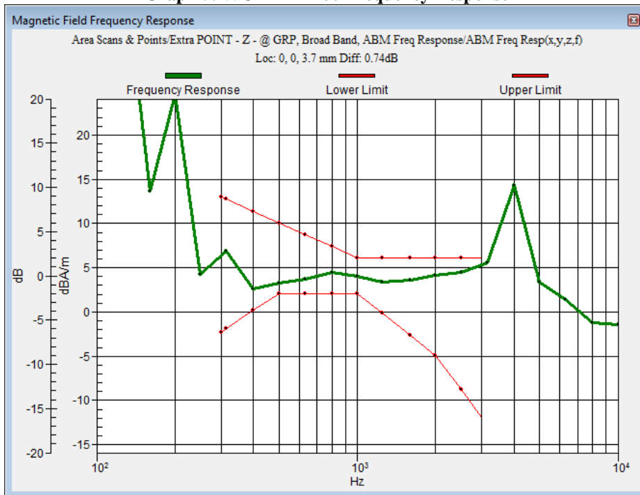
Graph 5: WCDMA 1700 Frequency Response
