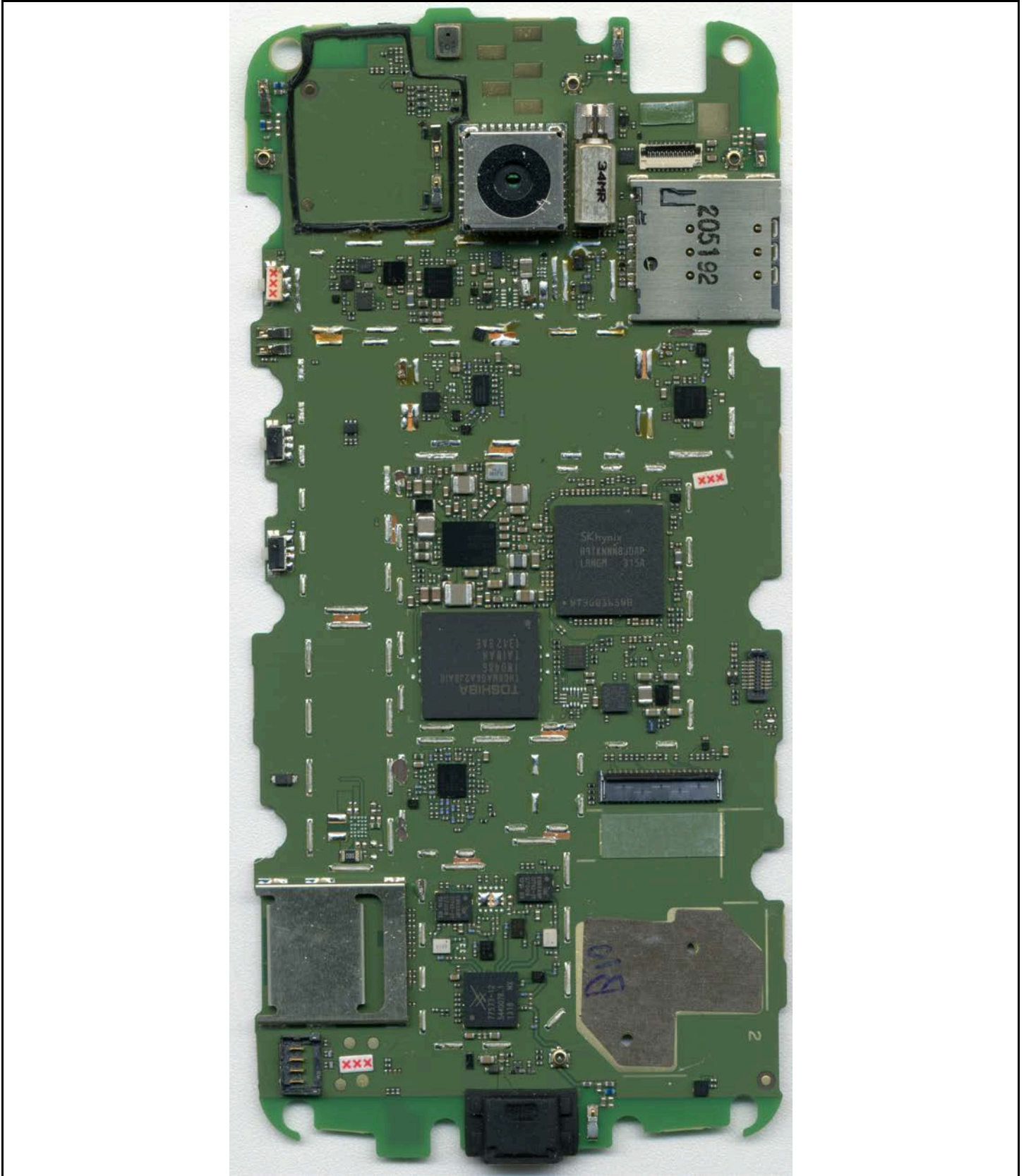
Photograph 9-3: Component side view of the device’s PC Board, Shields Removed.
