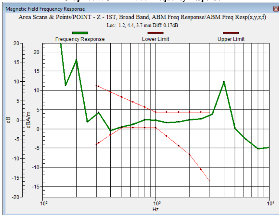
Graph 5: WCDMA 1900 Frequency Response
