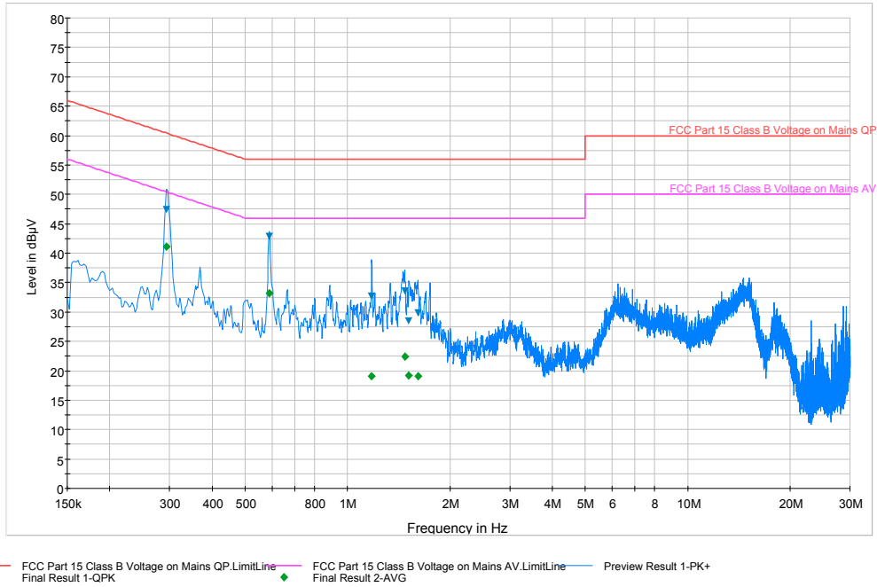
Plot 6-52. Line Conducted Plot with 802.11b (N)
