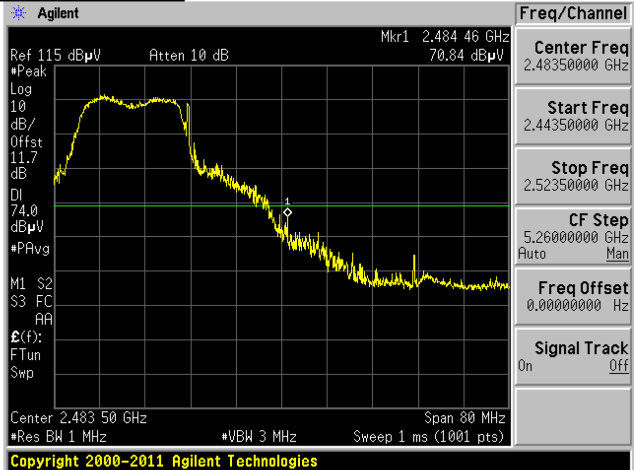
Plot 6-48. Radiated Restricted Upper Band Edge Measurement (Peak)
