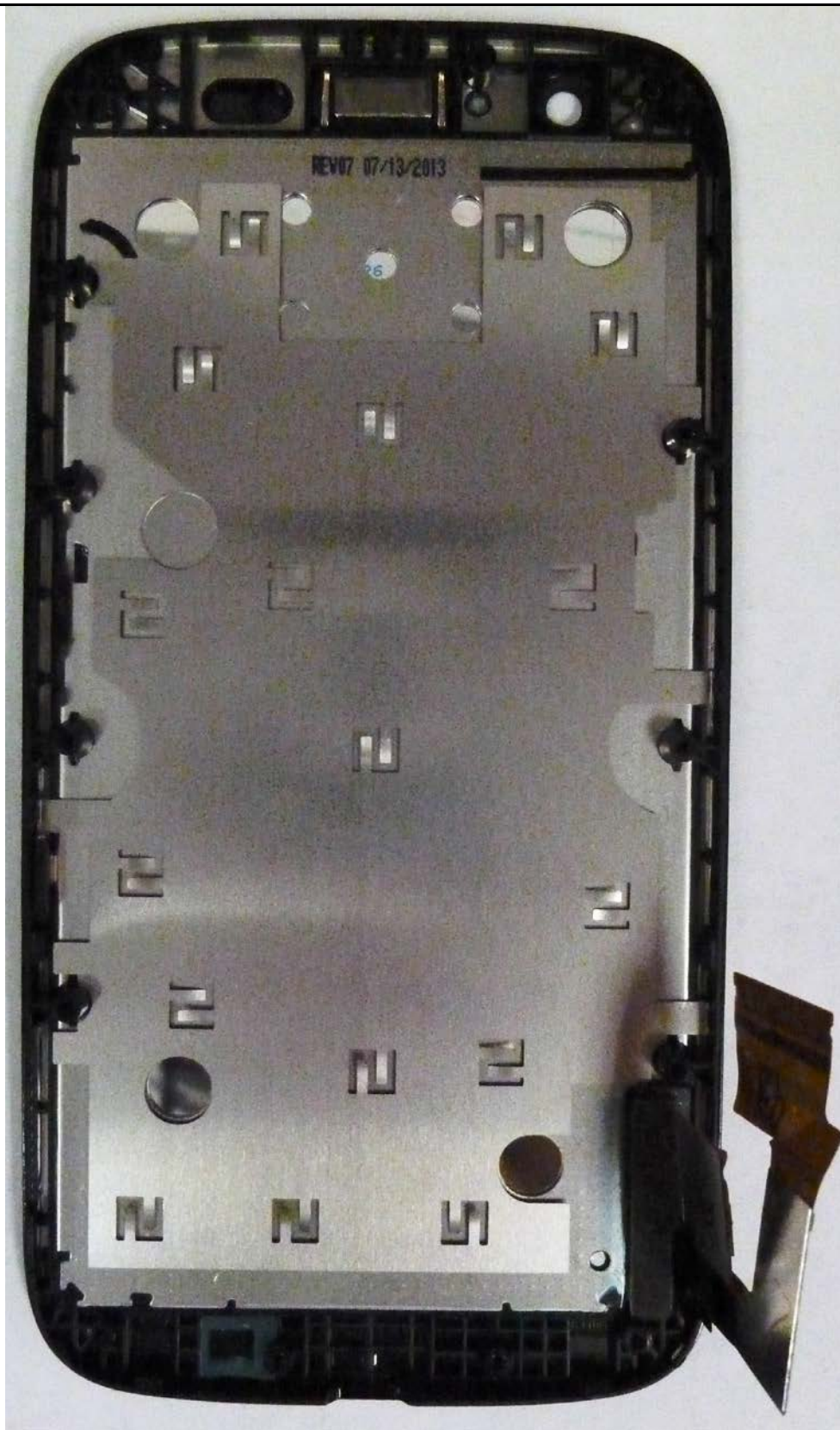
Photograph 9-4: Interior Housing View.
