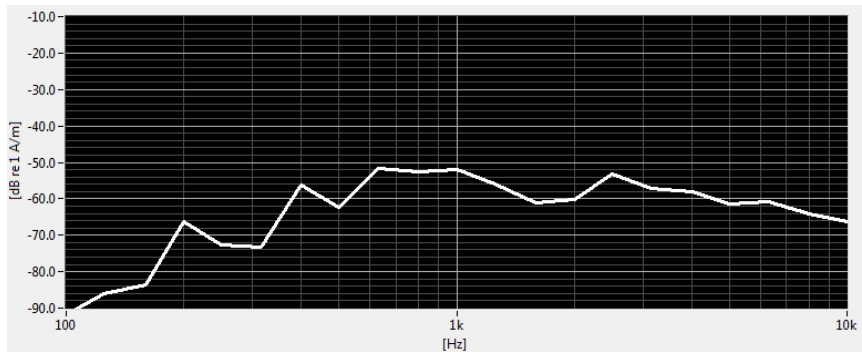
Figure 7-3 Worst-case ABM2 Plot for GSM
