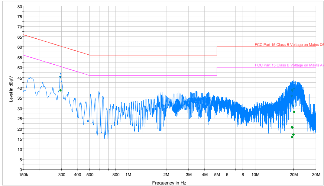
Plot 6-30. Line Conducted Plot with 802.11a UNII Band 1 (L1)
