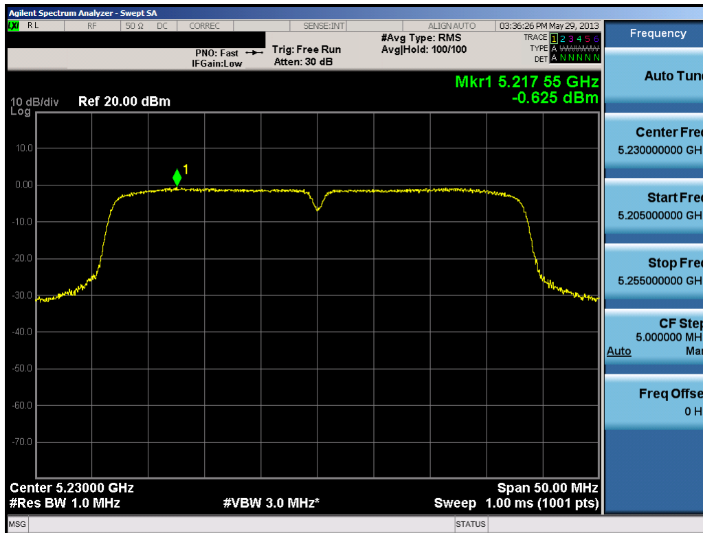
Plot 6-18. Peak Power Spectral Density Plot (40MHz BW 802.11n (UNII Band 1) – Ch. 46)
