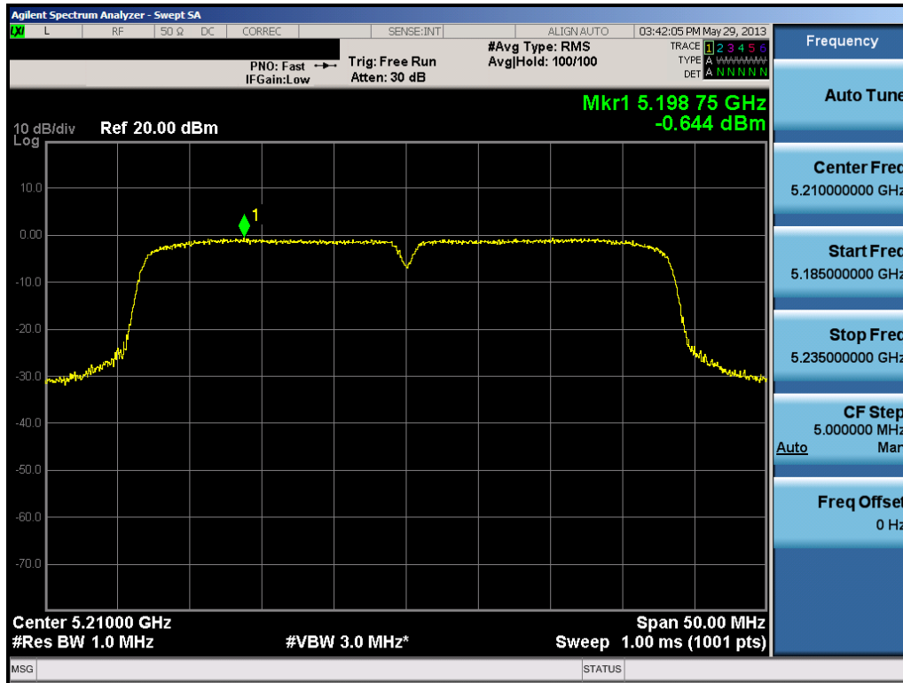
Plot 6-17. Peak Power Spectral Density Plot (40MHz BW 802.11n (UNII Band 1) – Ch. 42)
