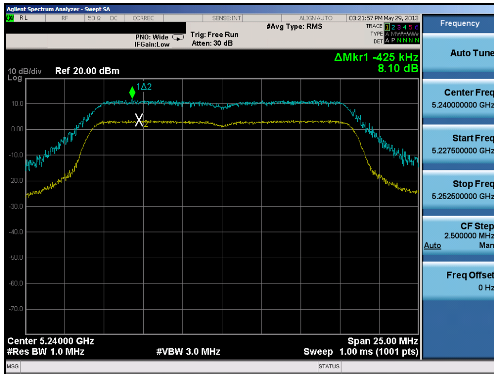
Plot 6-19. Peak Excursion Ratio Plot (802.11a)
