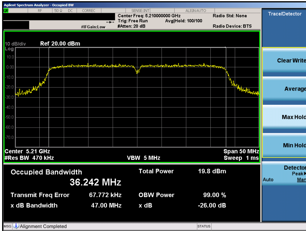
Plot 6-8. 26dB Bandwidth Plot (40MHz BW 802.11n (UNII Band 1) – Ch. 42)
