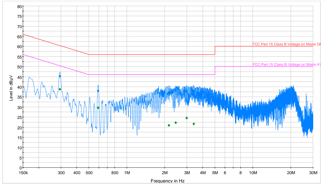
— FCC Part 15 Class B Voltage on Mains QP.LimitLine — FCC Part 15 Class B Voltage on Mains AV.LimitLine — Preview Result 1-PK+ ▼ Final Result 1-QPK ◆ Final Result 2-AVC
