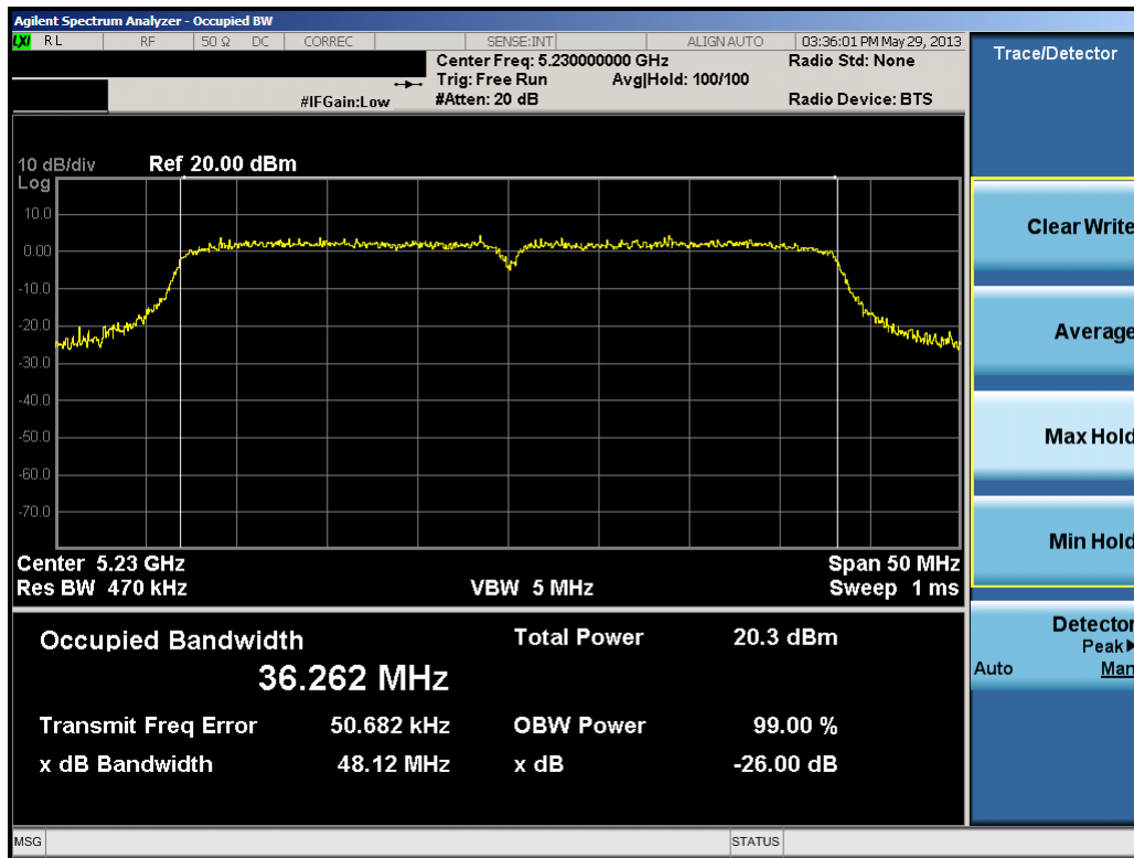
Plot 6-9. 26dB Bandwidth Plot (40MHz BW 802.11n (UNII Band 1) – Ch. 46)
