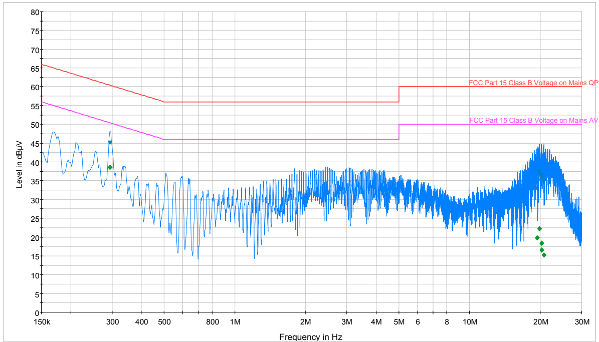
Plot 6-22. Line Conducted Plot with Bluetooth LE (L1)
