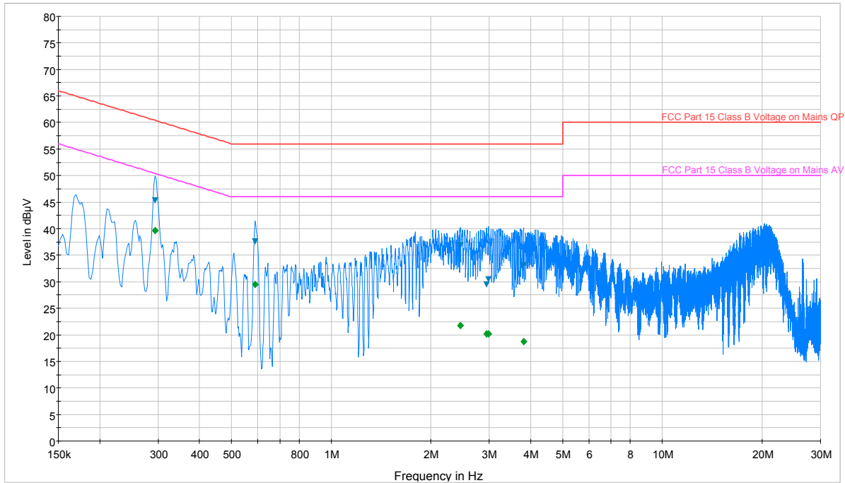
Plot 6-23. Line Conducted Plot with Bluetooth LE (N)
