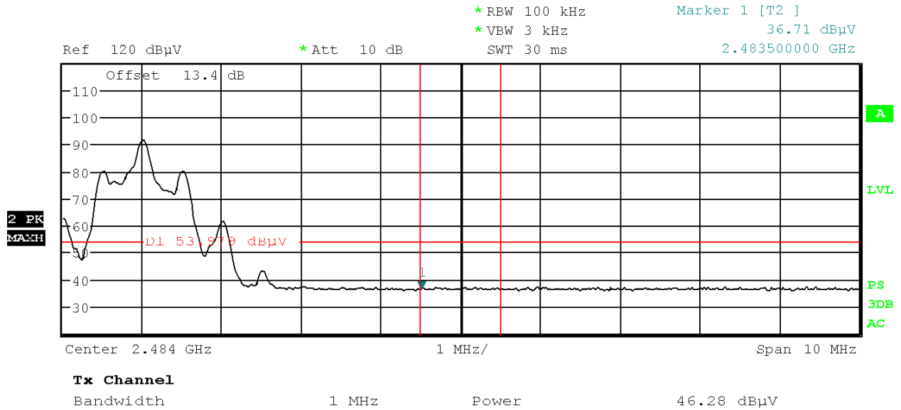
Plot 6-20. Radiated Restricted Upper Band Edge Measurement with WCP (Average)
