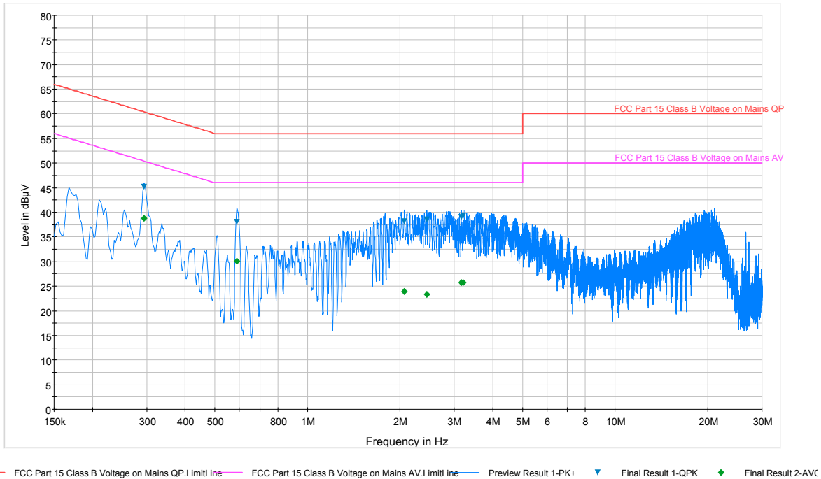
Plot 6-80. Line Conducted Plot with 802.11a (N)
