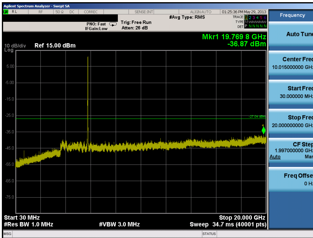
Plot 6-57. Conducted Spurious Plot (802.11a – Ch. 157)
