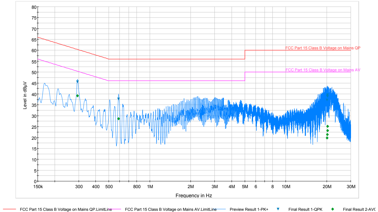
Plot 6-77. Line Conducted Plot with 802.11b (L1)
