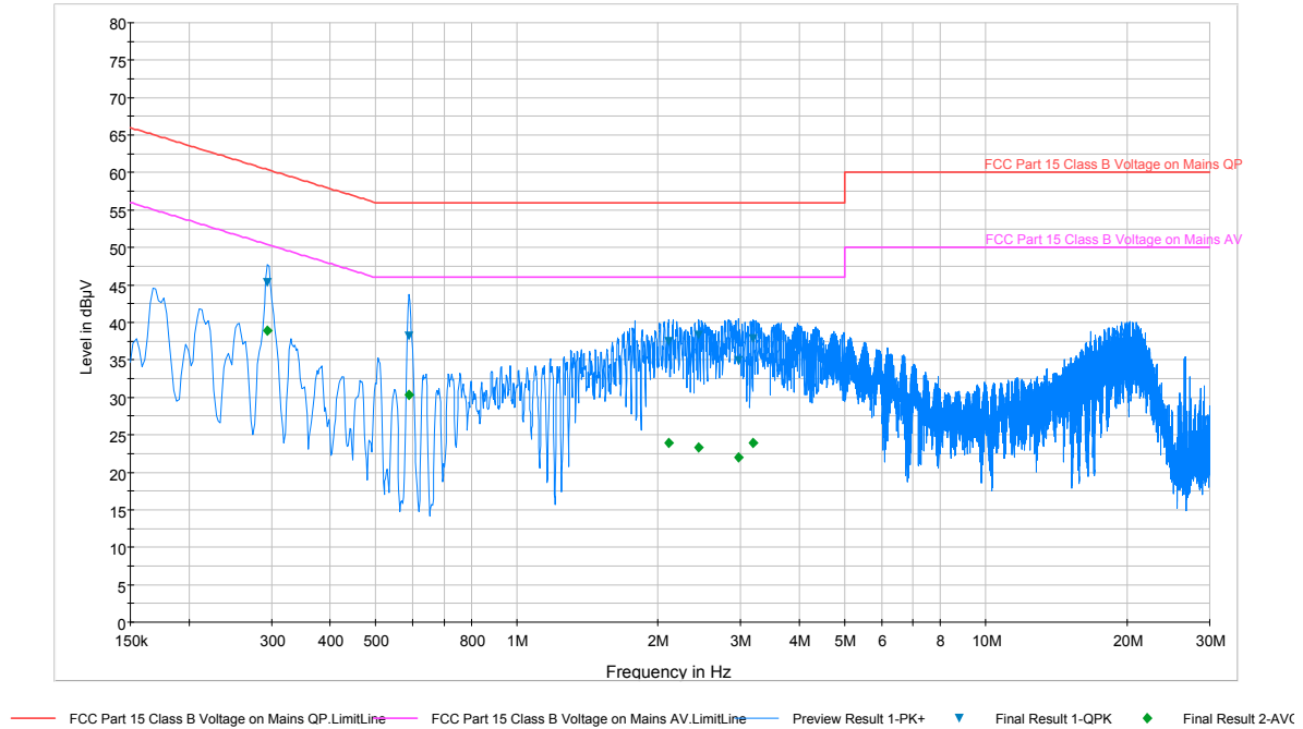
Plot 6-78. Line Conducted Plot with 802.11b (N)
