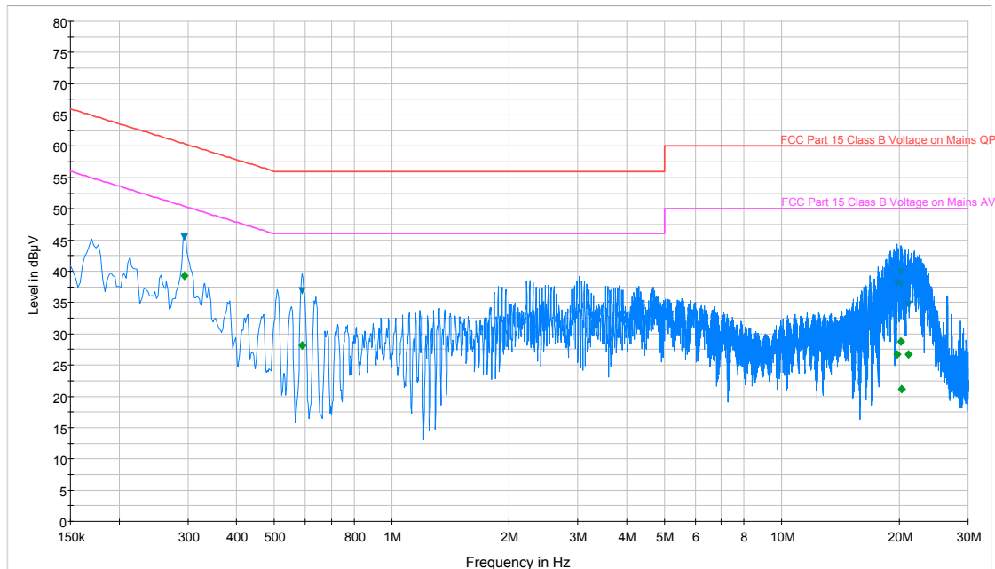
Plot 6-79. Line Conducted Plot with 802.11a (L1)
