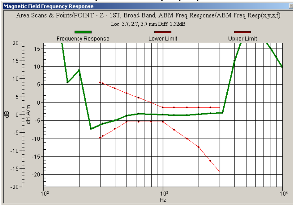
Graph 4: GSM 850 Frequency Response
