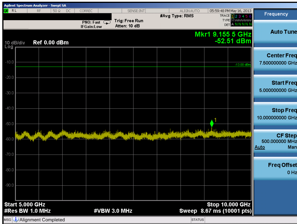
Plot 7-56. Conducted Spurious Plot (Cellular WCDMA Mode – Ch. 4233)
