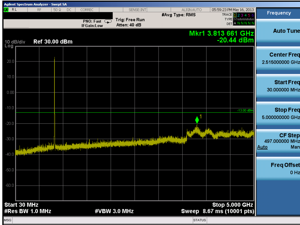
Plot 7-55. Conducted Spurious Plot (Cellular WCDMA Mode – Ch. 4233)
