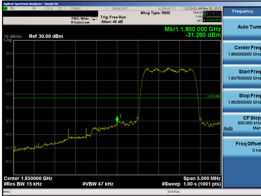
Plot 7-39. Band Edge Plot (PCS CDMA Mode – Ch. 25)
