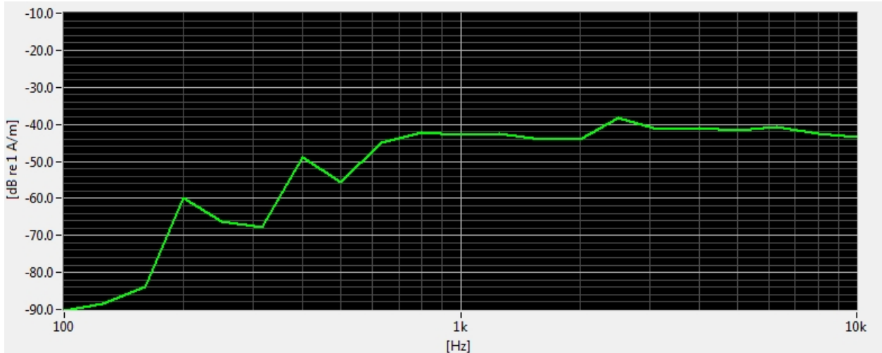
Figure 7-4 Worst-case ABM2 Plot for GSM
