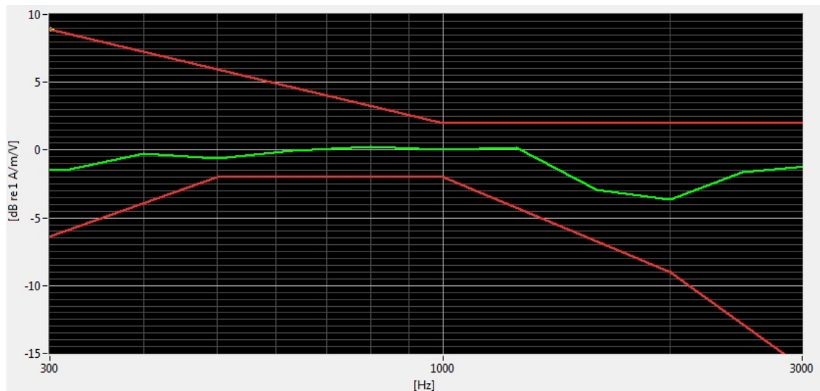
Figure 7-2 Axial Frequency Response for GSM and UMTS
