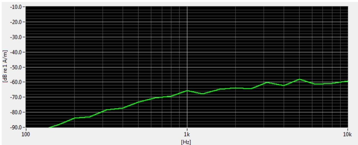
Figure 7-5 Worst-case ABM2 Plot for UMTS
