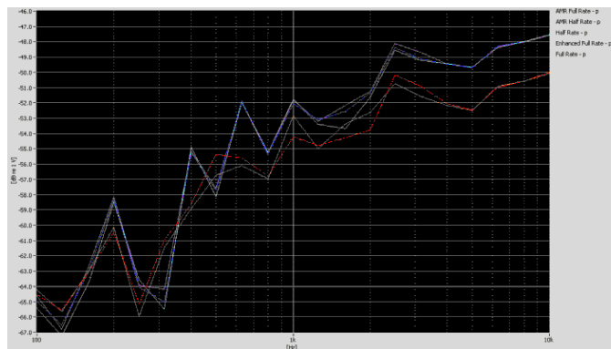
Figure 5-11 Vocoder Analysis for ABM Noise
