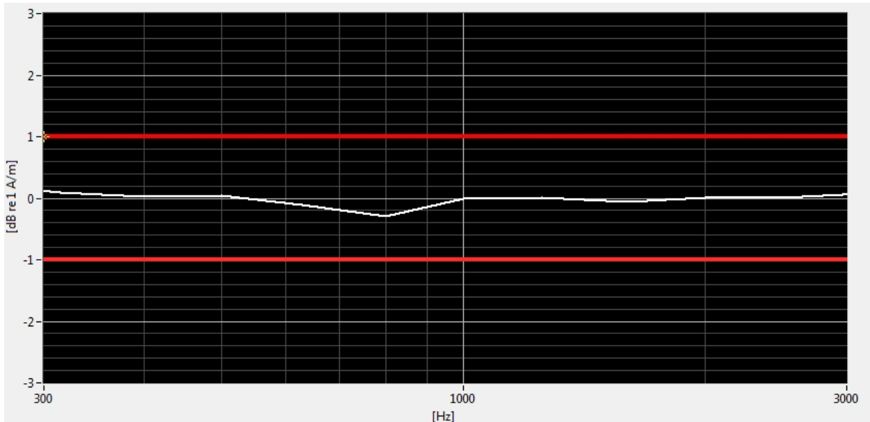
Figure 7-6 Helmholtz Coil Validation for Frequency Response
