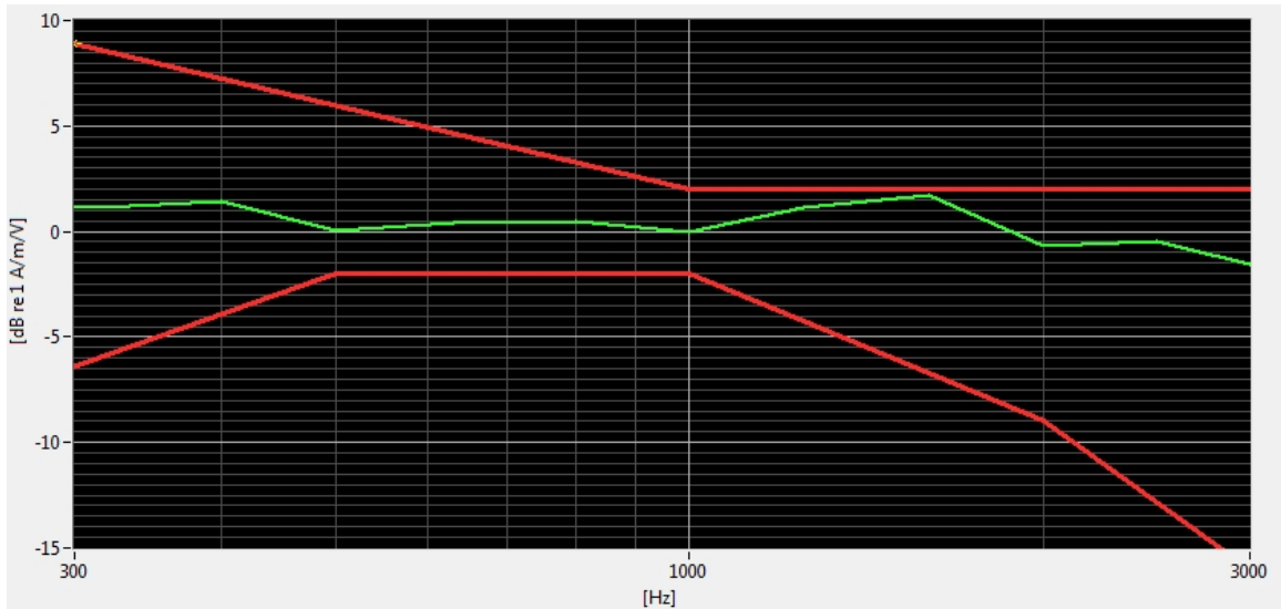
Figure 7-1 Axial Frequency Response for CDMA
