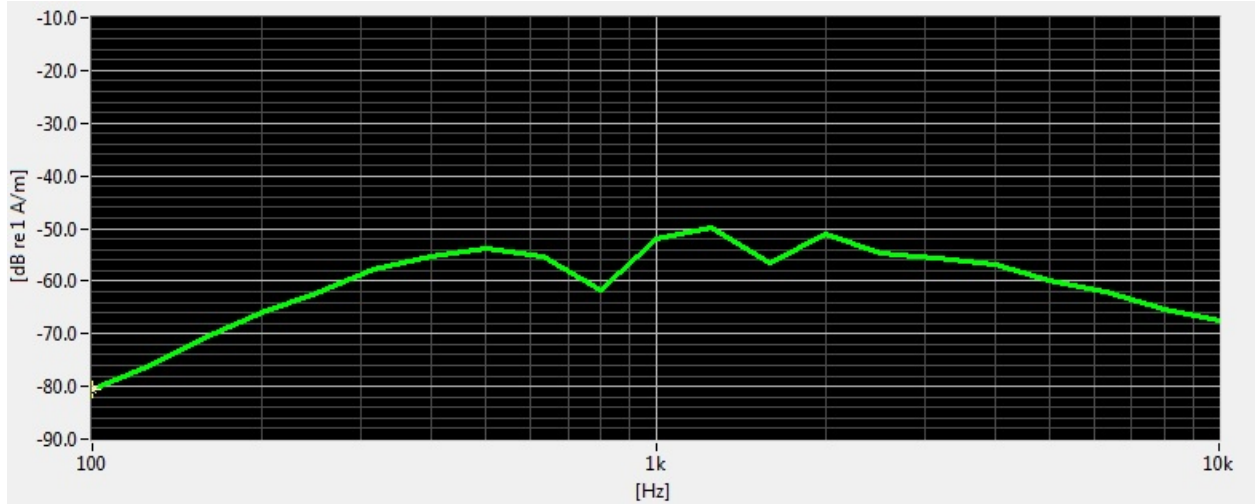
Figure 7-3 Worst-case ABM2 Plot for CDMA
