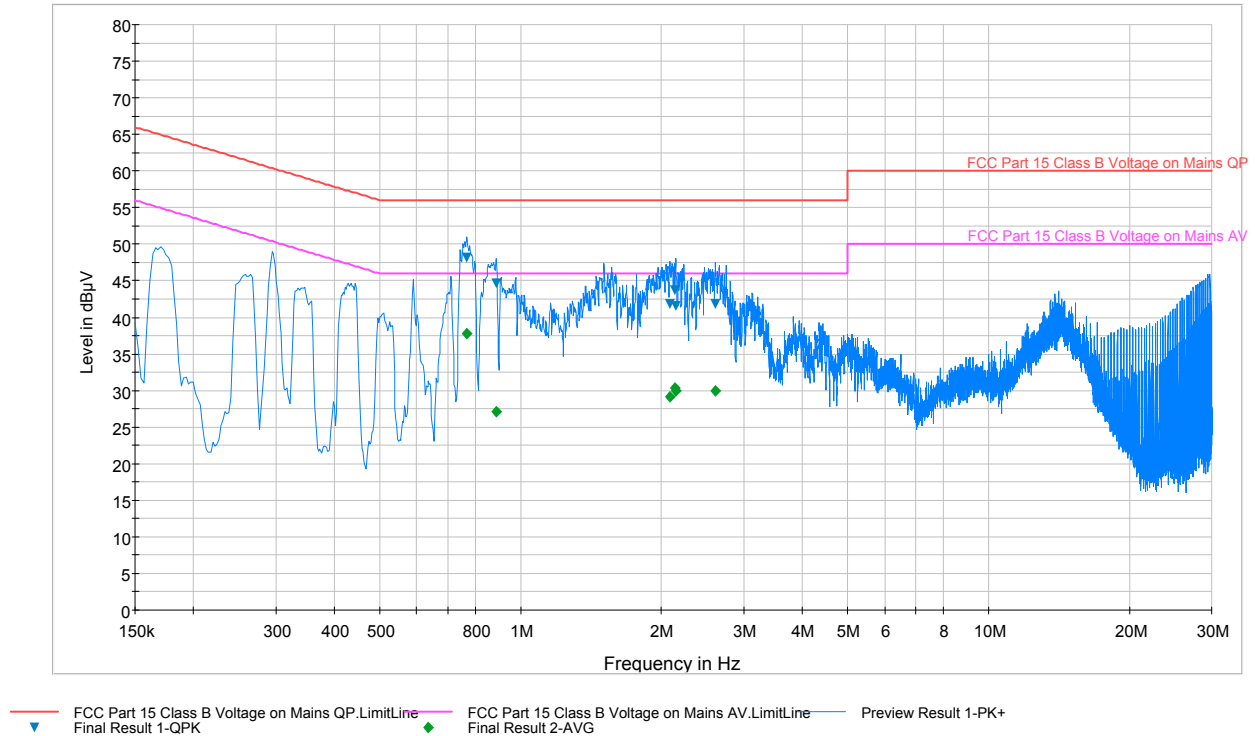
Plot 6-49. Line-Conducted Test Plot (N w/ WCP)
