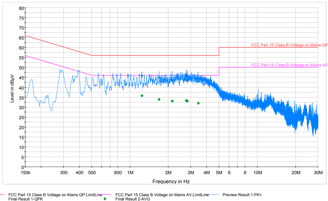
Plot 6-47. Line-Conducted Test Plot (N)
