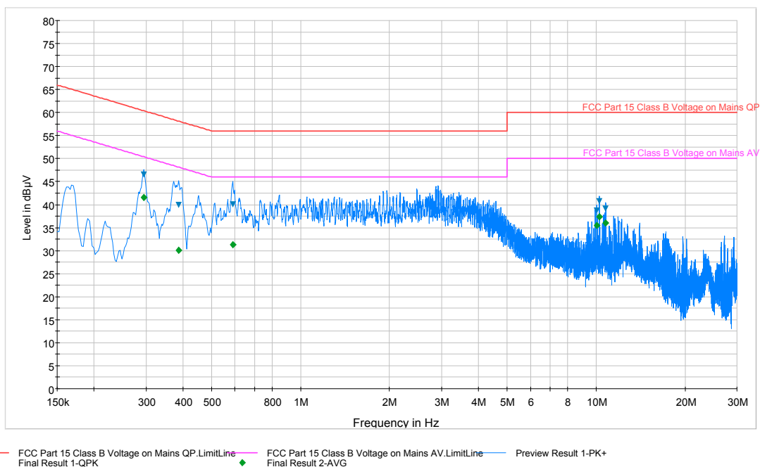
Plot 6-46. Line-Conducted Test Plot (L1)
