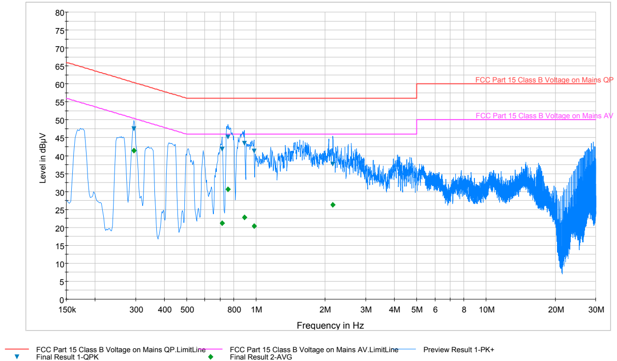
Plot 6-48. Line-Conducted Test Plot (L1 w/ WCP)
