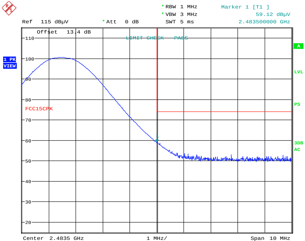
Plot 6-45. Radiated Restricted Upper Band Edge Measurement (Peak – WCP)
