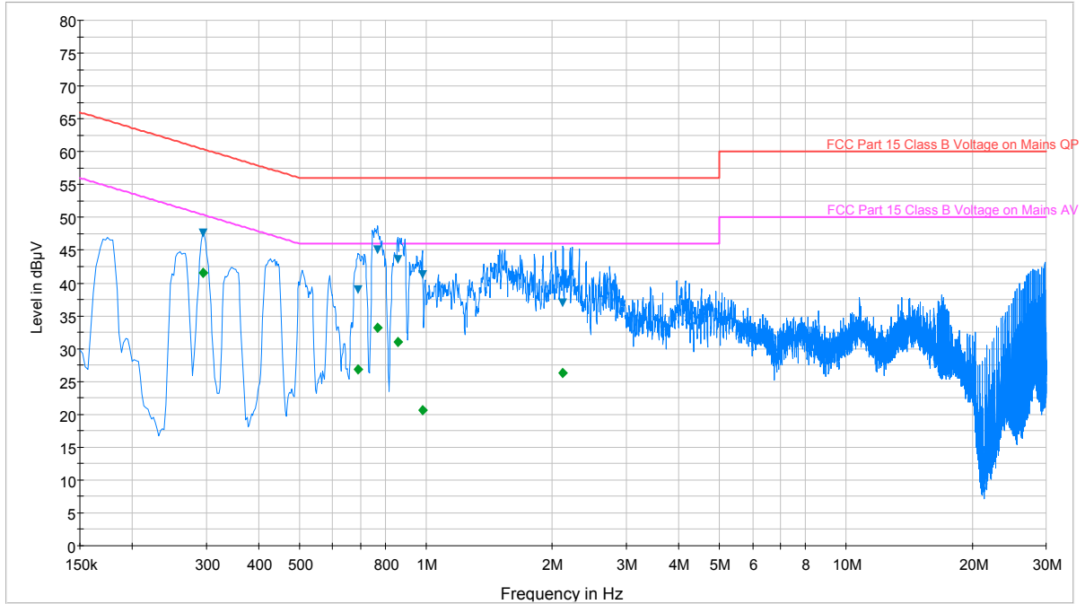
Plot 6-24. Line Conducted Plot with Bluetooth LE (L1 w/ WCP)
