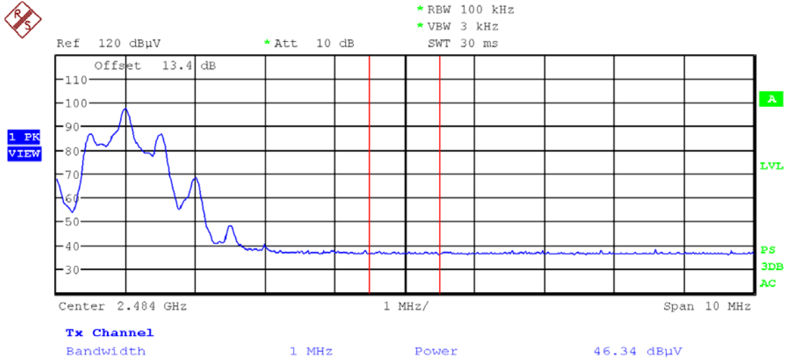
Plot 6-20. Radiated Restricted Upper Band Edge Measurement (Average – WCP)
