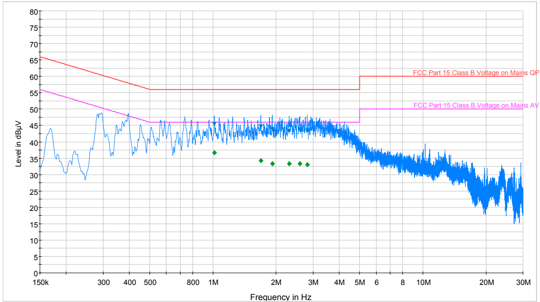
Plot 6-23. Line Conducted Plot with Bluetooth LE (N)
