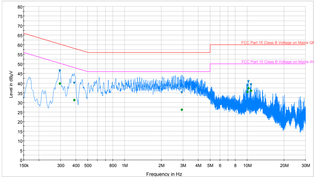
Plot 6-22. Line Conducted Plot with Bluetooth LE (L1)
