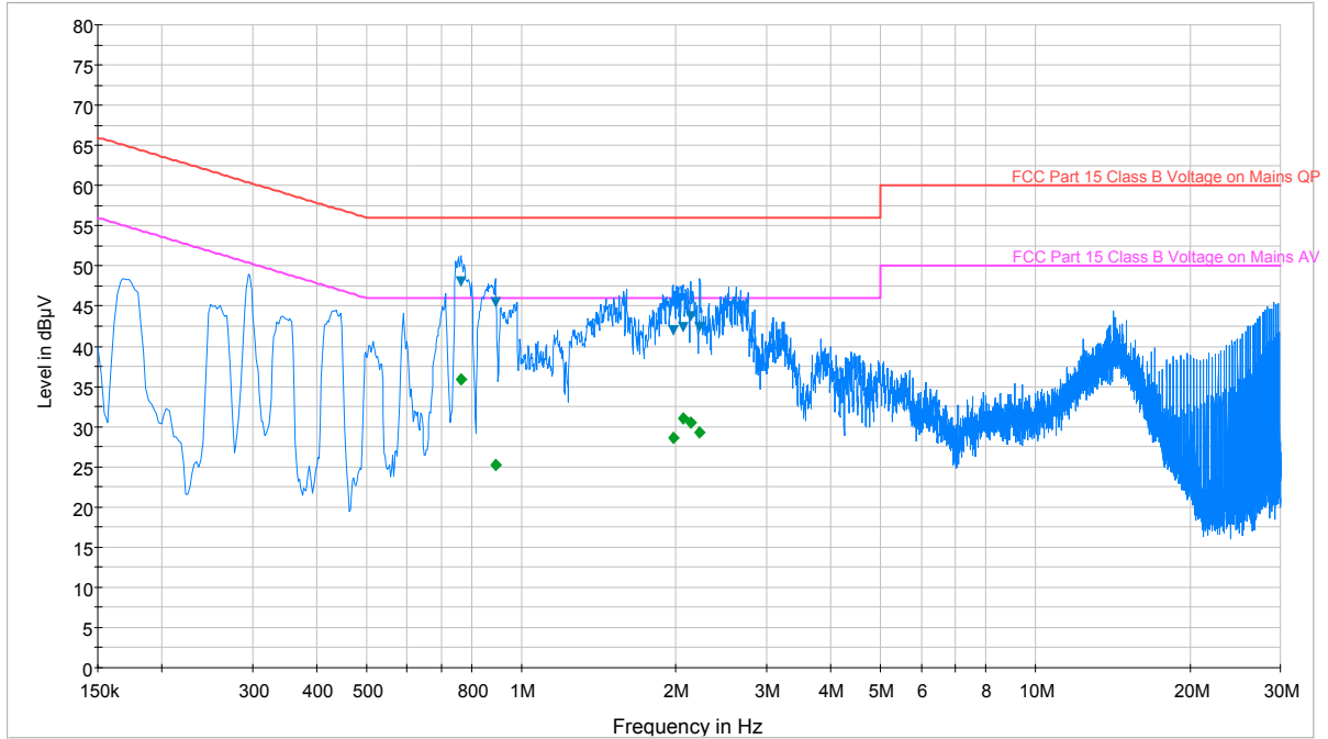
Plot 6-25. Line Conducted Plot with Bluetooth LE (N w/ WCP)
