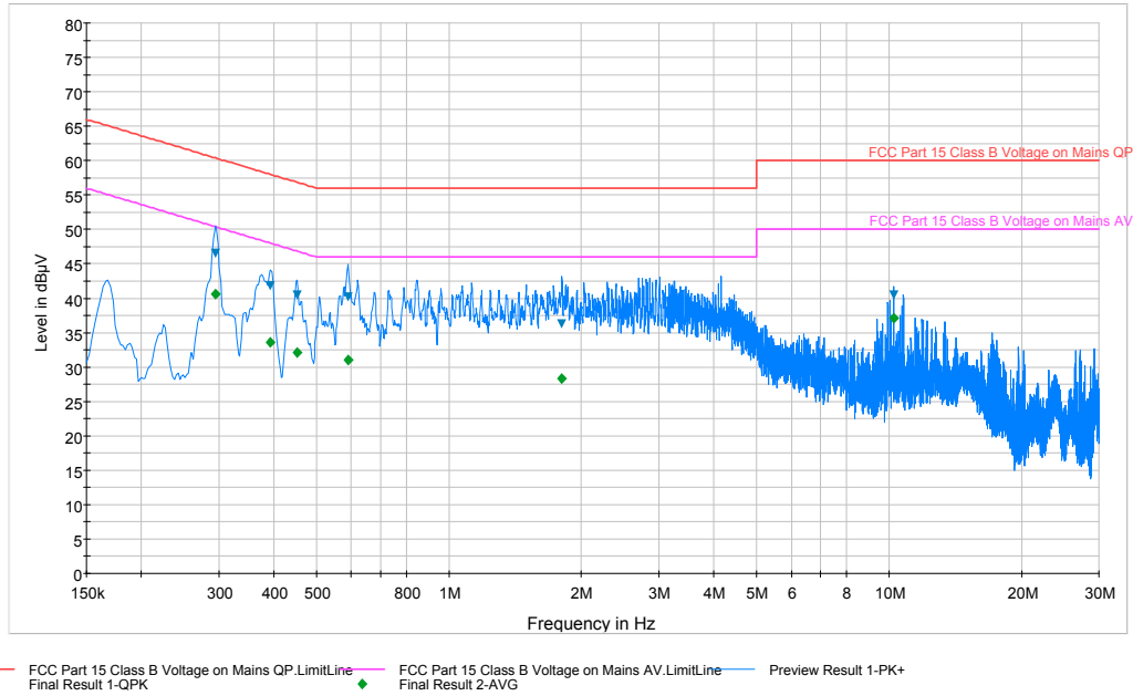
Plot 6-75. Line Conducted Plot with 802.11b (L1)
