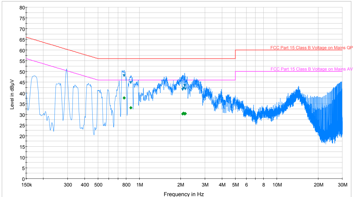
Plot 6-80. Line Conducted Plot with 802.11b (N w/ WCP)
