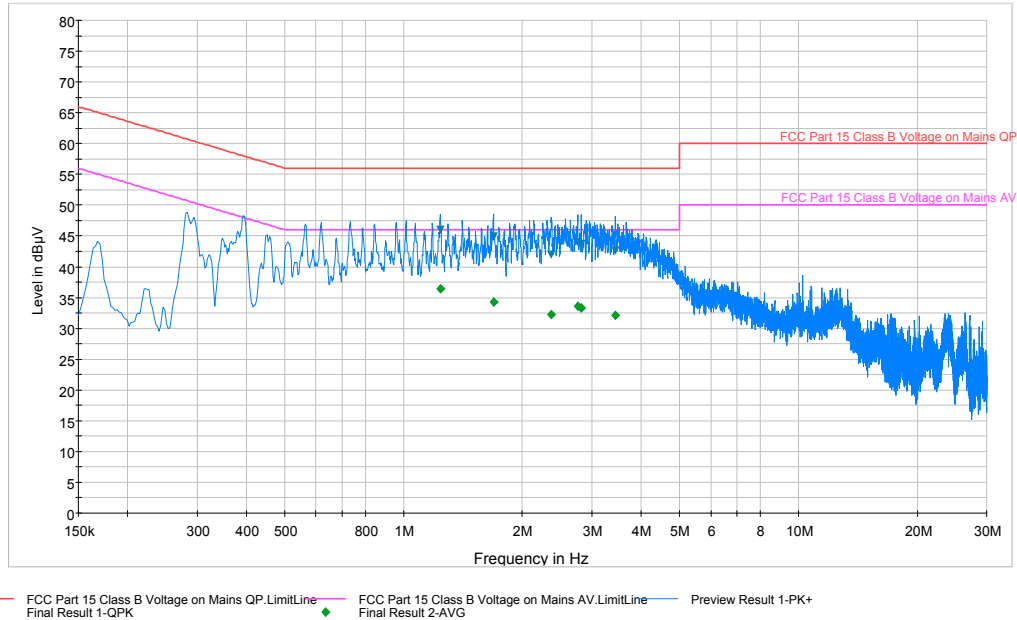
Plot 6-76. Line Conducted Plot with 802.11b (N)
