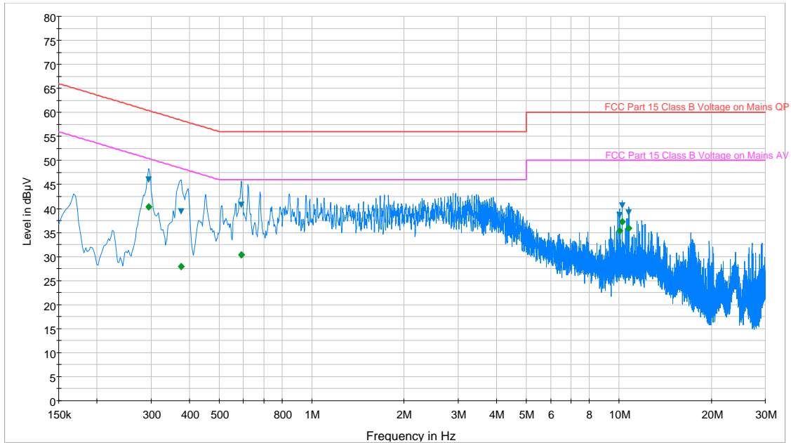
Plot 6-28. Line Conducted Plot with 802.11a UNII Band 1 (L1)
