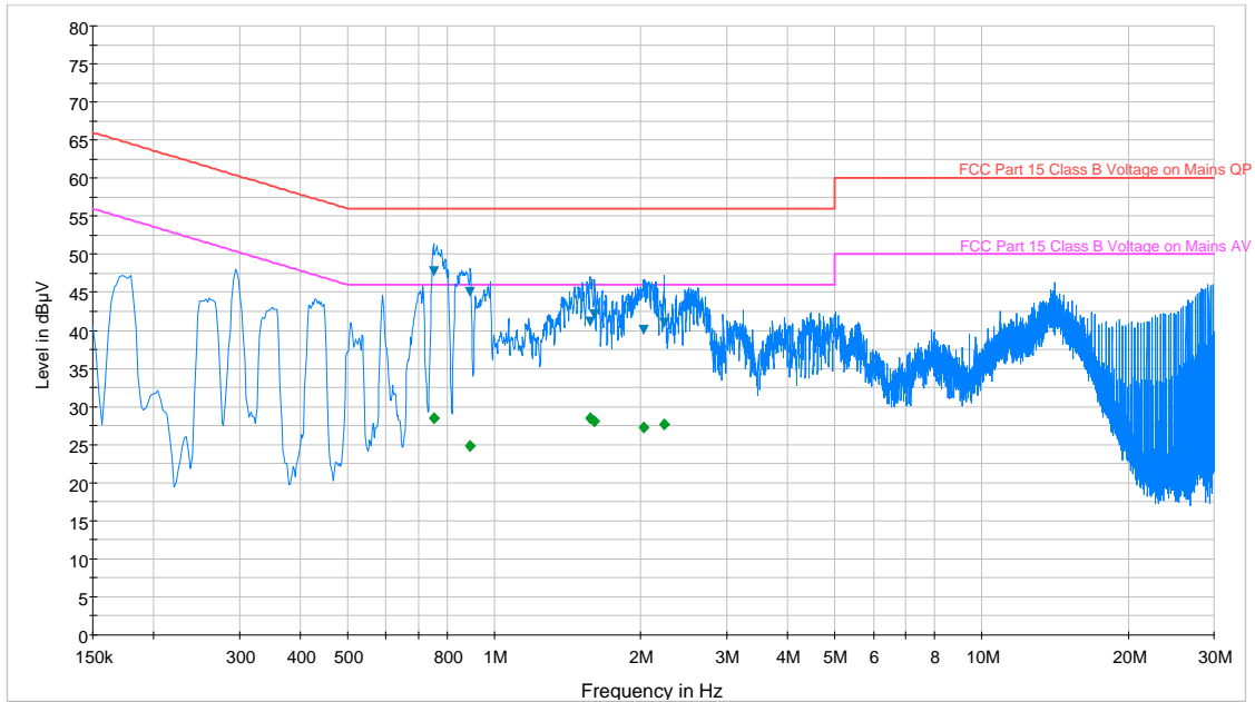
Plot 6-31. Line Conducted Plot with 802.11a UNII Band 1 (N w/ WCP)
