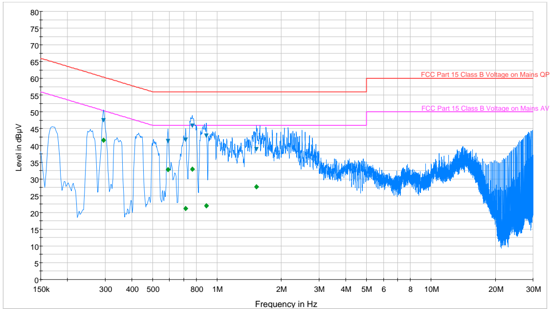
Plot 6-30. Line Conducted Plot with 802.11a UNII Band 1 (L1 w/ WCP)
