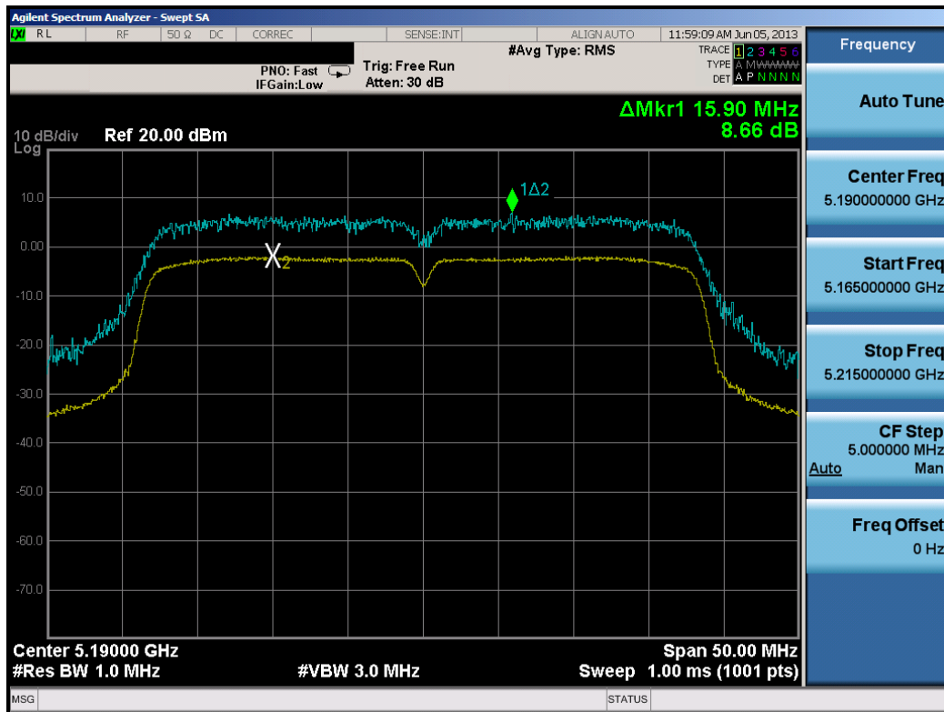
Plot 6-19. Peak Excursion Ratio Plot (40MHz BW 802.11n)
