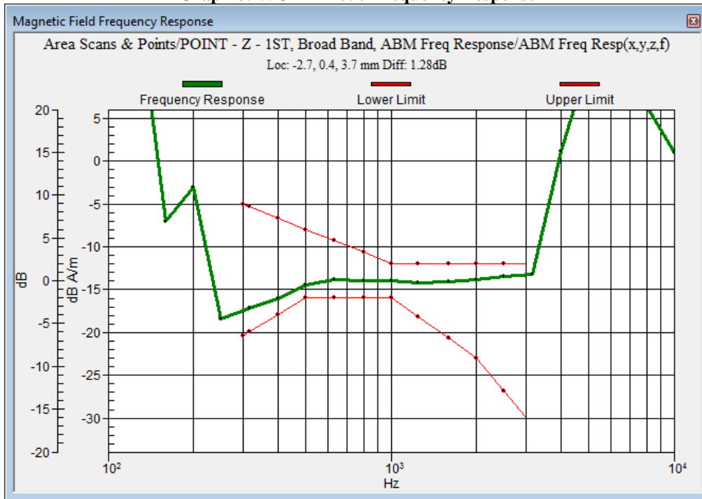
Graph 6: WCDMA 850 Frequency Response
