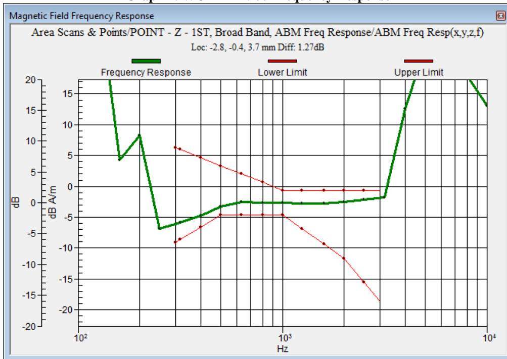
Graph 7: WCDMA 1900 Frequency Response
