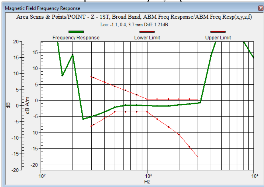
Graph 5: GSM 1900 Frequency Response
