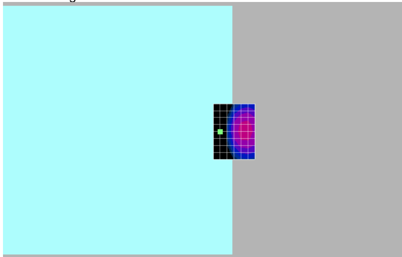
Y-Radial Signal Scan
