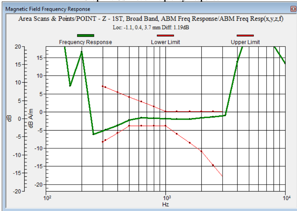
Graph 4: GSM 850 Frequency Response
