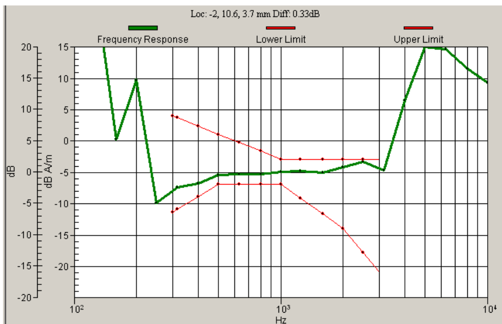
Graph 3: CDMA 1900 Frequency Response
