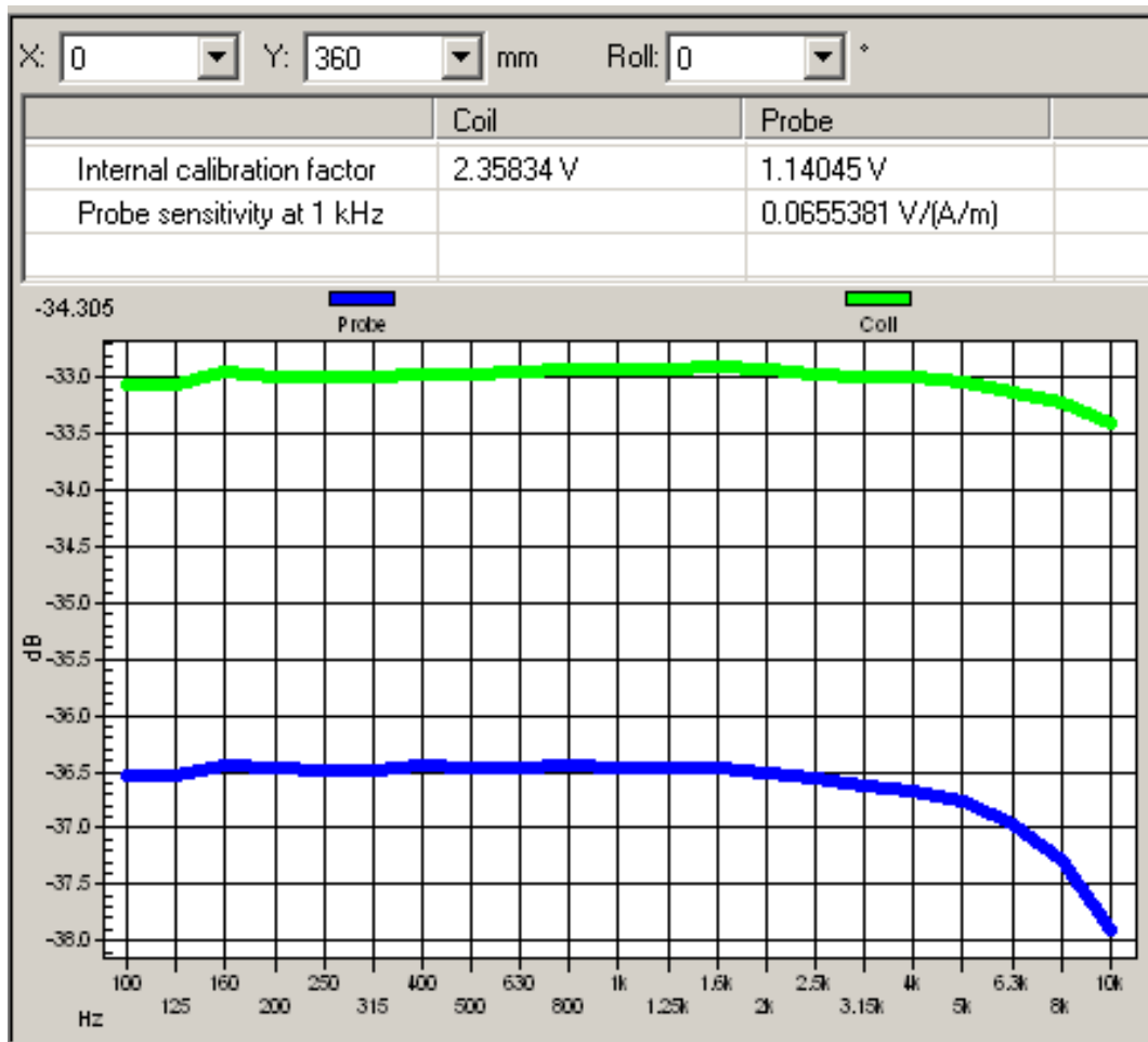
Graph 1: Frequency Response measured in AMCC
