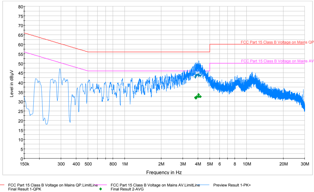
Plot 6-82. Line Conducted Plot with 802.11b (N)
