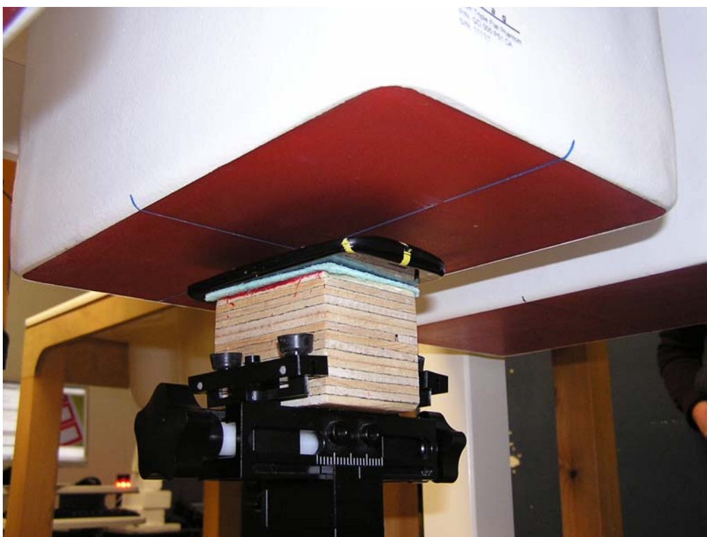
Figure 7: Mobile Hotspot Position, Back of Phone facing Phantom (10 mm separation)
