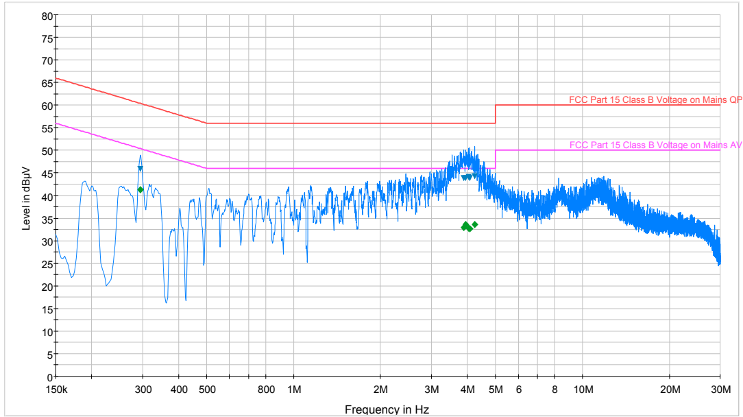
Plot 6-45. Line-Conducted Test Plot (N)
