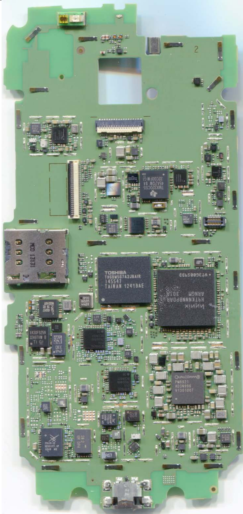
Photograph 9-3: Front side view of the device's PC Board, Shields Removed.
