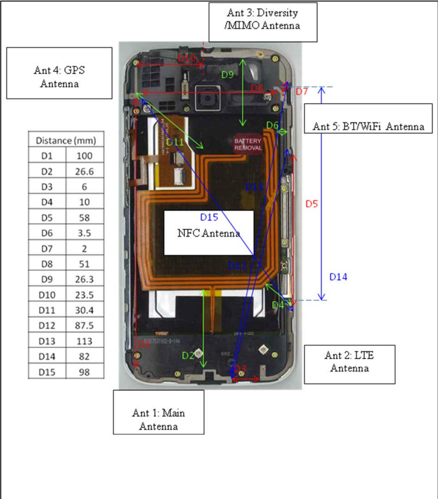
Photograph 9-6: Further Antenna Locations and Spacings Details.
