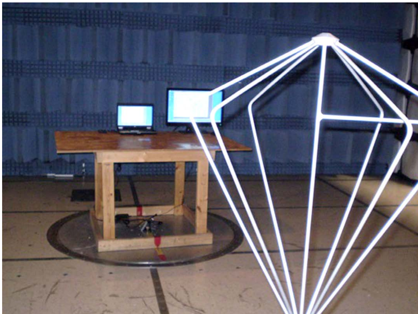
Figure 7B2-1: Spurious Radiations (Part 15 Computing Device).
