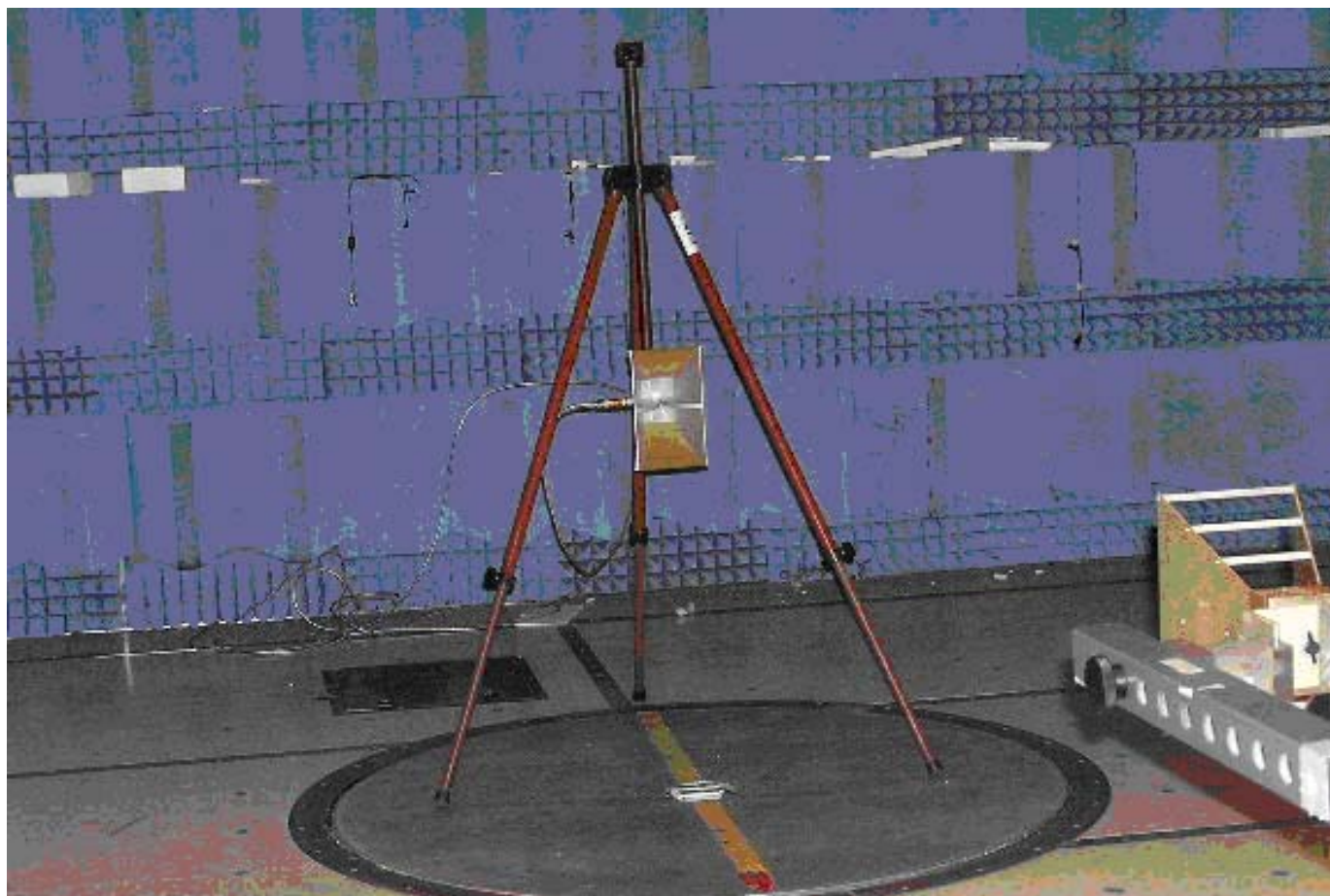
Figure 7B1-2: Antenna - Substitution.
