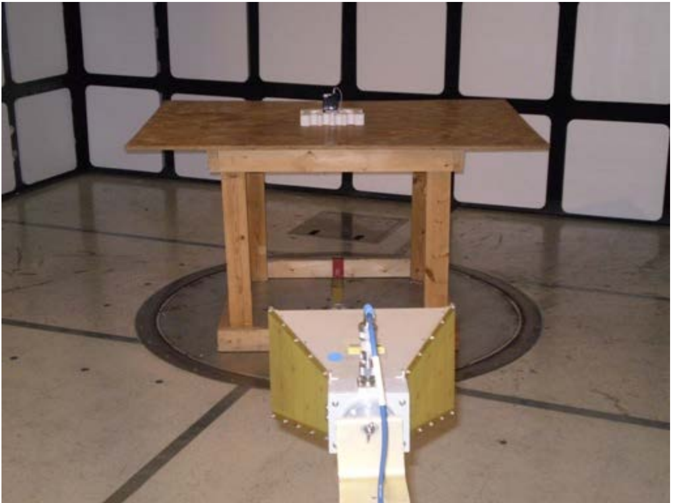
Figure 7B1-1: TX Radiated Emissions Configuration.
