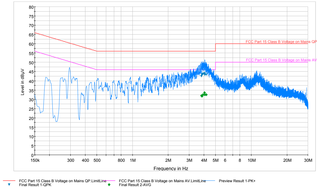
Plot 6-82. Line Conducted Plot with 802.11b (N)
