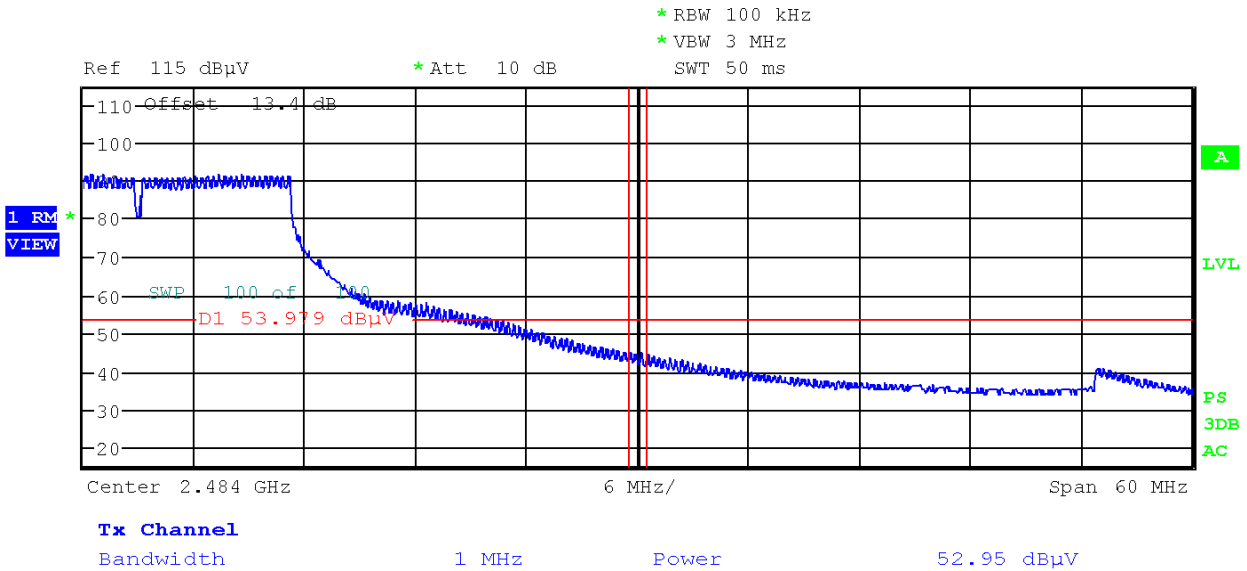
Plot 6-77. Radiated Restricted Upper Band Edge Measurement (Average)
