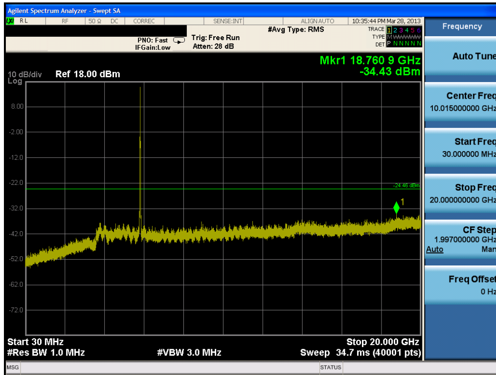
Plot 6-65. Conducted Spurious Plot (802.11a – Ch. 165)
