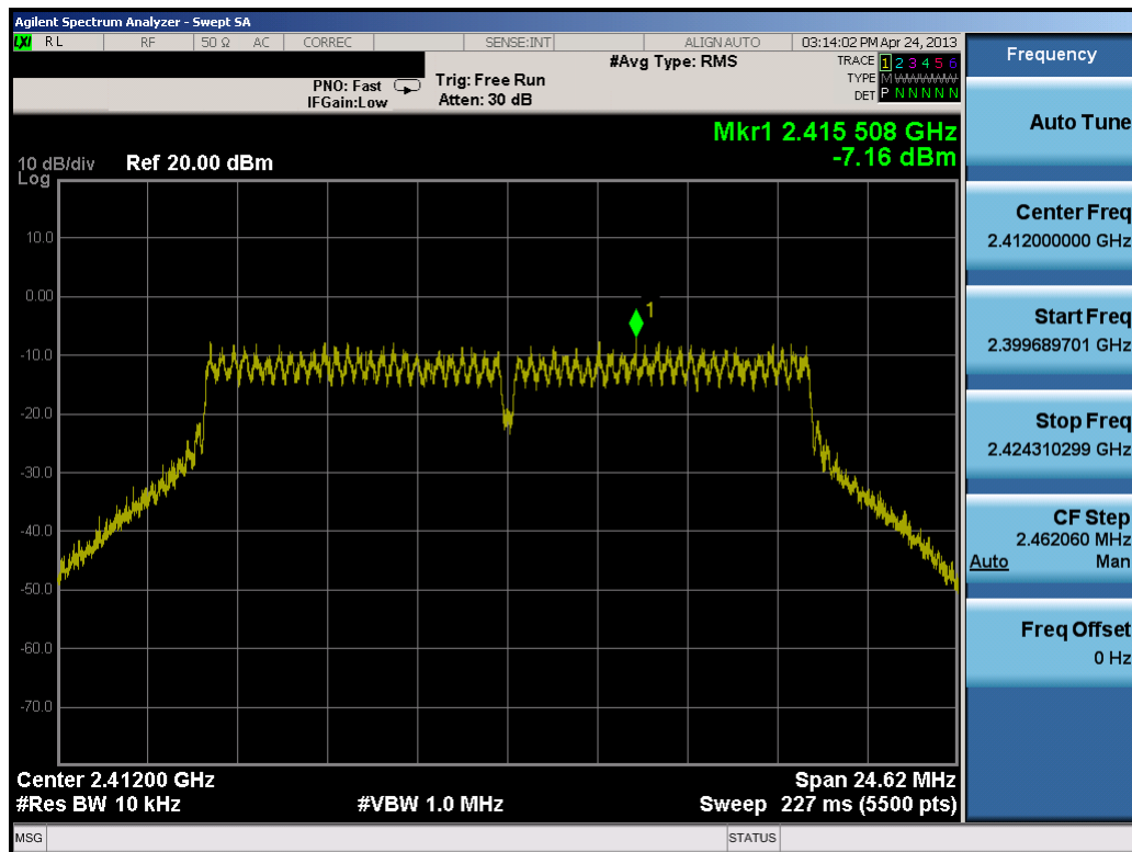
Plot 6-24. Power Spectral Density Plot (802.11g – Ch. 1)
