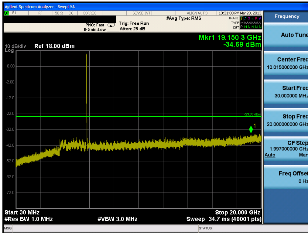
Plot 6-63. Conducted Spurious Plot (802.11a – Ch. 157)
