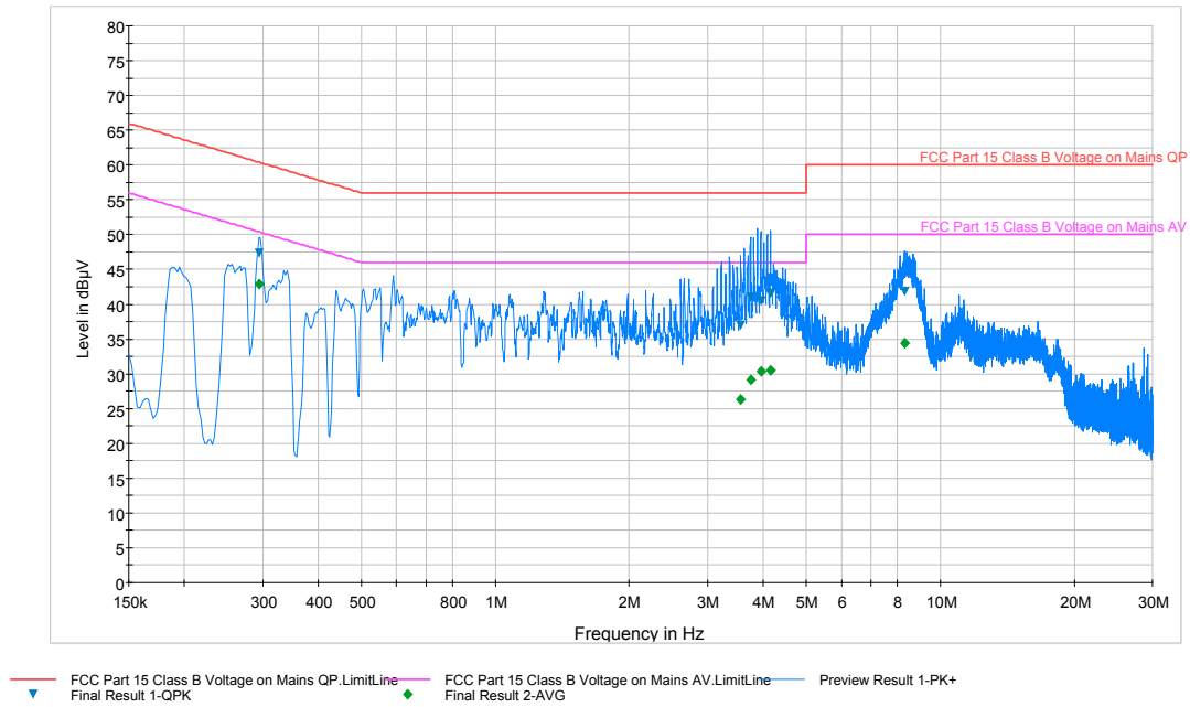
Plot 6-83. Line Conducted Plot with 802.11a (L1)
