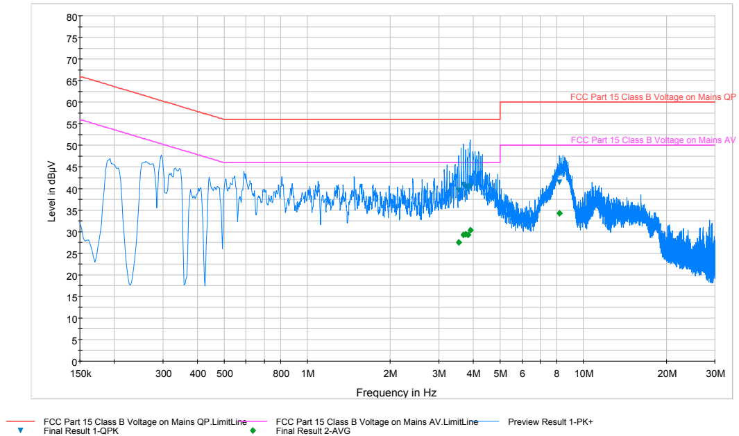
Plot 6-81. Line Conducted Plot with 802.11b (L1)
