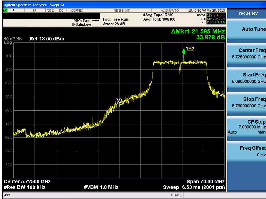
Plot 6-49. Band Edge Plot (20MHz BW 802.11n (5.8GHz) – Ch. 149)
