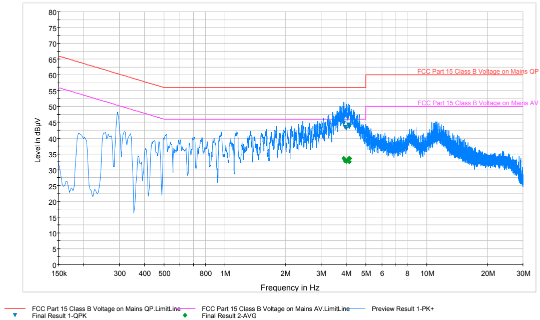
Plot 6-84. Line Conducted Plot with 802.11a (N)
