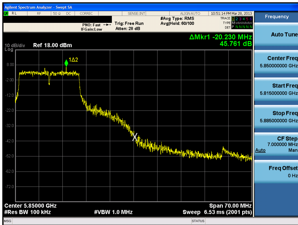
Plot 6-50. Band Edge Plot (20MHz BW 802.11n (5.8GHz) – Ch. 165)
