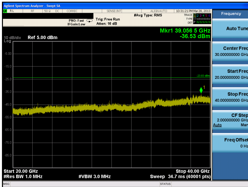
Plot 6-64. Conducted Spurious Plot (802.11a – Ch. 157)
