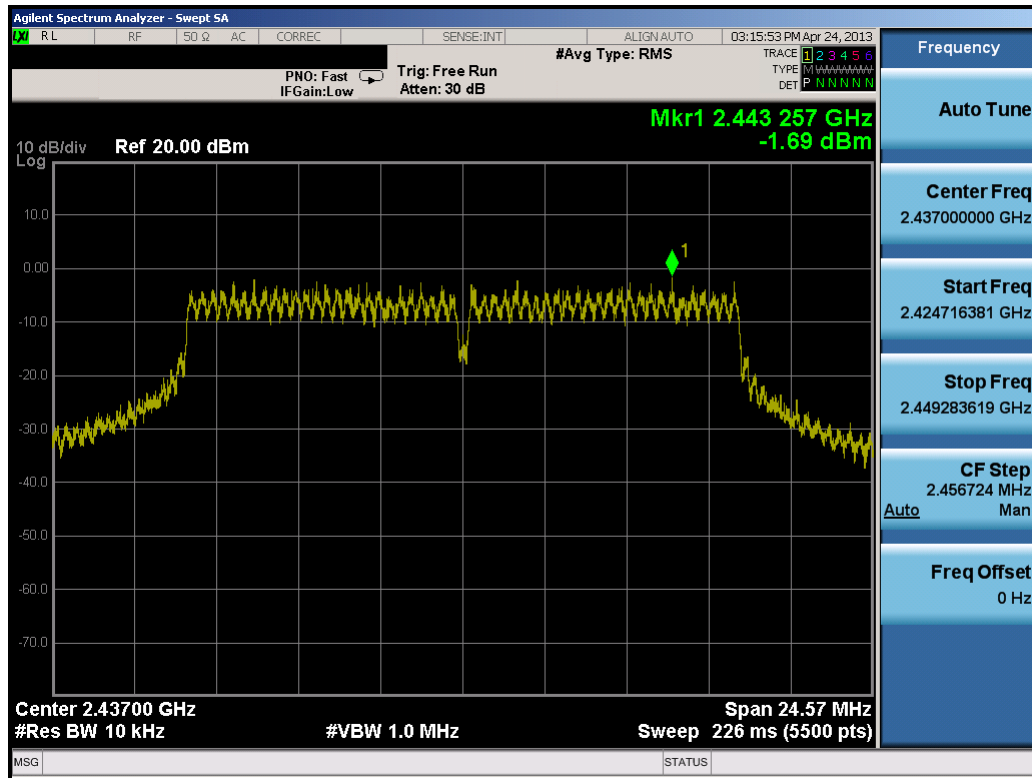
Plot 6-25. Power Spectral Density Plot (802.11g – Ch. 6)
