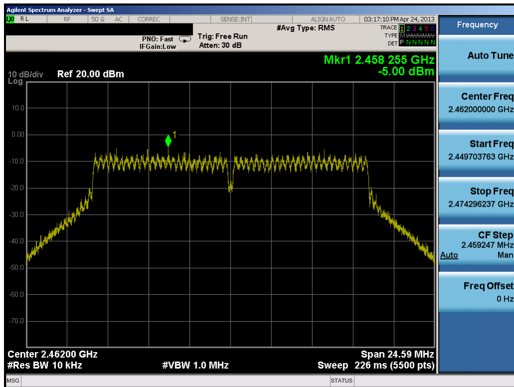
Plot 6-26. Power Spectral Density Plot (802.11g – Ch. 11)
