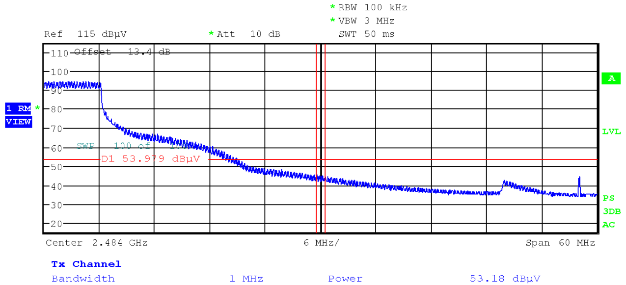
Plot 6-75. Radiated Restricted Upper Band Edge Measurement (Average)
