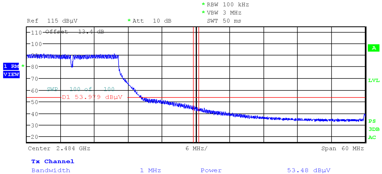
Plot 6-79. Radiated Restricted Upper Band Edge Measurement (Average)
