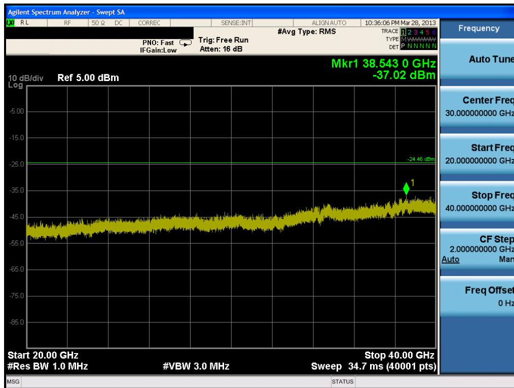
Plot 6-66. Conducted Spurious Plot (802.11a – Ch. 165)
