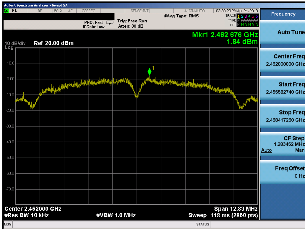
Plot 6-23. Power Spectral Density Plot (802.11b – Ch. 11)
