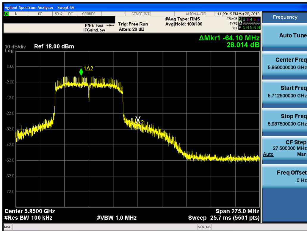
Plot 6-54. Band Edge Plot (80MHz BW 802.11ac (5.8GHz) – Ch. 155)
