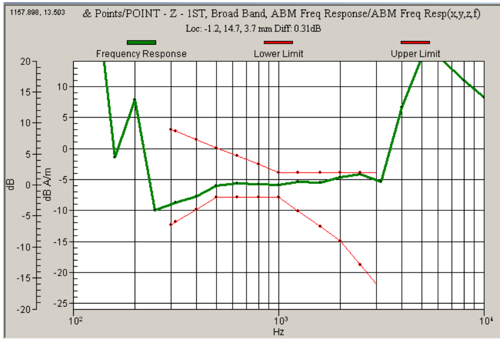
Graph 2: CDMA BC10 Frequency Response
