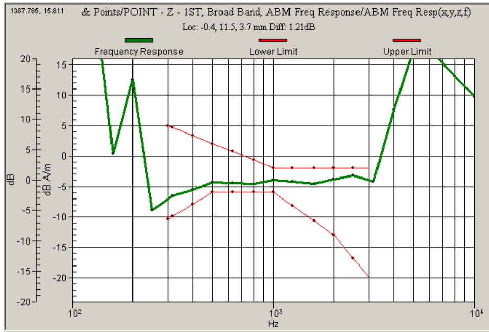
Graph 3: CDMA 1900 Frequency Response
