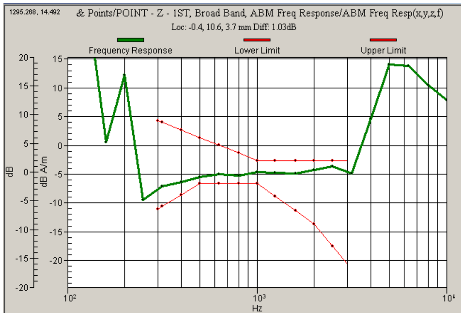
Graph 3: CDMA 800 Frequency Response
