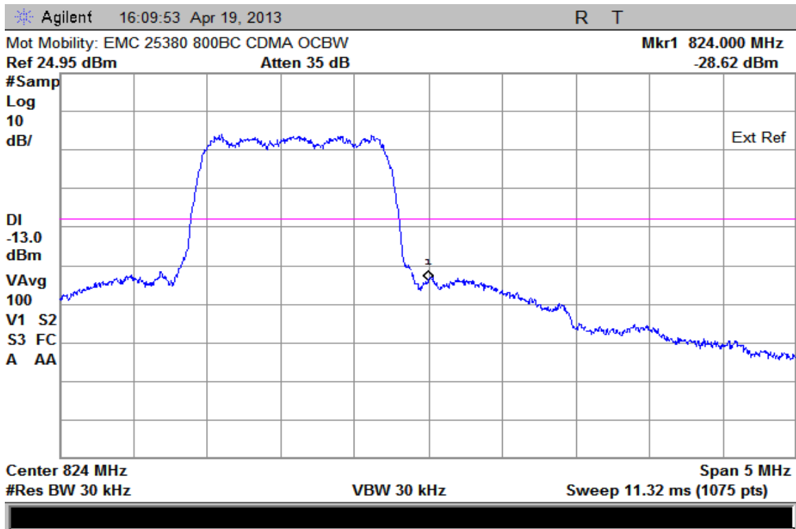
CDMA Band Class 10 – Upper Band Edge – Channel 684 (823.1 MHz)
