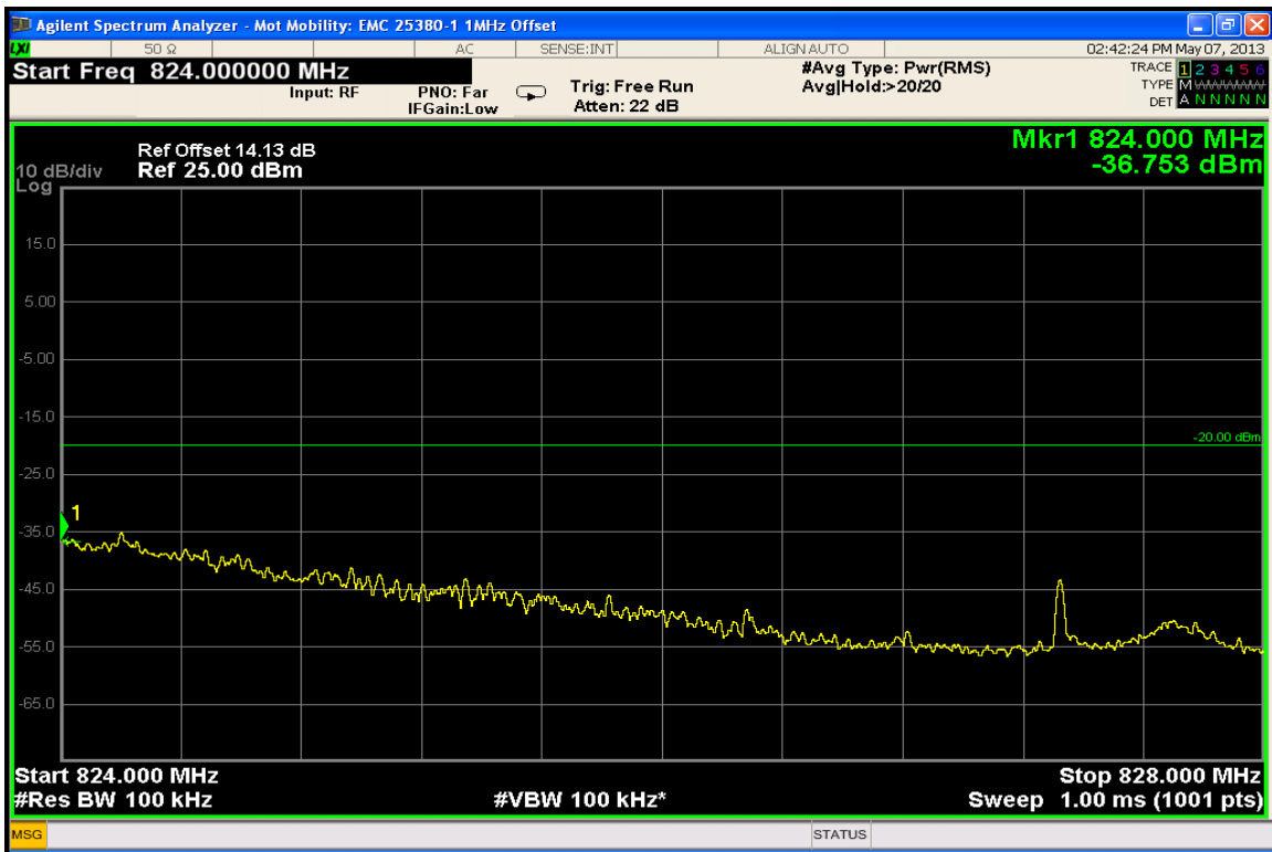
CDMA Band Class 10 Conducted Spurious Emissions (Upper adjacent 1MHz band)
