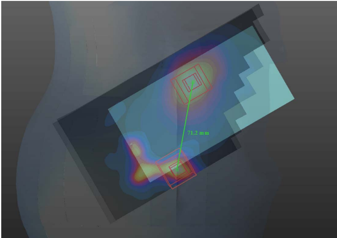
CDMA 1900 Right Head Cheek SAR overlaid with Wi-Fi 5 GHz Right Head Cheek SAR
