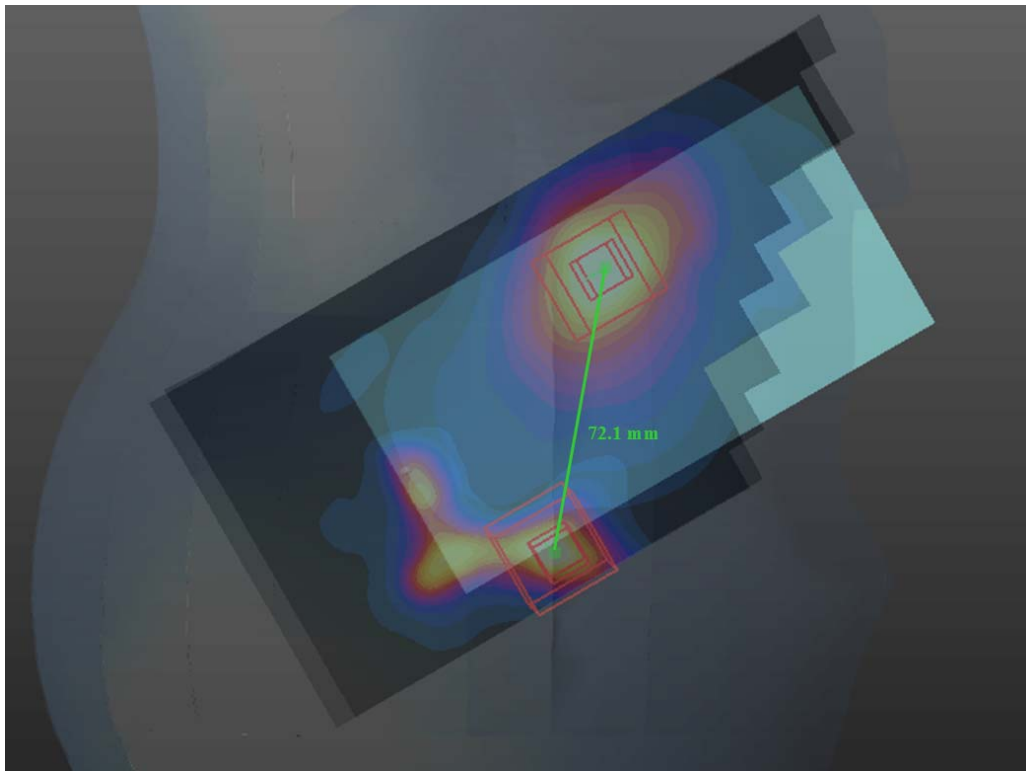
WCDMA 1900 Right Head Cheek SAR overlaid with Wi-Fi 5 GHz Right Head Cheek SAR
