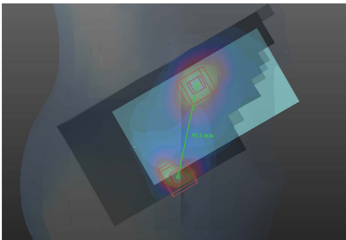
CDMA 1900 Right Head Cheek SAR overlaid with Wi-Fi 2.4 GHz Right Head Cheek SAR
