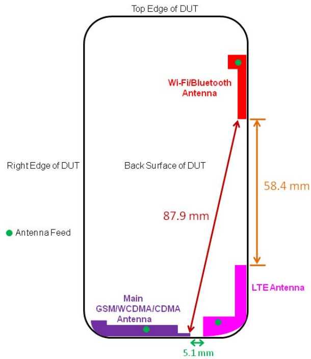
Figure 2: Antenna Locations and Separation Distances
