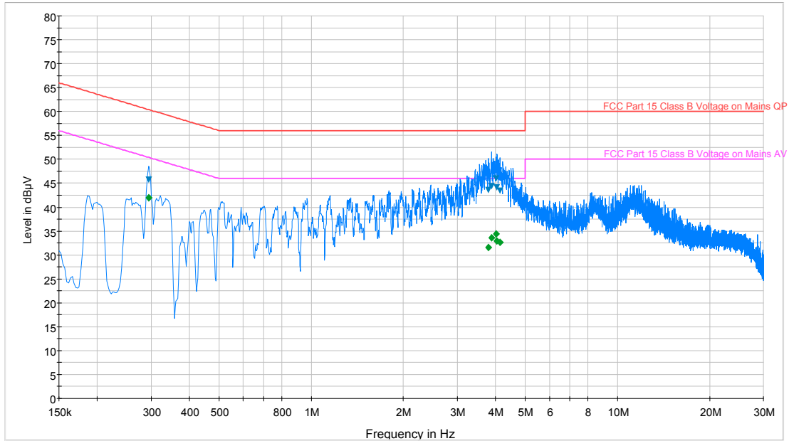
Plot 6-18. Line Conducted Plot with Bluetooth LE (N)
