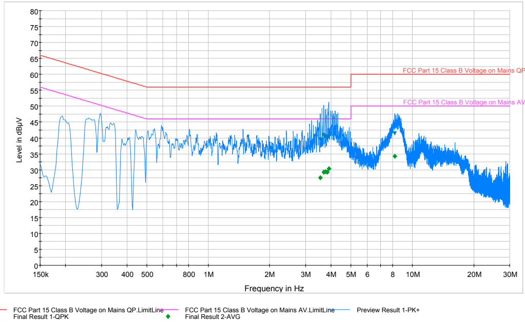
Plot 6-81. Line Conducted Plot with 802.11b (L1)
