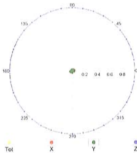
f=600 MHz, TEM, 90^\circ
