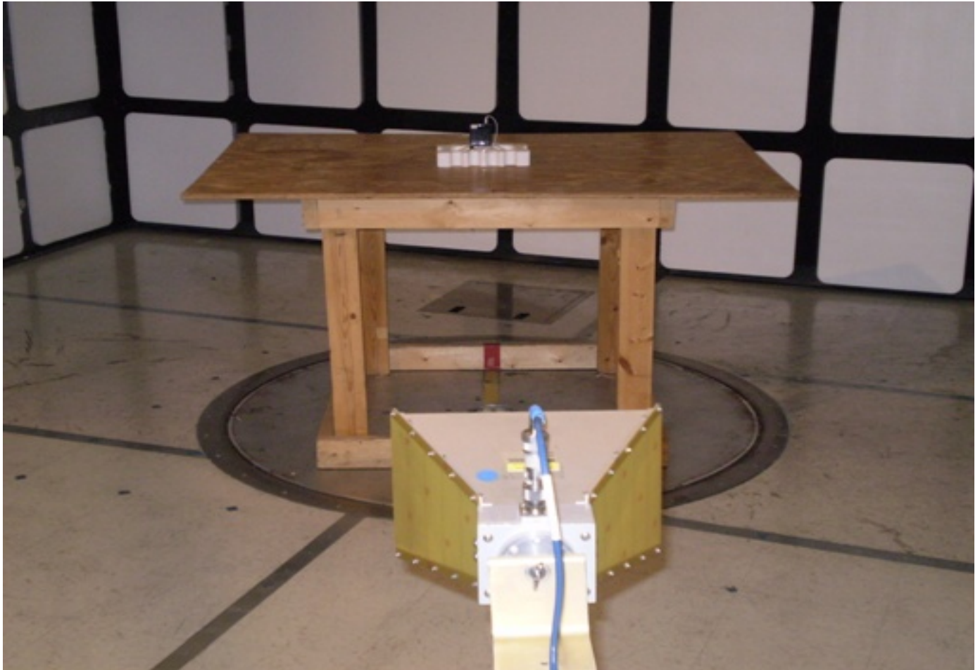
Figure 7B1-1: TX Radiated Configuration.
