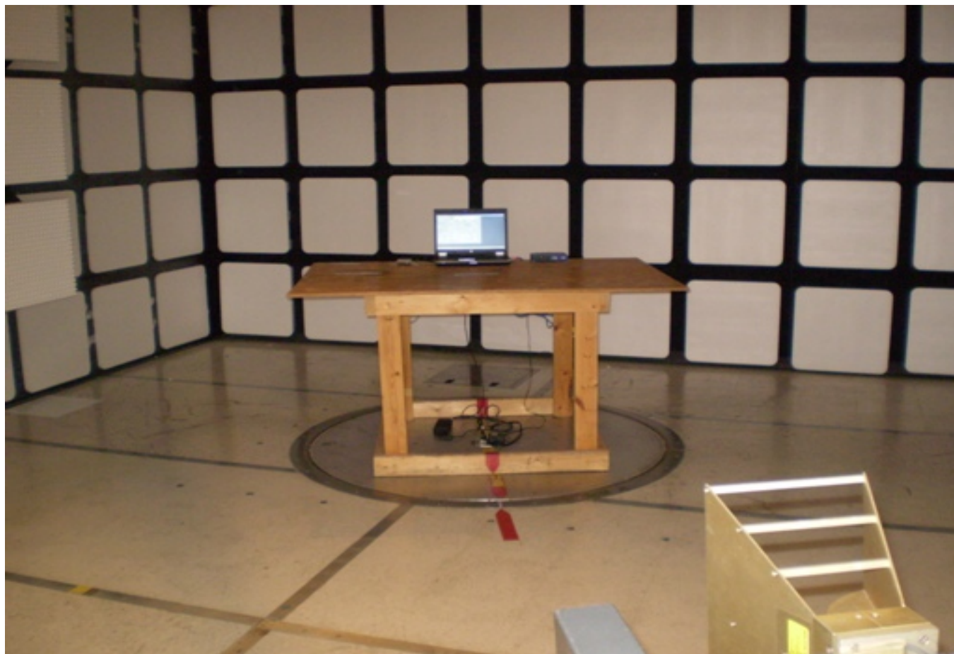
Figure 7B2-1: Spurious Radiations (Part 15 Computing Device).
