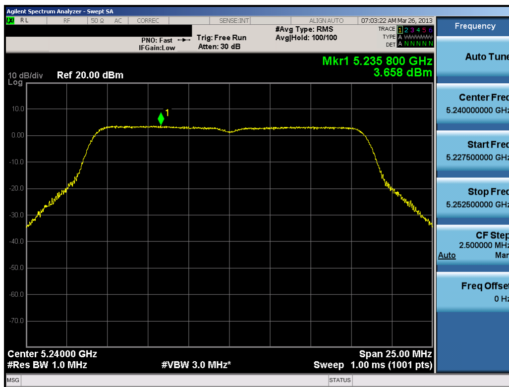
Plot 6-12. Peak Power Spectral Density Plot (802.11a (UNII Band 1) – Ch. 48)
