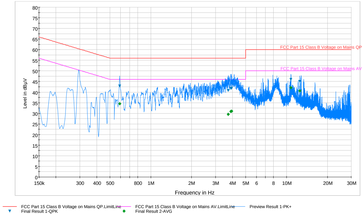
Plot 6-30. Line Conducted Plot with 802.11a UNII Band 1 (N)
