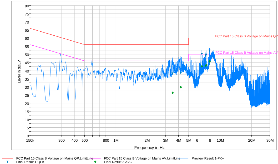
Plot 6-29. Line Conducted Plot with 802.11a UNII Band 1 (L1)
