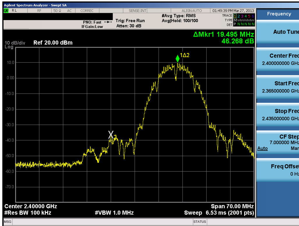
Plot 6-41. Band Edge Plot (802.11b - Ch. 1)
