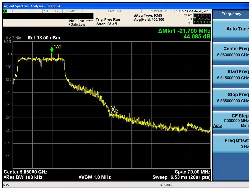
Plot 6-48. Band Edge Plot (802.11a – Ch. 165)
