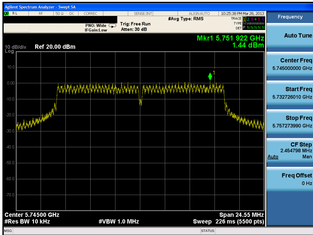
Plot 6-30. Power Spectral Density Plot (802.11a - Ch. 149)
