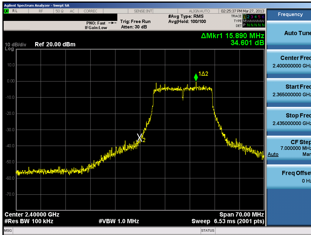
Plot 6-43. Band Edge Plot (802.11g- Ch. 1)
