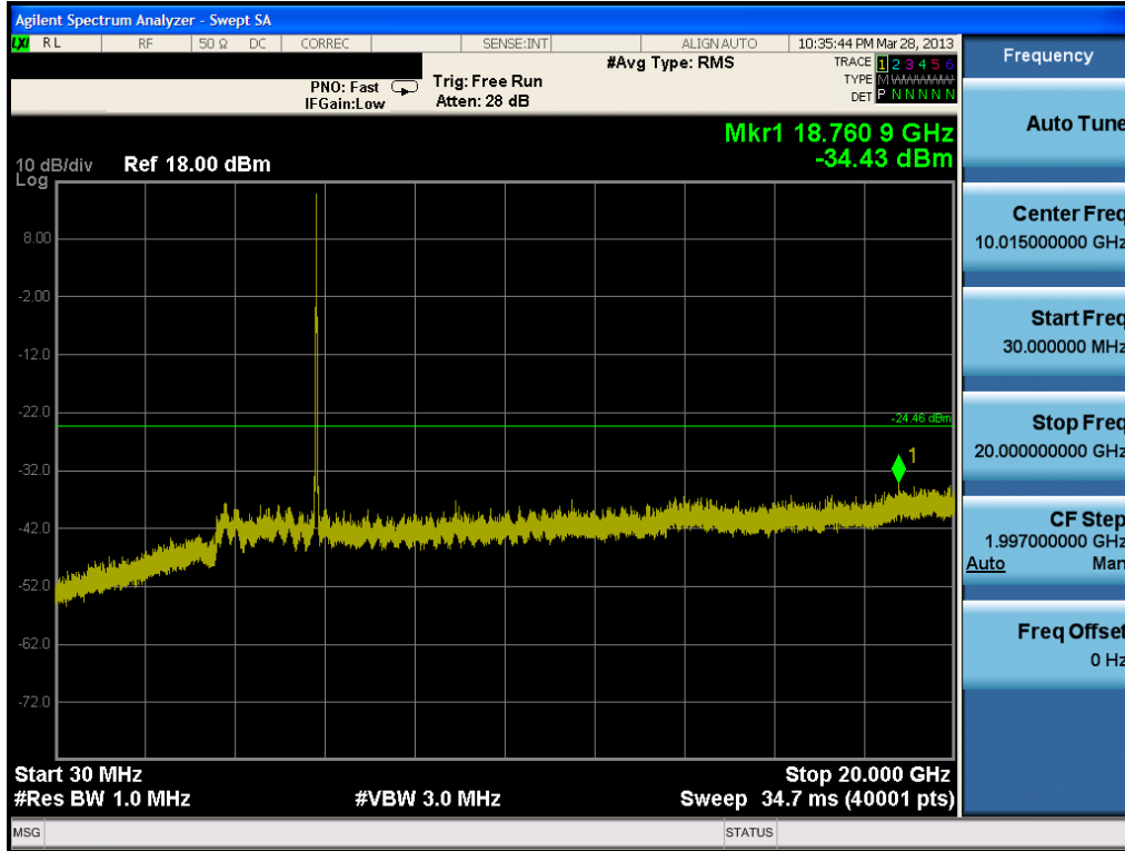
Plot 6-65. Conducted Spurious Plot (802.11a – Ch. 165)
