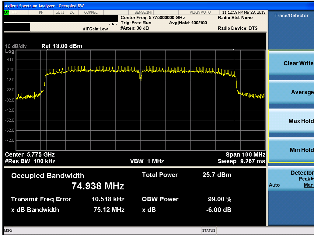
Plot 6-19. 6dB Bandwidth Plot (80MHz BW 802.11ac (5.8GHz) – Ch. 155)
