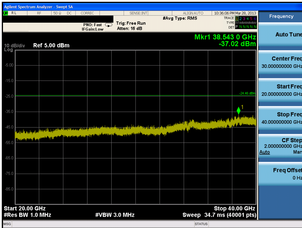
Plot 6-66. Conducted Spurious Plot (802.11a – Ch. 165)
