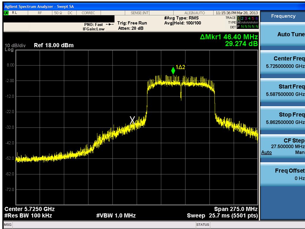
Plot 6-53. Band Edge Plot (80MHz BW 802.11ac (5.8GHz) – Ch. 155)
