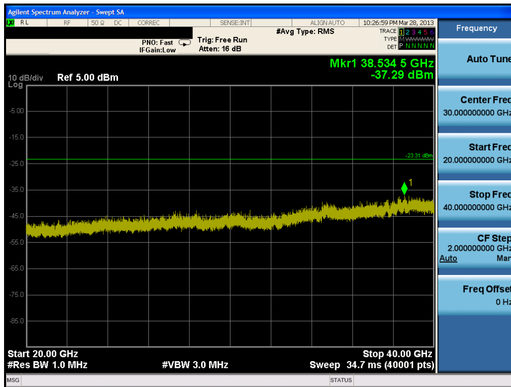
Plot 6-62. Conducted Spurious Plot (802.11a – Ch. 149)
