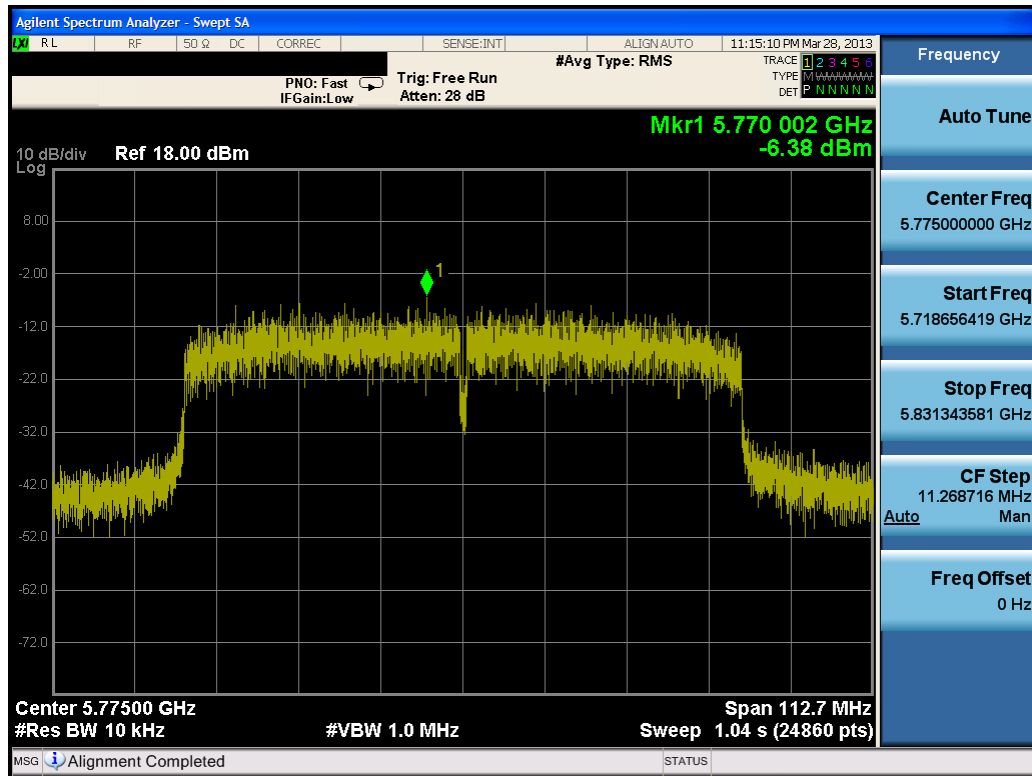
Plot 6-39. Power Spectral Density Plot (80MHz BW 802.11ac (5.8GHz) – Ch. 155)
