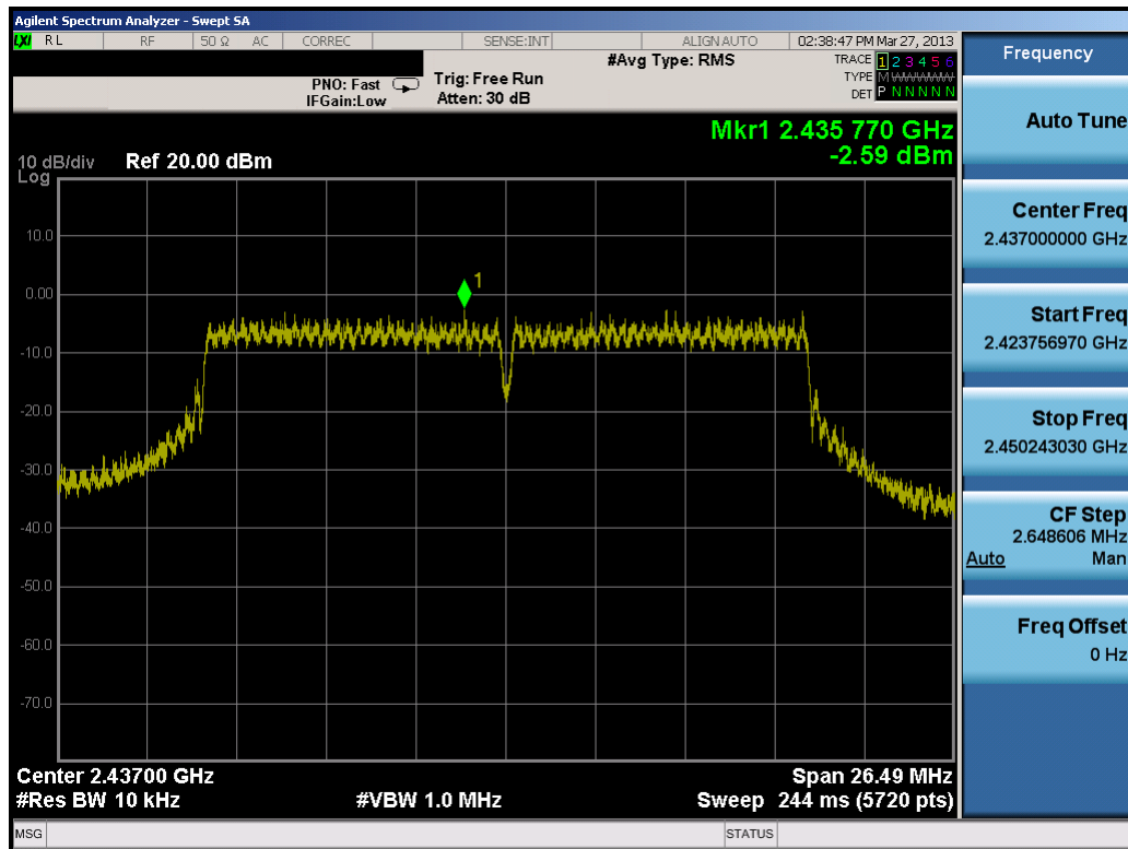
Plot 6-28. Power Spectral Density Plot (802.11n (2.4GHz) – Ch. 6)
