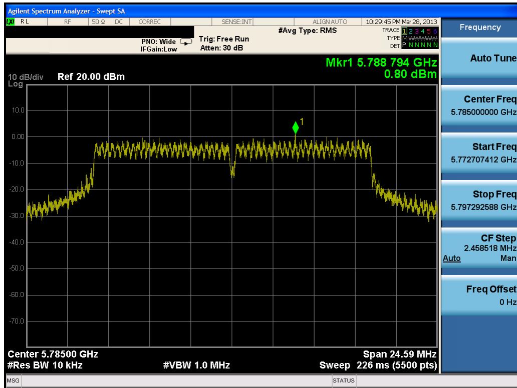
Plot 6-31. Power Spectral Density Plot (802.11a - Ch. 157)
