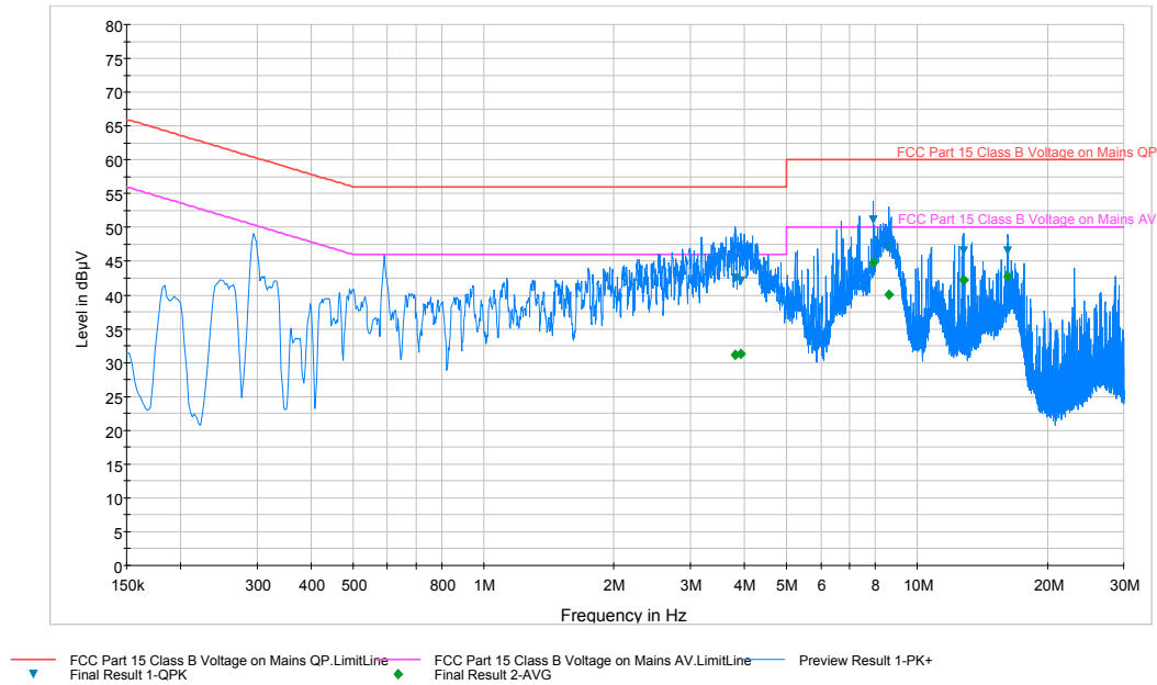
Plot 6-86. Line Conducted Plot with 802.11b (N)
