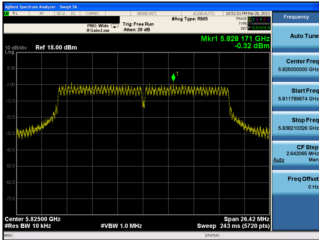
Plot 6-35. Power Spectral Density Plot (20MHz BW 802.11n (5.8GHz) – Ch. 165)
