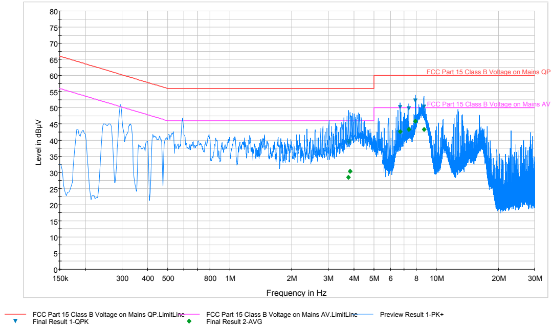
Plot 6-87. Line Conducted Plot with 802.11a (L1)
