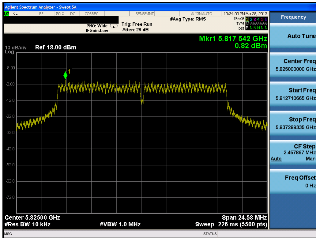
Plot 6-32. Power Spectral Density Plot (802.11a - Ch. 165)
