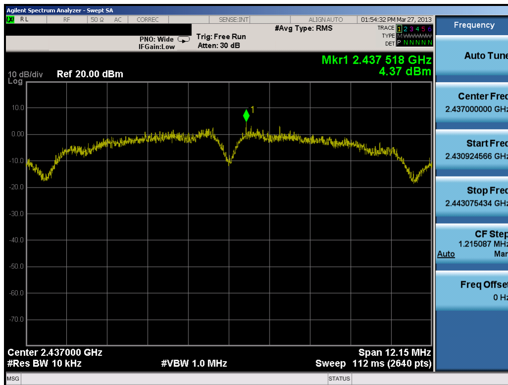
Plot 6-22. Power Spectral Density Plot (802.11b – Ch. 6)
