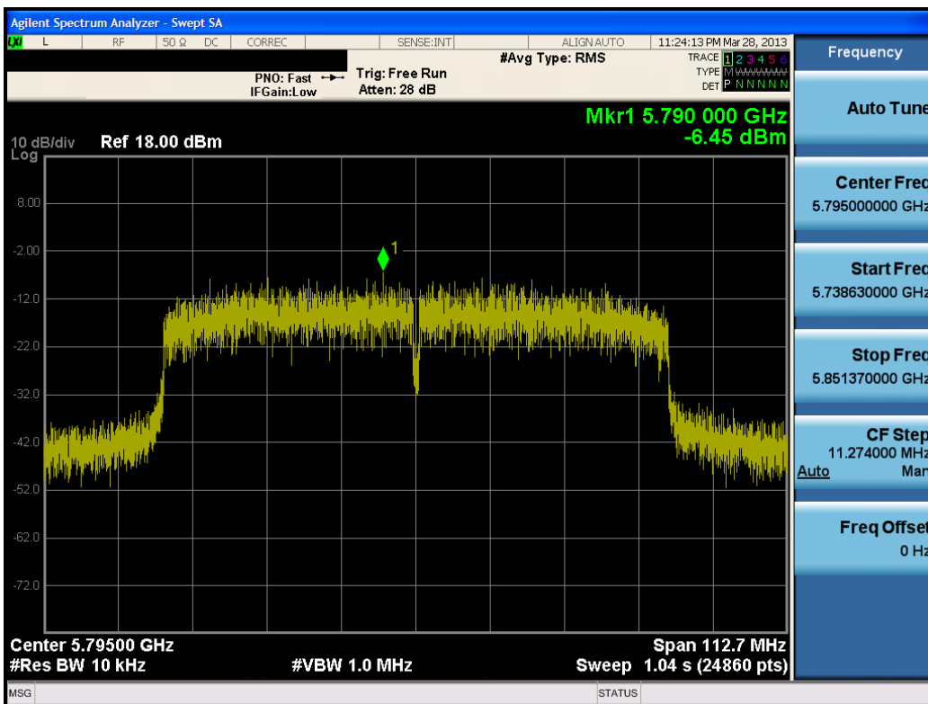
Plot 6-40. Power Spectral Density Plot (80MHz BW 802.11ac (5.8GHz) – Ch. 159)
