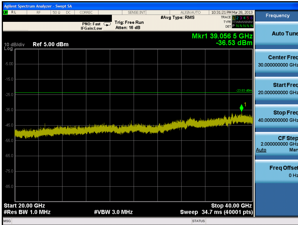
Plot 6-64. Conducted Spurious Plot (802.11a – Ch. 157)
