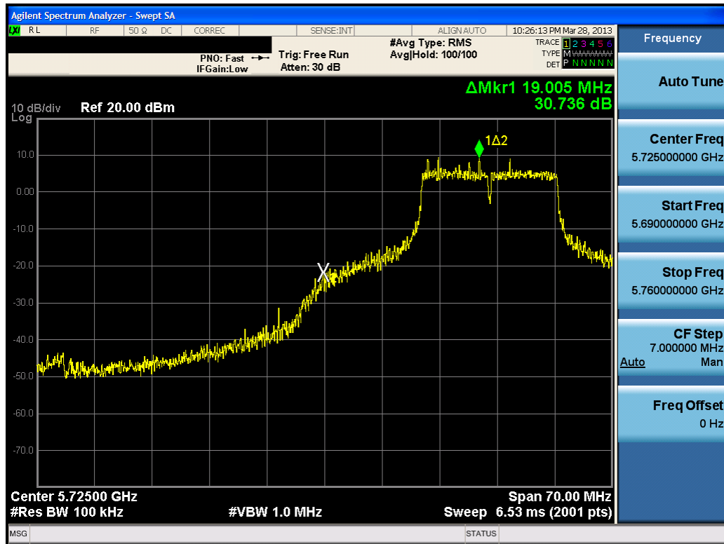
Plot 6-47. Band Edge Plot (802.11a – Ch. 149)
