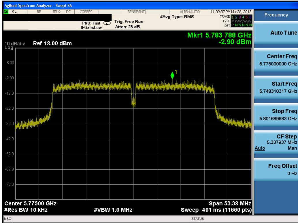
Plot 6-37. Power Spectral Density Plot (40MHz BW 802.11n (5.8GHz) – Ch. 155)
