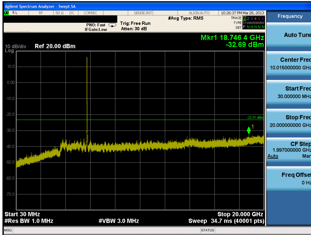
Plot 6-61. Conducted Spurious Plot (802.11a – Ch. 149)
