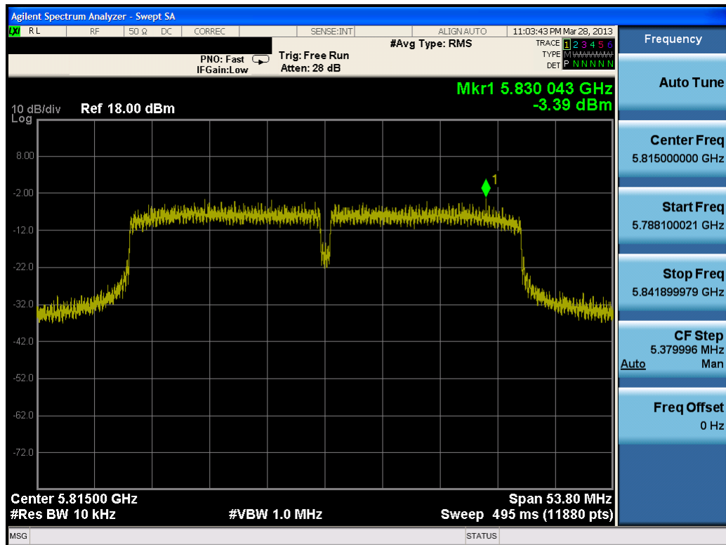
Plot 6-38. Power Spectral Density Plot (40MHz BW 802.11n (5.8GHz) – Ch. 163)
