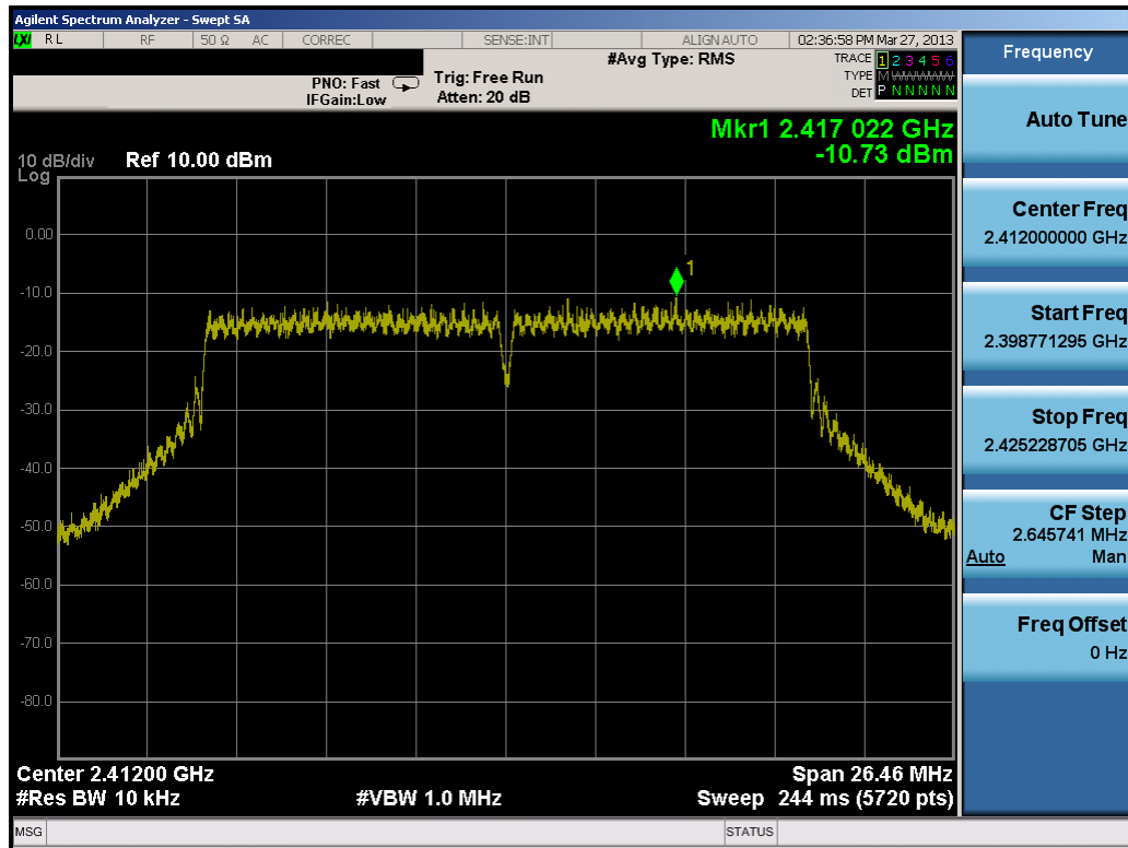
Plot 6-27. Power Spectral Density Plot (802.11n (2.4GHz) – Ch. 1)
