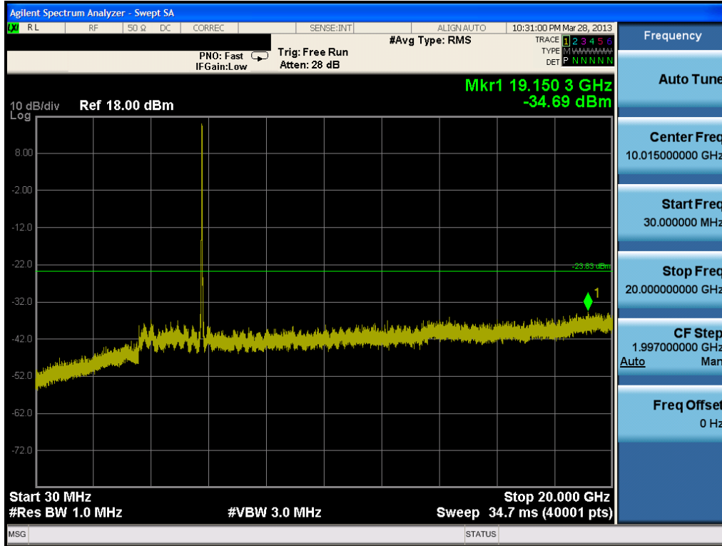
Plot 6-63. Conducted Spurious Plot (802.11a – Ch. 157)
