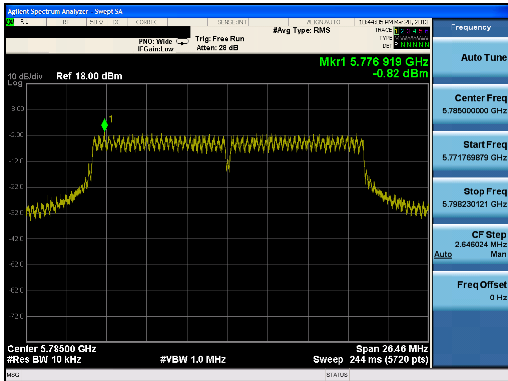
Plot 6-34. Power Spectral Density Plot (20MHz BW 802.11n (5.8GHz) – Ch. 157)
