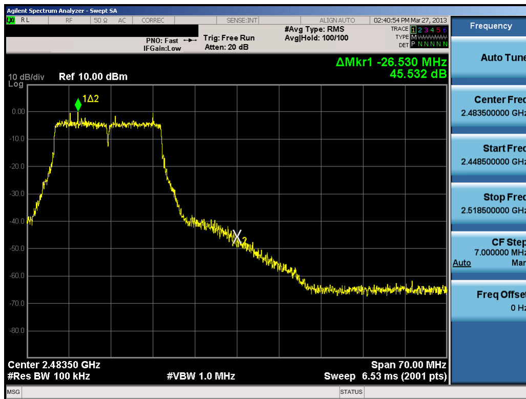
Plot 6-46. Band Edge Plot (802.11n (2.4GHz) – Ch. 11)
