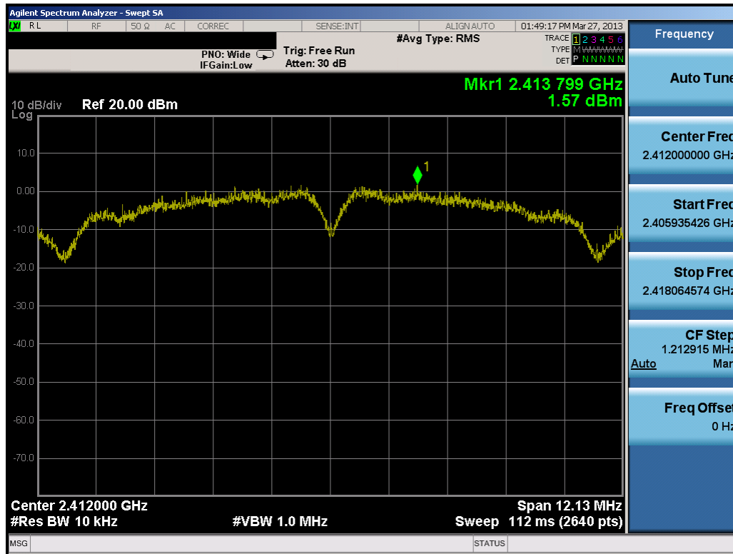
Plot 6-21. Power Spectral Density Plot (802.11b – Ch. 1)
