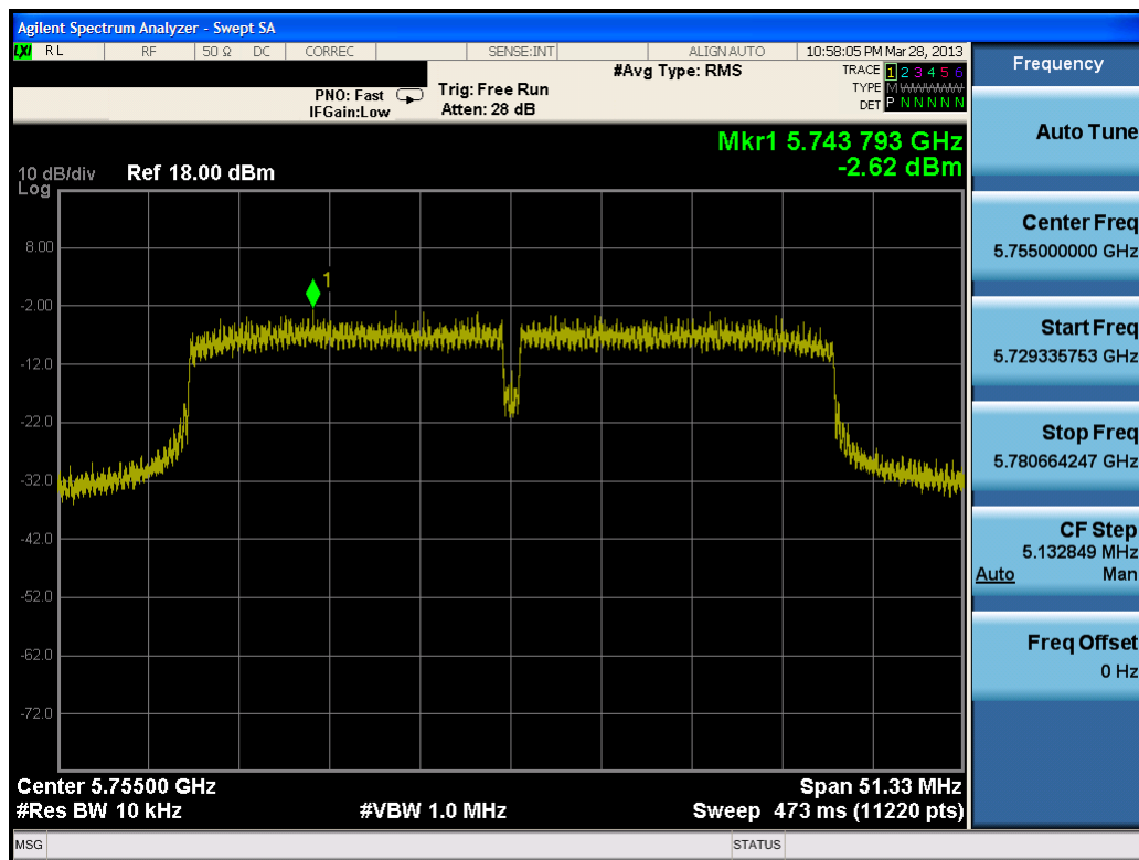
Plot 6-36. Power Spectral Density Plot (40MHz BW 802.11n (5.8GHz) – Ch. 151)
