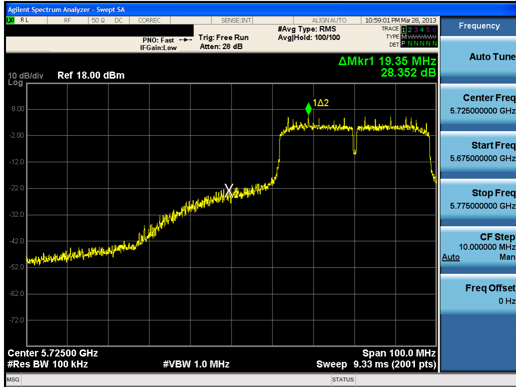
Plot 6-51. Band Edge Plot (40MHz BW 802.11n (5.8GHz) – Ch. 151)
