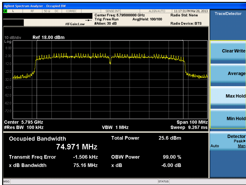
Plot 6-20. 6dB Bandwidth Plot (80MHz BW 802.11ac (5.8GHz) – Ch. 159)
