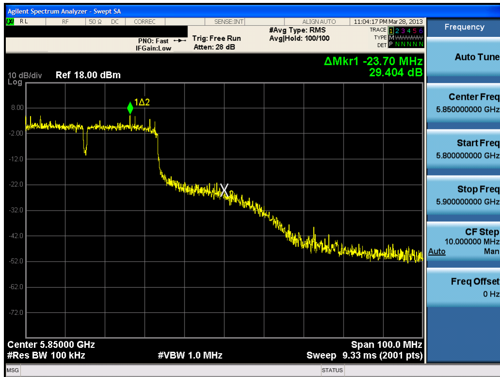
Plot 6-52. Band Edge Plot (40MHz BW 802.11n (5.8GHz) – Ch. 163)
