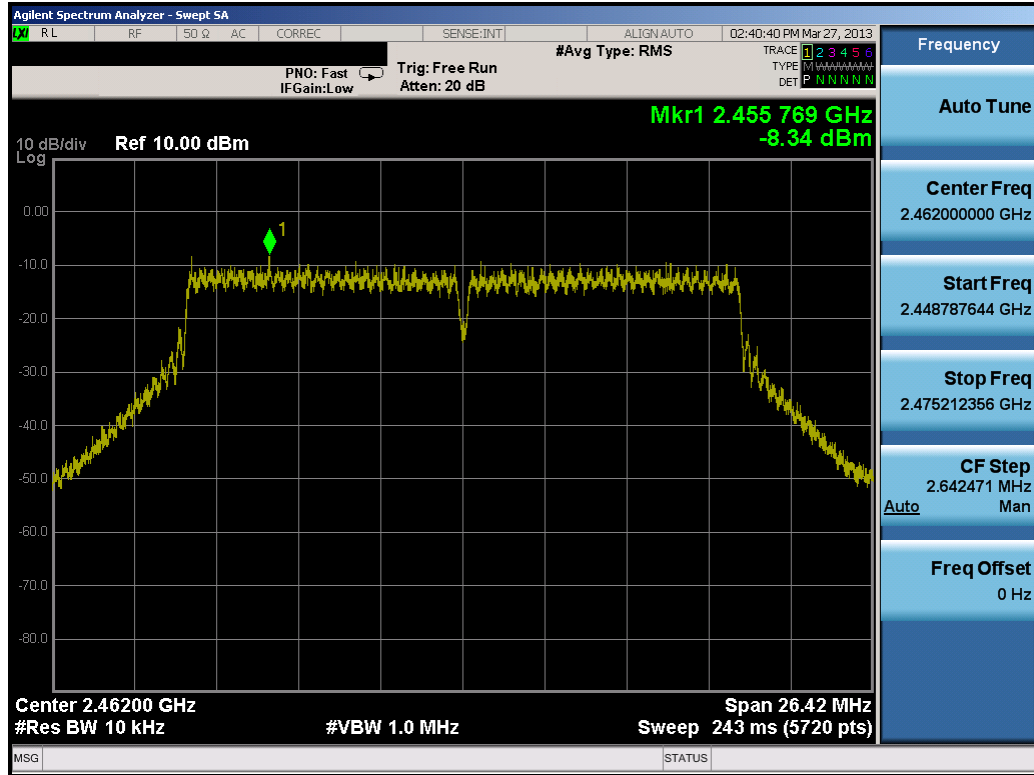
Plot 6-29. Power Spectral Density Plot (802.11n (2.4GHz) – Ch. 11)
