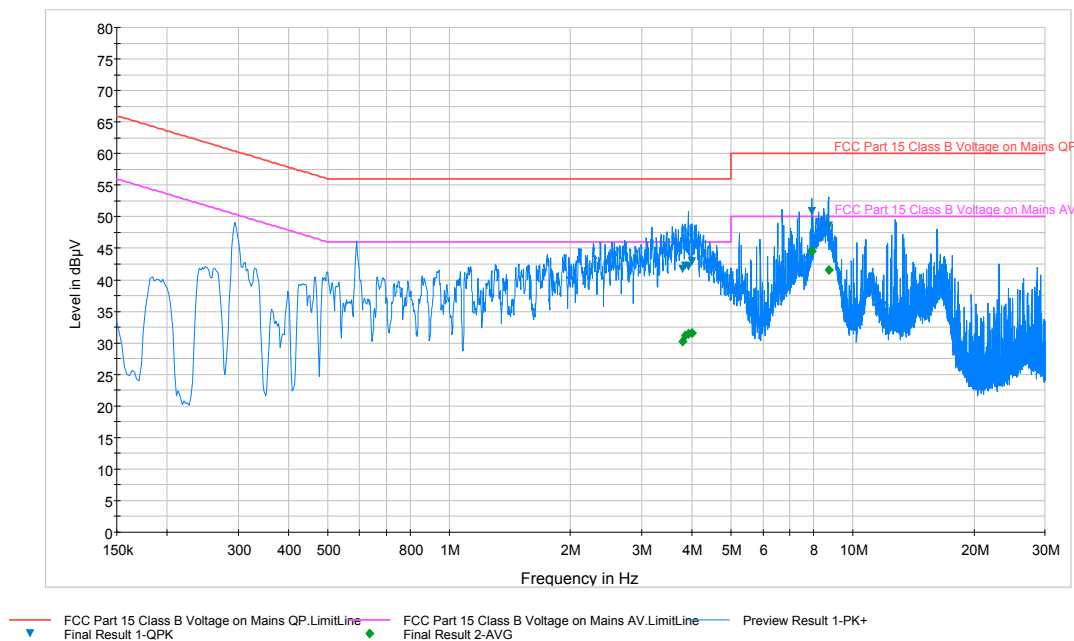
Plot 6-88. Line Conducted Plot with 802.11a (N)
