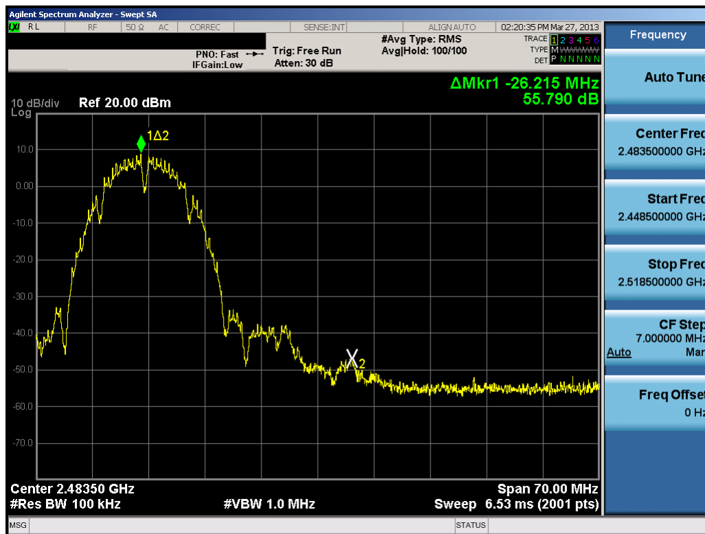
Plot 6-42. Band Edge Plot (802.11b - Ch. 11)
