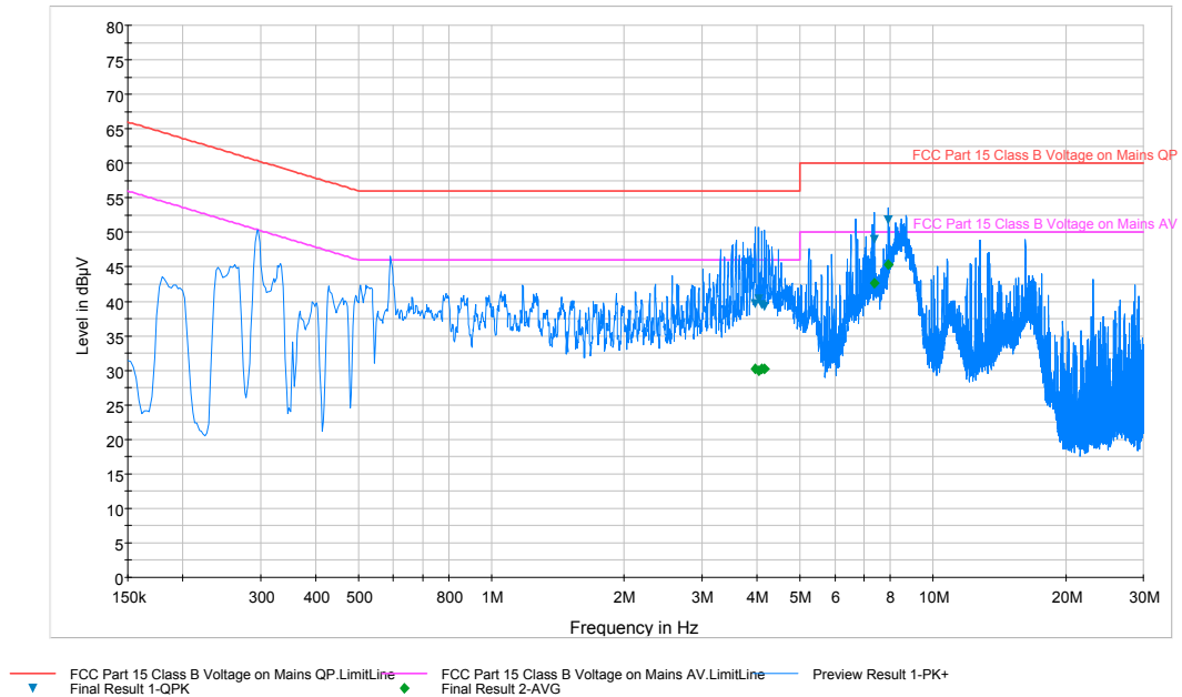
Plot 6-85. Line Conducted Plot with 802.11b (L1)
