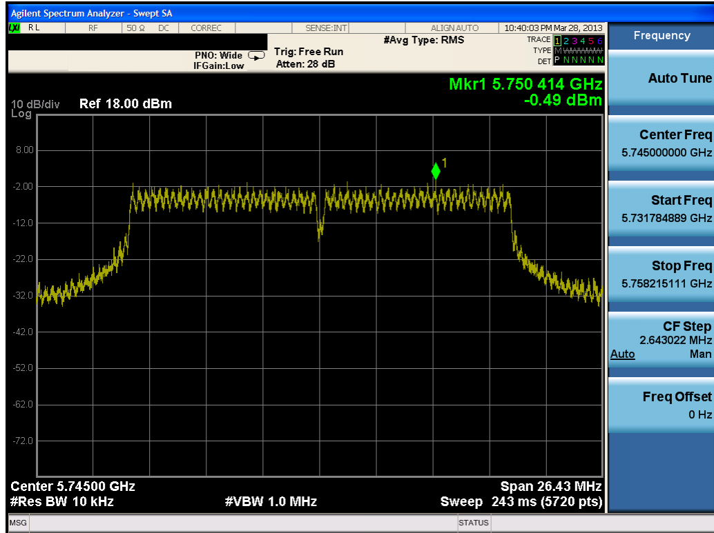
Plot 6-33. Power Spectral Density Plot (20MHz BW 802.11n (5.8GHz) – Ch. 149)
