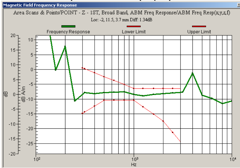
Graph 5: WCDMA 1700 Frequency Response
