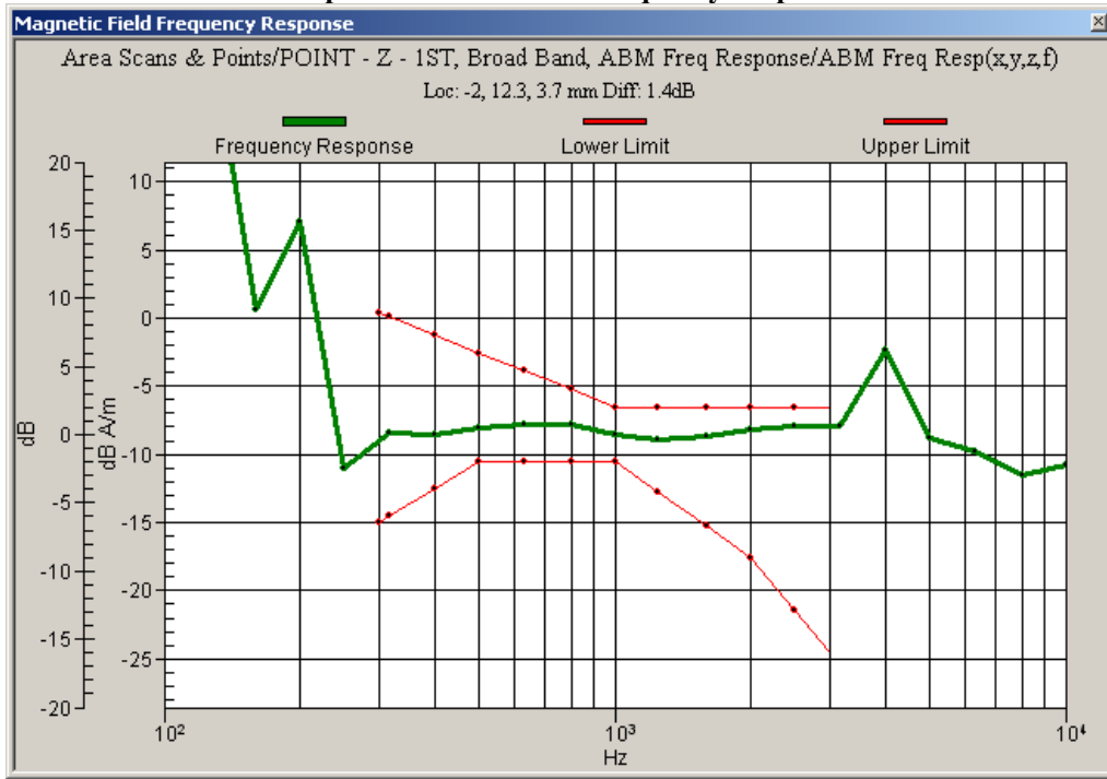
Graph 6: WCDMA 1900 Frequency Response
