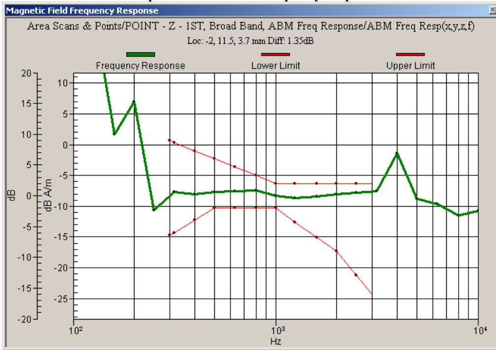
Graph 4: WCDMA 850 Frequency Response
